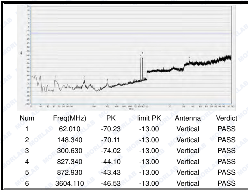
(Plot E2: WCDMA 850MHz Channel = 4132, Test Antenna Vertical)
