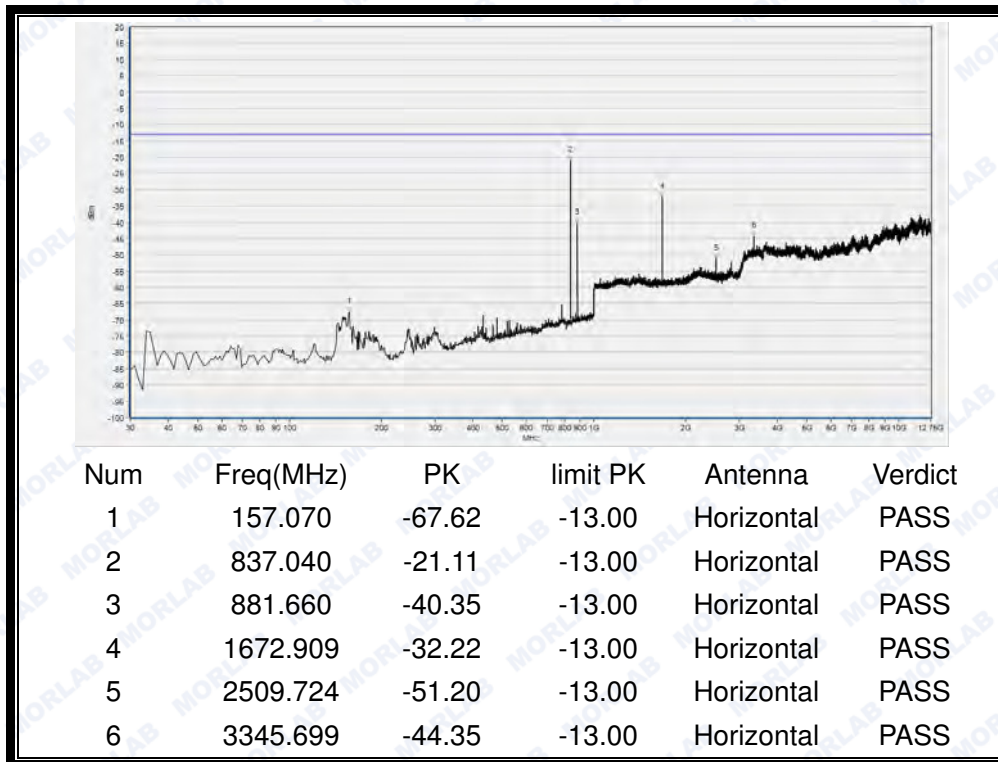
(Plot A3: GSM850MHz Channel = 190, Test Antenna Horizontal)
