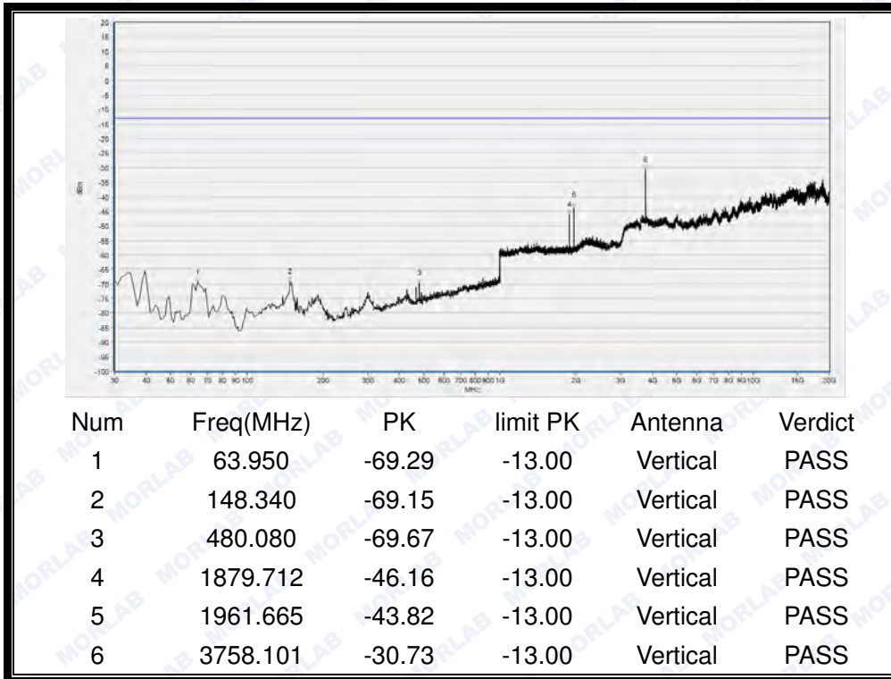
(Plot J4: HSUPA 1900MHz Channel = 9400, Test Antenna Vertical)
