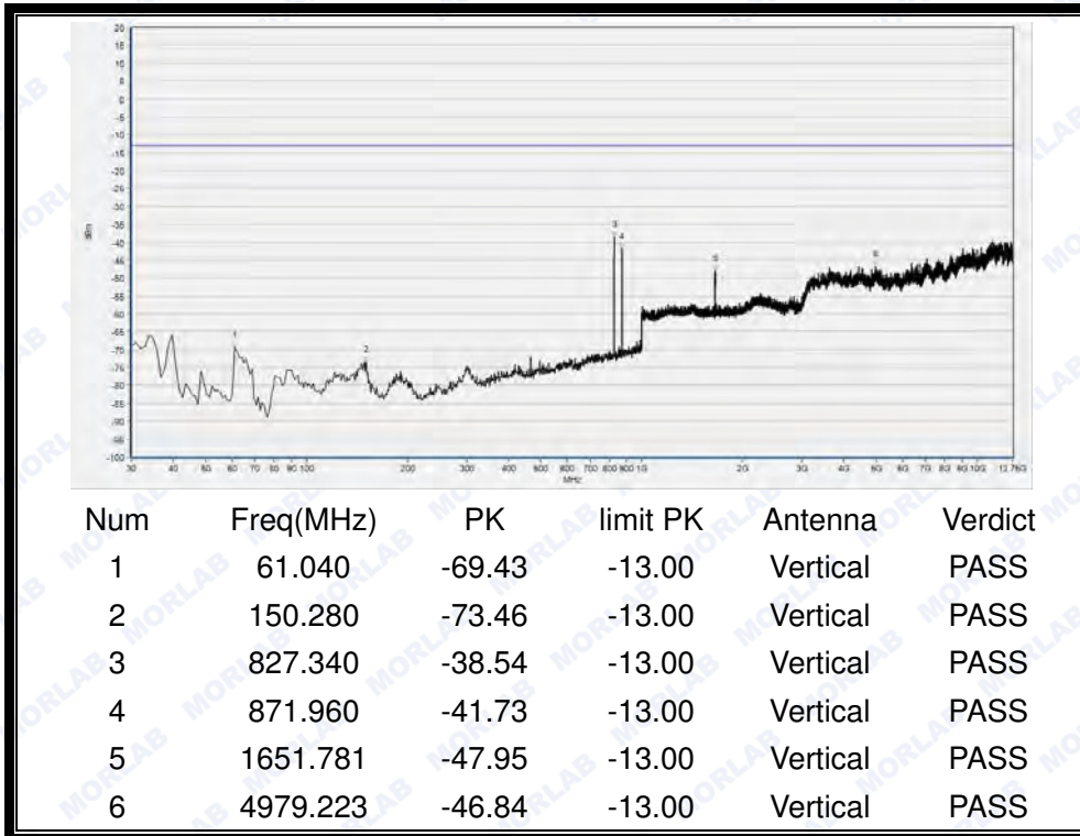
(Plot K2: HSPA+ 850MHz Channel = 4132, Test Antenna Vertical)
