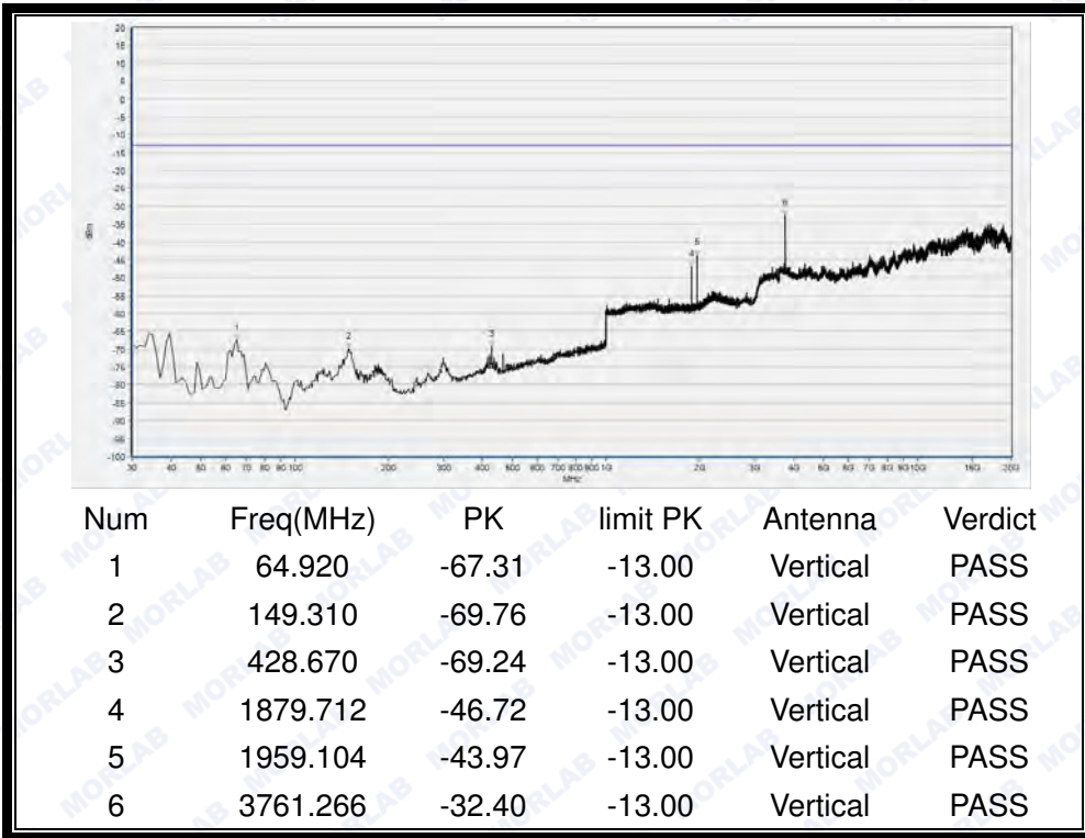
(Plot H4: HSDPA 1900MHz Channel = 9400, Test Antenna Vertical)
