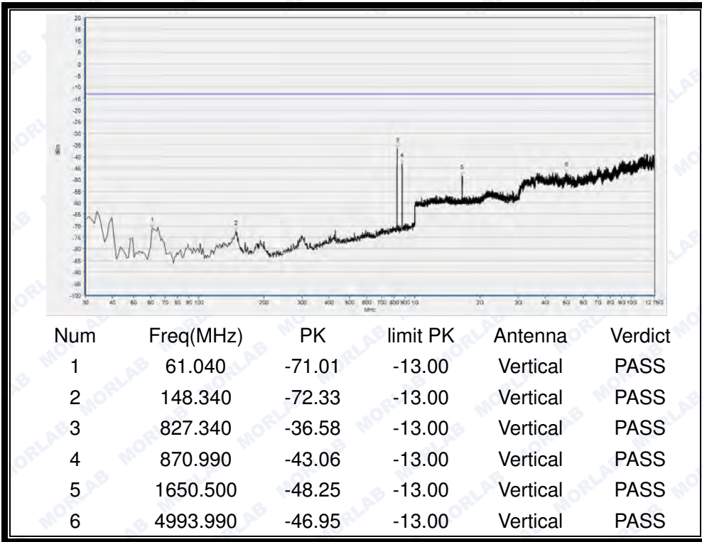
(Plot G2: HSDPA 850MHz Channel = 4132, Test Antenna Vertical)
