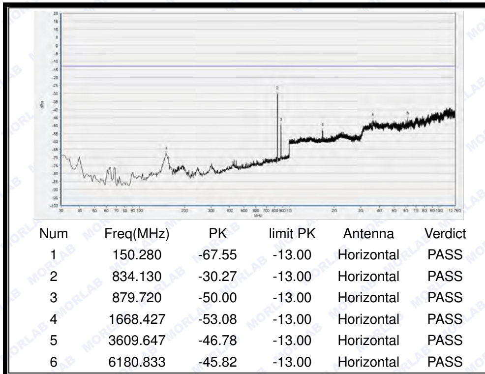
(Plot I3: HSUPA 850MHz Channel = 4175, Test Antenna Horizontal)
