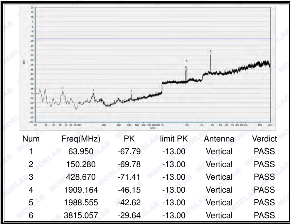
(Plot F6: WCDMA 1900MHz Channel = 9538, Test Antenna Vertical)
