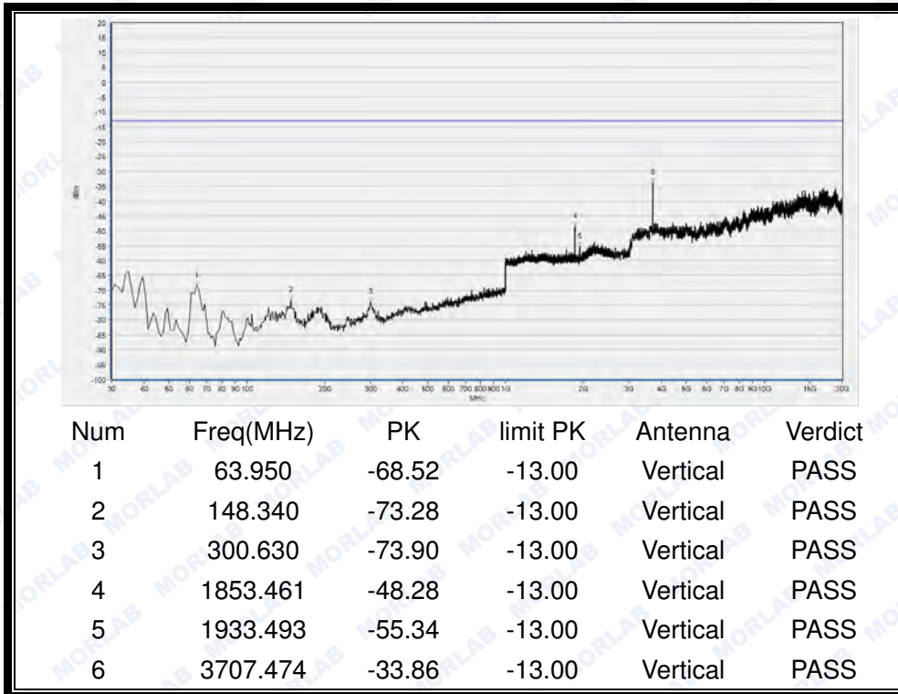
(Plot L2: HSPA+ 1900MHz Channel = 9262, Test Antenna Vertical)
