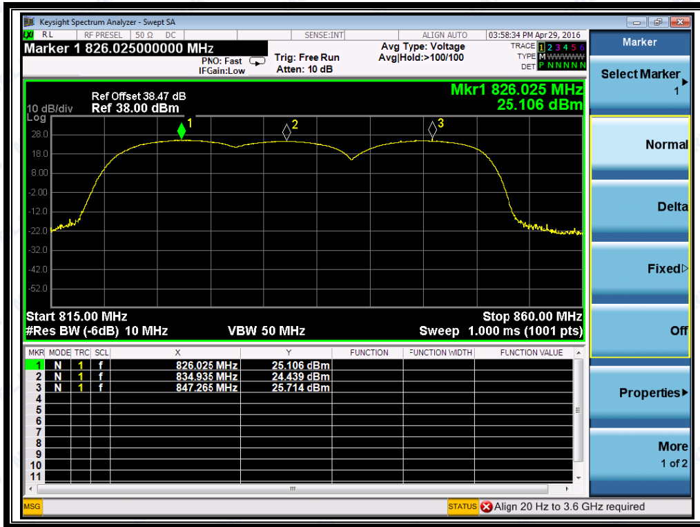
(Plot I: HSPA+ 850 MHz Channel = 4132, 4175, 4233)
