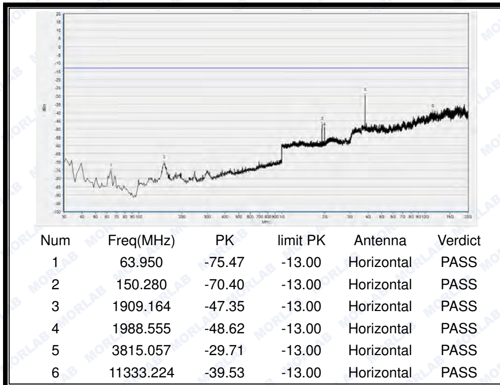
(Plot J5: HSUPA 1900MHz Channel = 9538, Test Antenna Horizontal)
