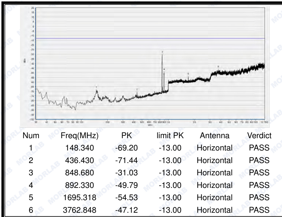
(Plot E5: WCDMA 850MHz Channel = 4233, Test Antenna Horizontal)
