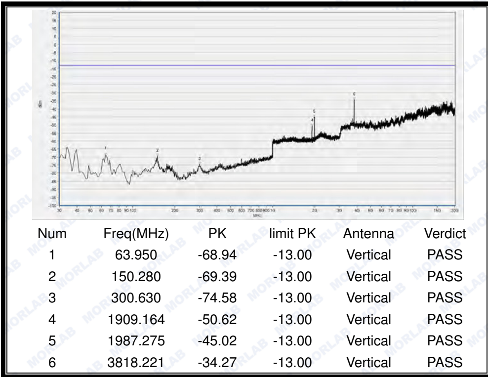
(Plot H6: HSDPA 1900MHz Channel = 9538, Test Antenna Vertical)
