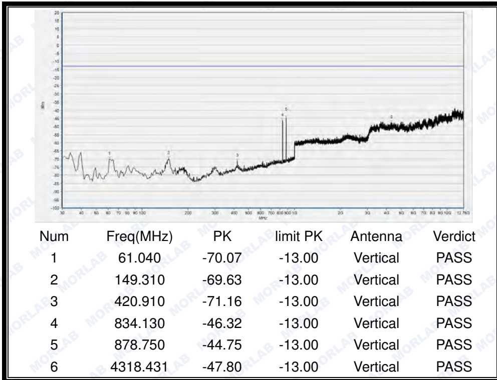
(Plot K4: HSPA+ 850MHz Channel = 4175, Test Antenna Vertical)
