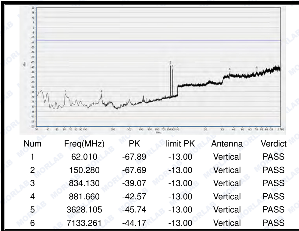
(Plot E4: WCDMA 850MHz Channel = 4175, Test Antenna Vertical)
