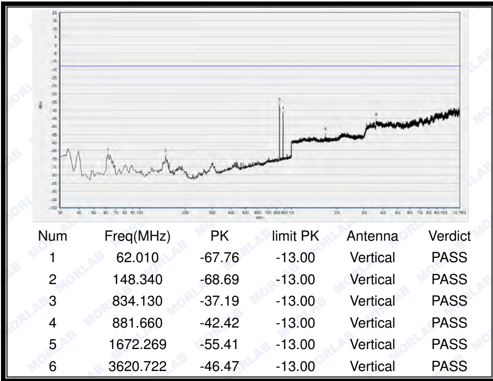
(Plot G4: HSDPA 850MHz Channel = 4175, Test Antenna Vertical)
