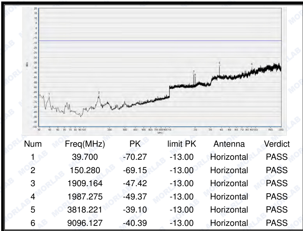
(Plot F5: WCDMA 1900MHz Channel = 9538, Test Antenna Horizontal)
