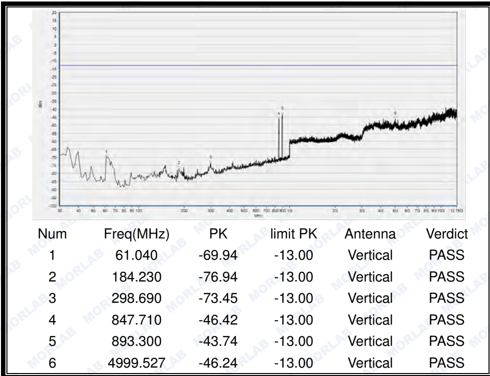
(Plot E6: WCDMA 850MHz Channel = 4233, Test Antenna Vertical)
