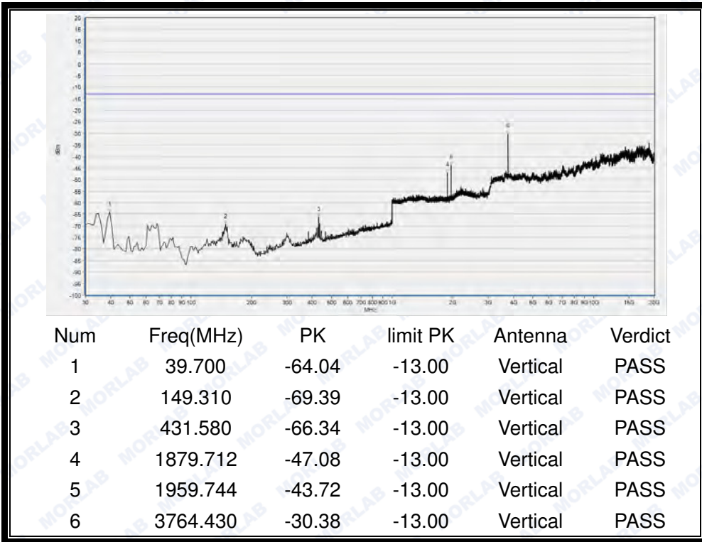
(Plot F4: WCDMA 1900MHz Channel = 9400, Test Antenna Vertical)
