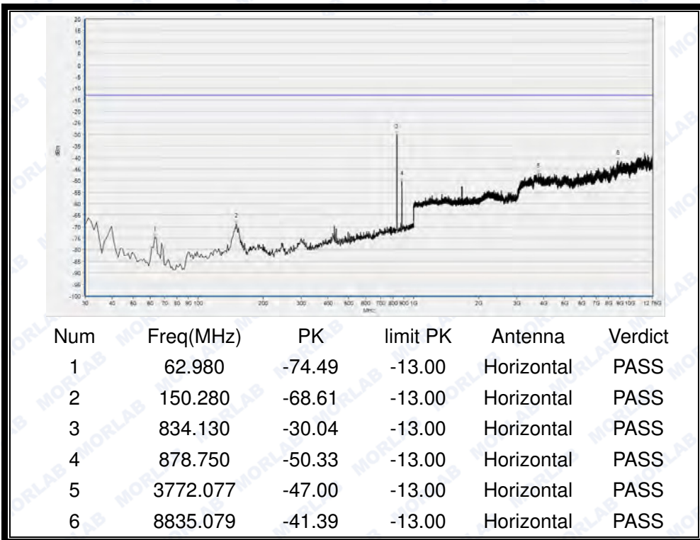
(Plot G3: HSDPA 850MHz Channel = 4175, Test Antenna Horizontal)
