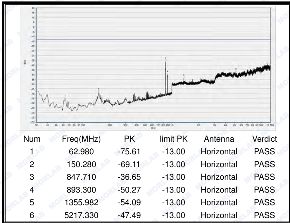
(Plot K5: HSPA+ 850MHz Channel = 4233, Test Antenna Horizontal)
