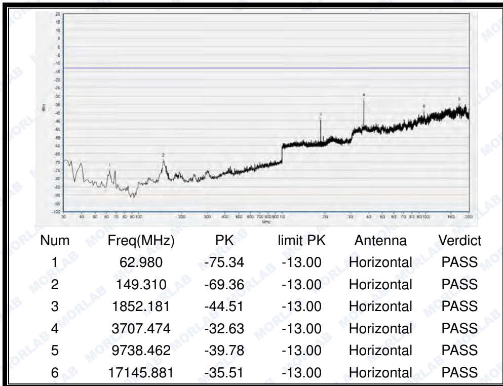
(Plot F1: WCDMA 1900MHz Channel = 9262, Test Antenna Horizontal)
