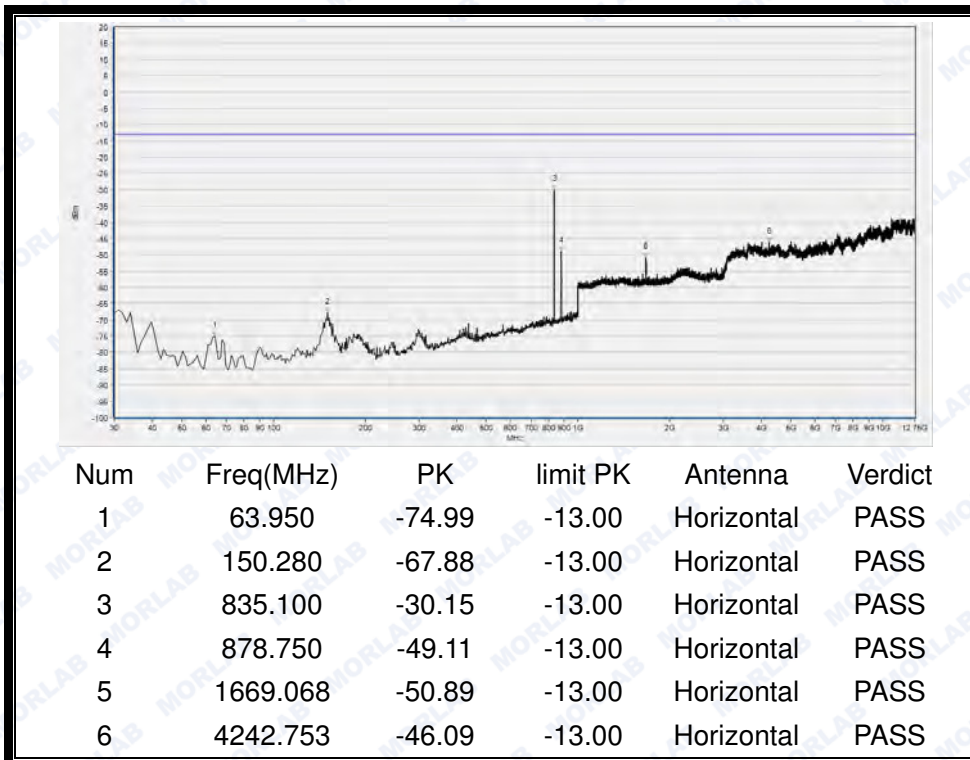
(Plot E3: WCDMA 850MHz Channel = 4175, Test Antenna Horizontal)
