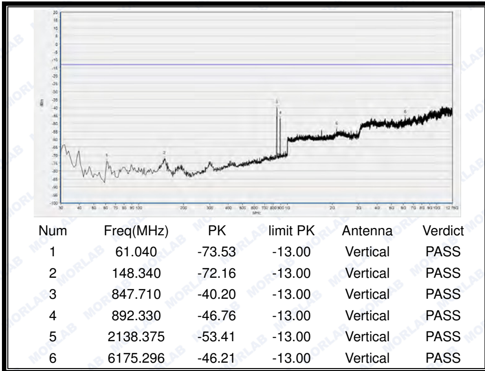
(Plot K6: HSPA+ 850MHz Channel = 4233, Test Antenna Vertical)
