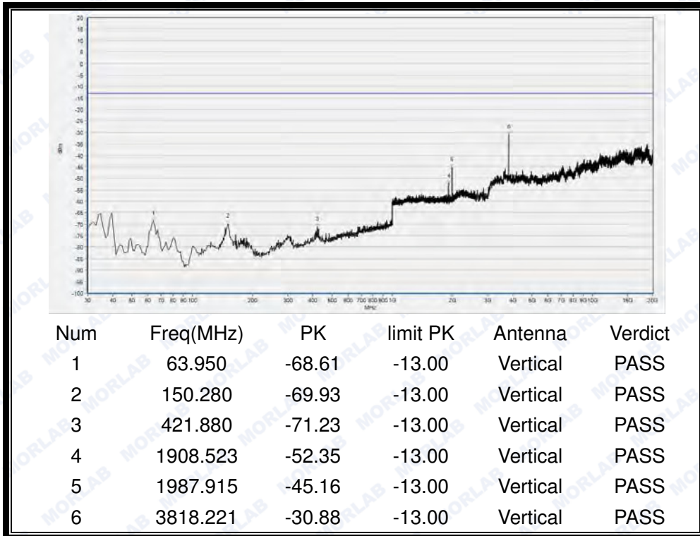
(Plot J6: HSUPA 1900MHz Channel = 9538, Test Antenna Vertical)
