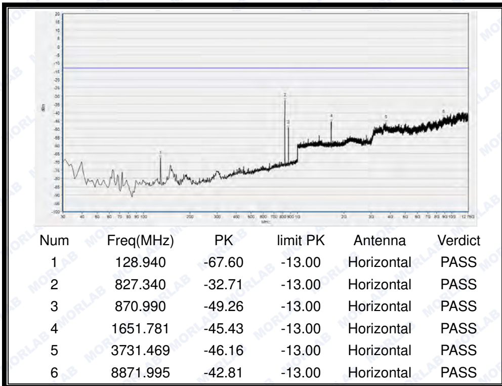
(Plot K1: HSPA+ 850MHz Channel = 4132, Test Antenna Horizontal)
