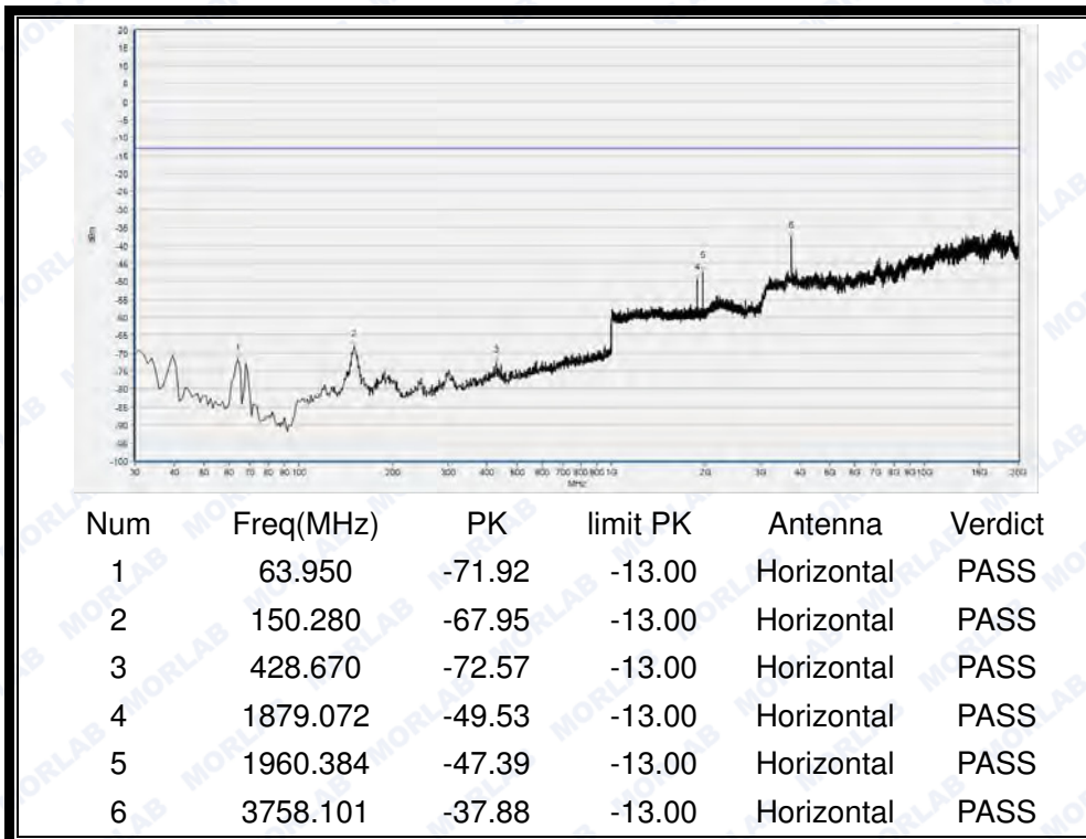
(Plot L3: HSPA+ 1900MHz Channel = 9400, Test Antenna Horizontal)
