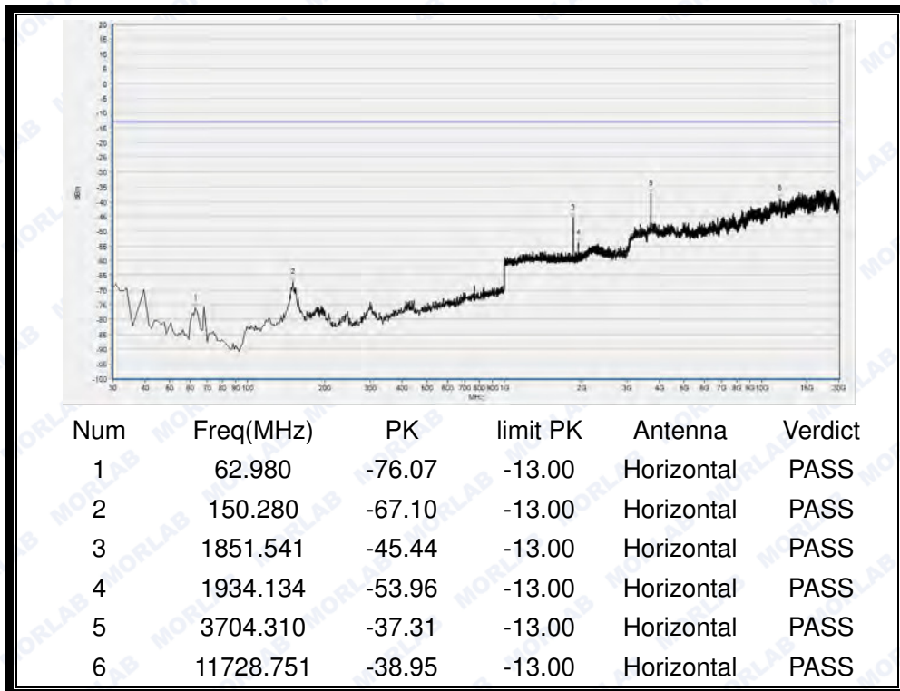
(Plot L1: HSPA+ 1900MHz Channel = 9262, Test Antenna Horizontal)
