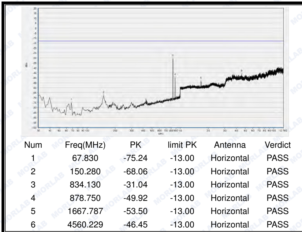
(Plot K3: HSPA+ 850MHz Channel = 4175, Test Antenna Horizontal)
