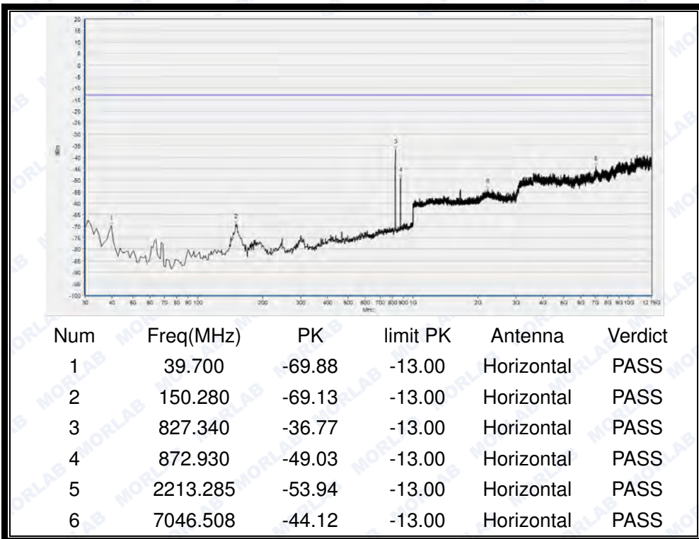
(Plot G1: HSDPA 850MHz Channel = 4132, Test Antenna Horizontal)
