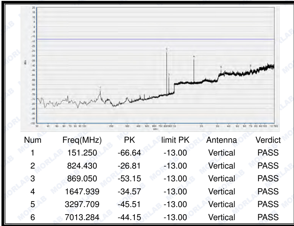
(Plot A2: GSM 850MHz Channel = 128, Test Antenna Vertical)
