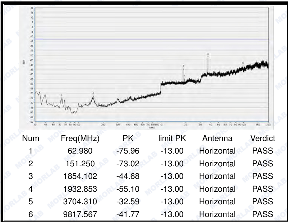
(Plot J1: HSUPA 1900MHz Channel = 9262, Test Antenna Horizontal)
