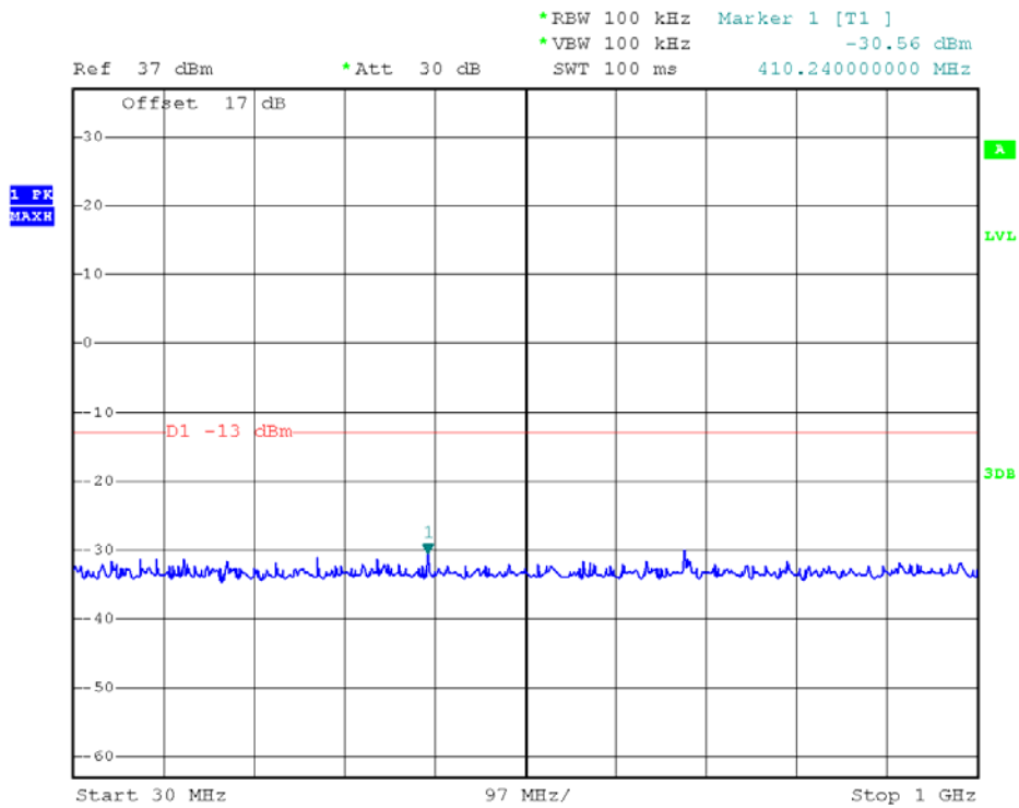
WCDMA1700MHz Channel = 1513, 30MHz to 1GHz
