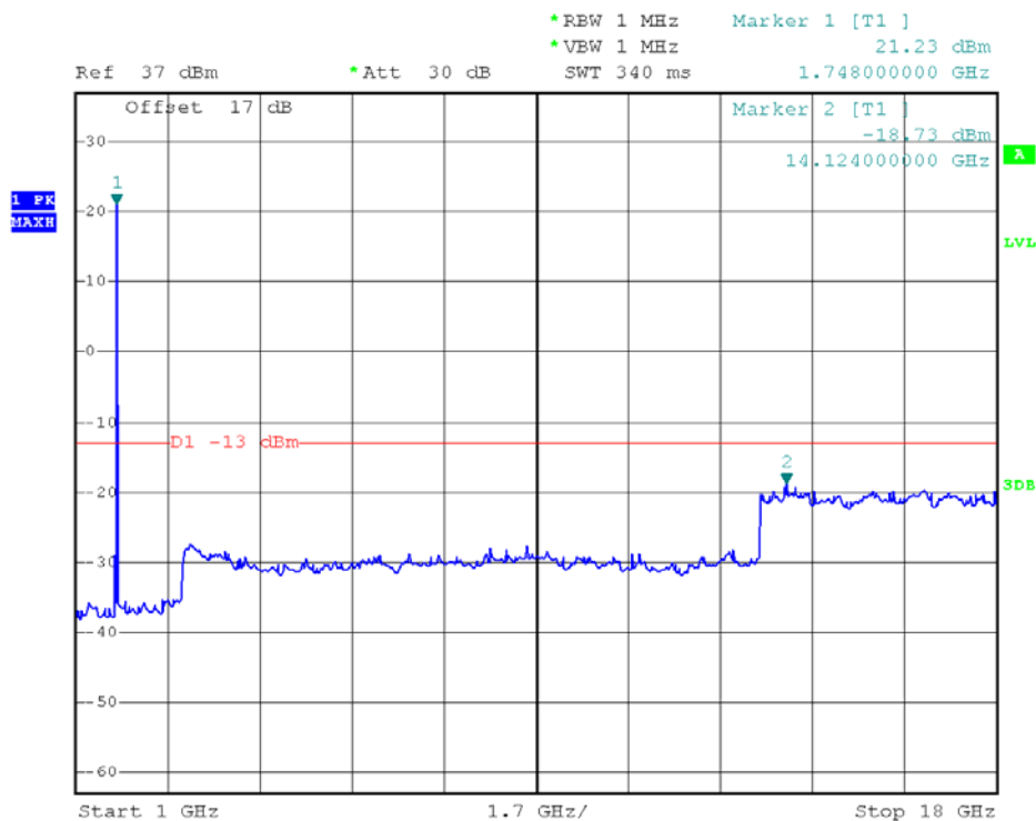
WCDMA1700MHz Channel = 1513 1GHz to 18GHz
