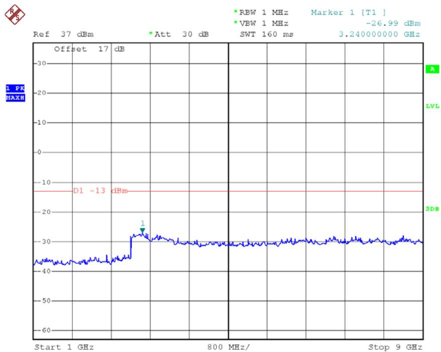
GSM 850MHz Channel = 128, 1GHz to 9GHz
