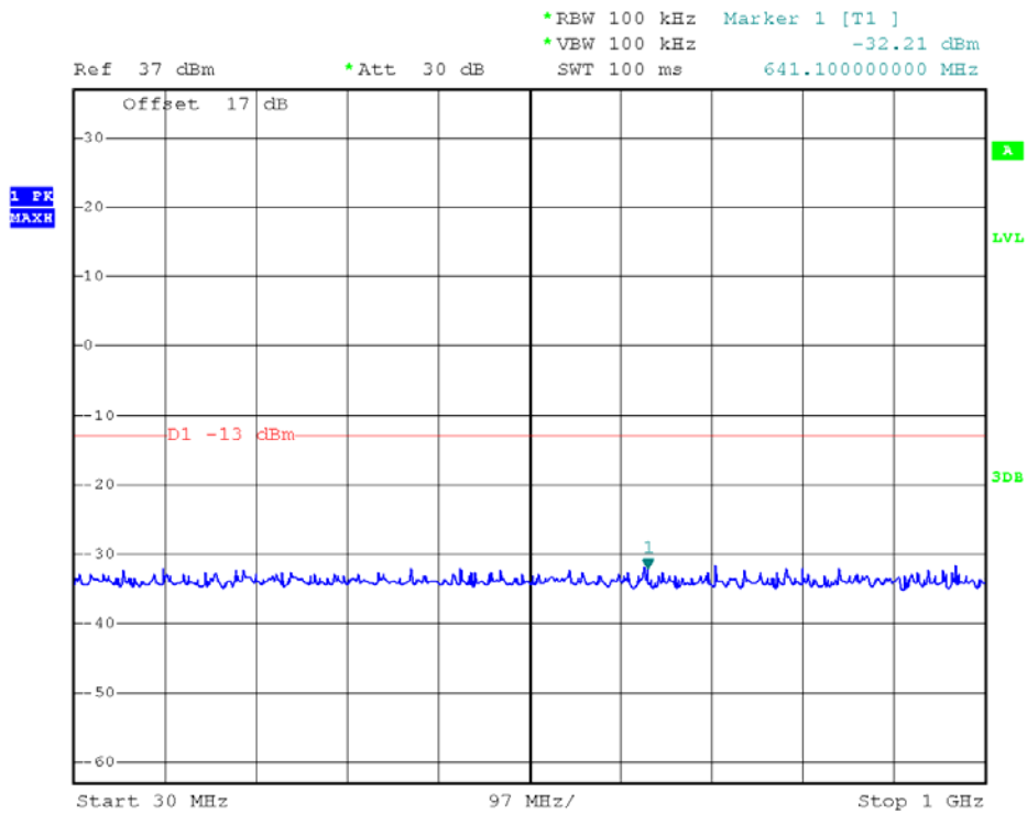
WCDMA1700MHz Channel = 1412, 30MHz to 1GHz
