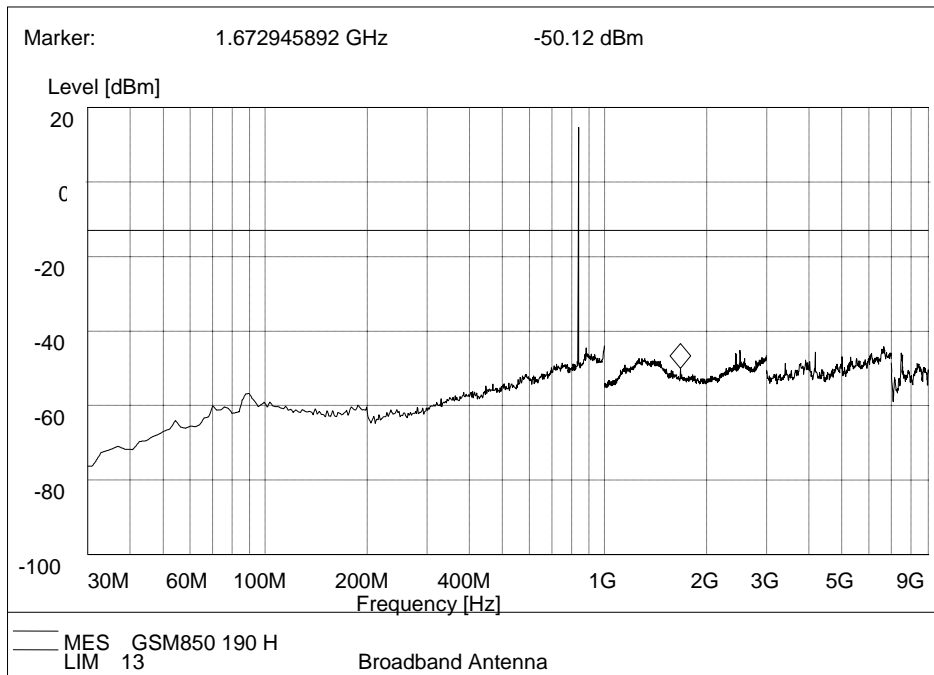
GSM 850MHz, Test Antenna Horizontal
