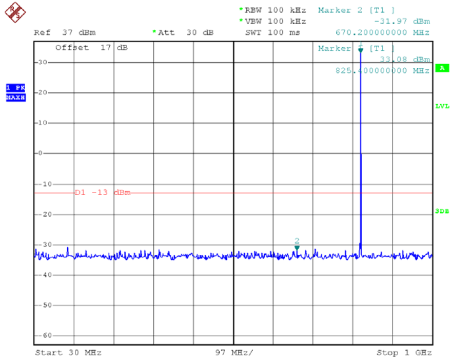
GSM 850MHz Channel = 128, 30MHz to 1GHz
