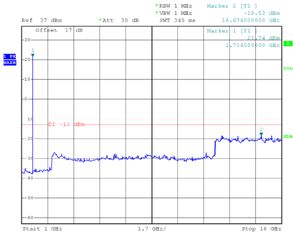
WCDMA1700MHz Channel = 1412, 1GHz to 18GHz
