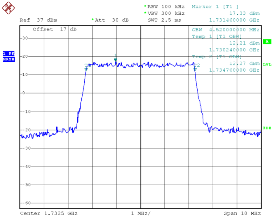
(Plot I1: 99% Occupied Bandwidth LTE Band 4/5MHz/QPSK)
