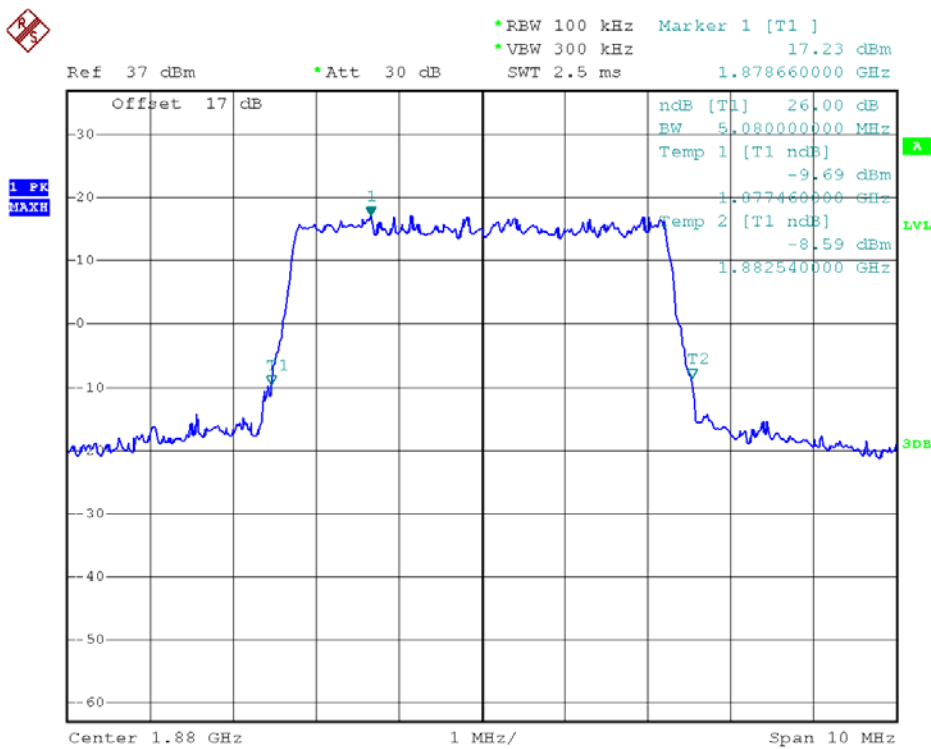
(Plot C2: 26dB Bandwidth LTE Band 2/5MHz/QPSK)
