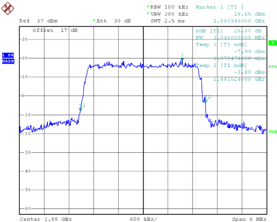
(Plot B4: 26dB Bandwidth LTE Band 2/3MHz/16QAM)
