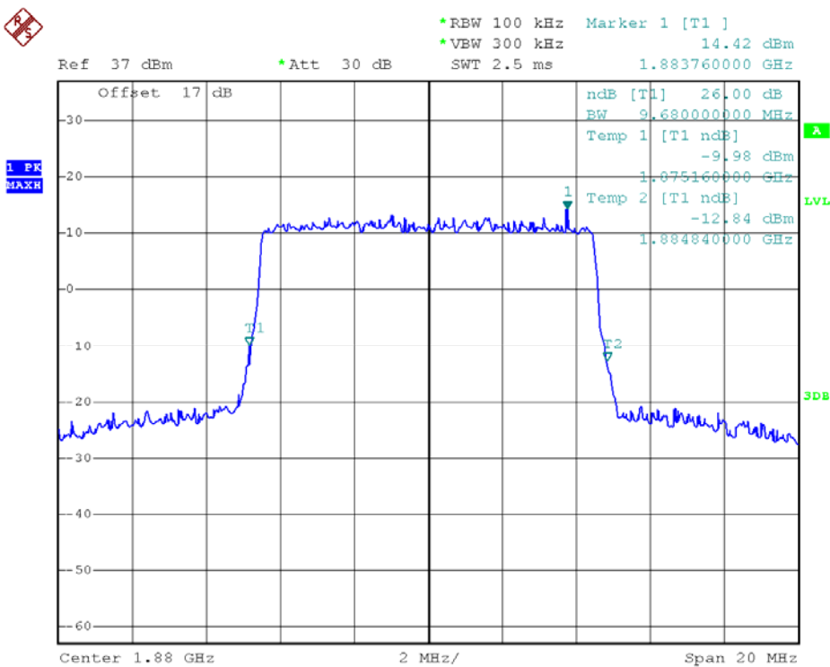
(Plot D3: 99% Occupied Bandwidth LTE Band 2/10MHz/16QAM)
