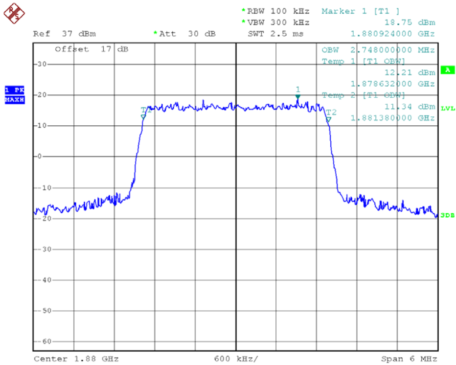
(Plot B3: 99% Occupied Bandwidth LTE Band 2/3MHz/16QAM)
