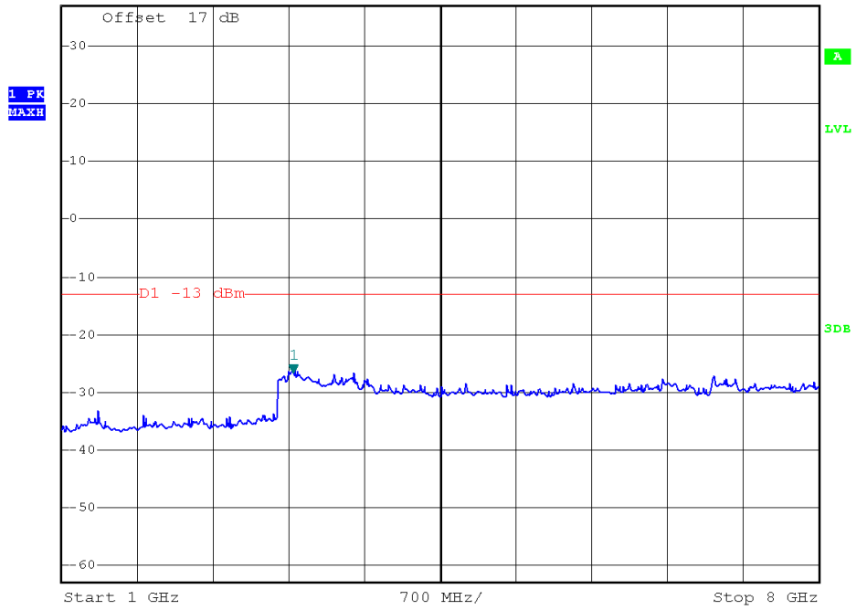
RB Size 1, RB Offset 0 1GHz to 8GHz
