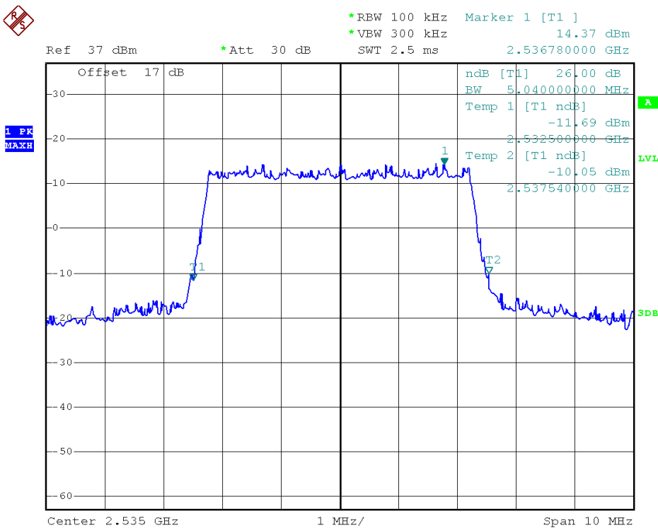
(Plot M4: 26dB Bandwidth LTE Band 7/5MHz/16QAM)
