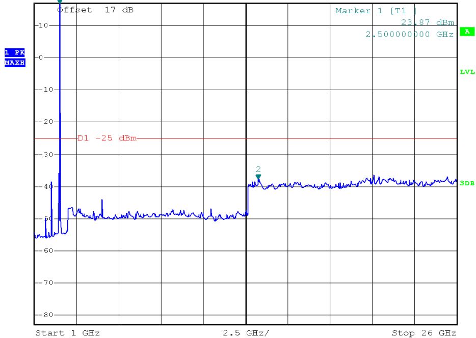
RB Size 1, RB Offset 0 1GHz to 26GHz
