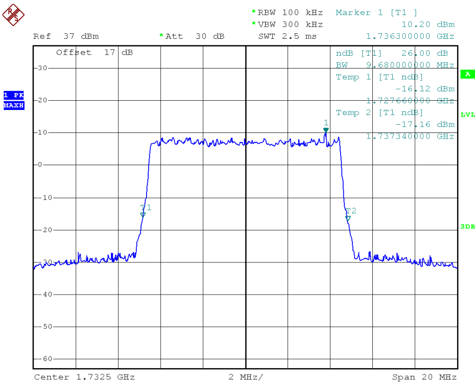
(Plot J4: 26dB Bandwidth LTE Band 4/10MHz/16QAM)
