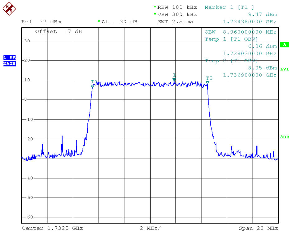
(Plot J1: 99% Occupied Bandwidth LTE Band 4/10MHz/QPSK)
