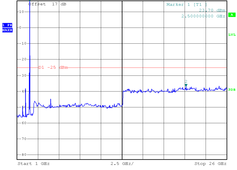
RB Size 1, RB Offset 0 1GHz to 26GHz
