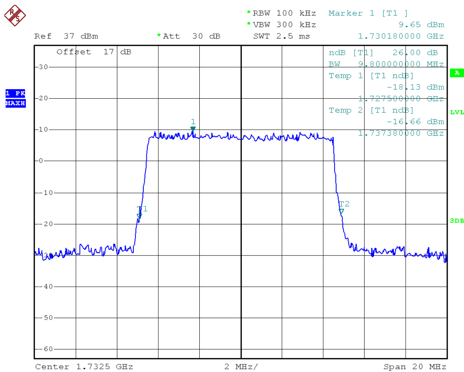
(Plot J2: 26dB Bandwidth LTE Band 4/10MHz/QPSK)
