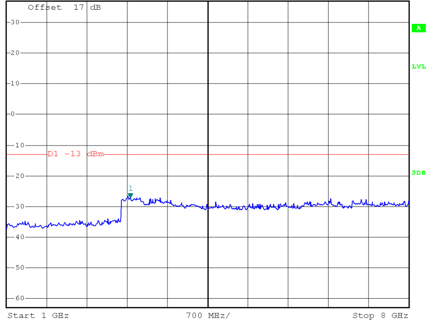
RB Size 1, RB Offset 0 1GHz to 8GHz
