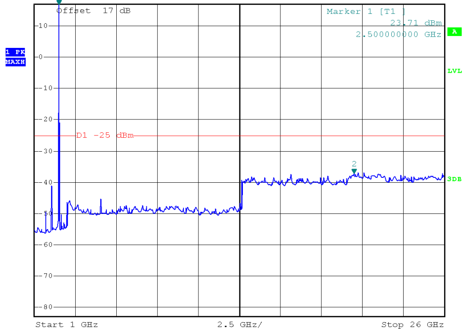
RB Size 1, RB Offset 0 1GHz to 26GHz
