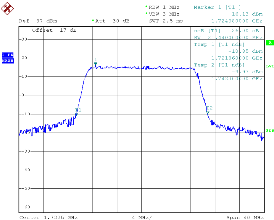
(Plot L4: 26dB Bandwidth LTE Band 4/20MHz/16QAM)
