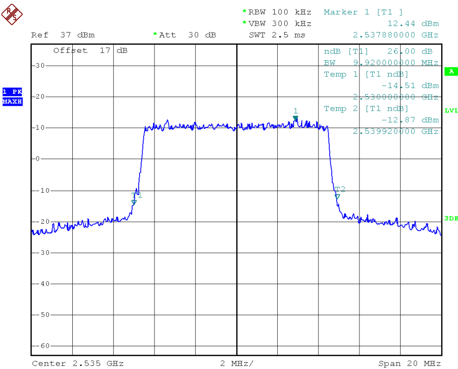
(Plot N2: 26dB Bandwidth LTE Band 7/10MHz/QPSK)
