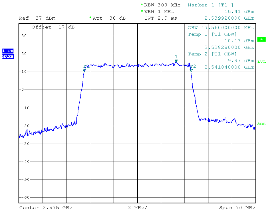
(Plot O3: 99% Occupied Bandwidth LTE Band 7/15MHz/16QAM)
