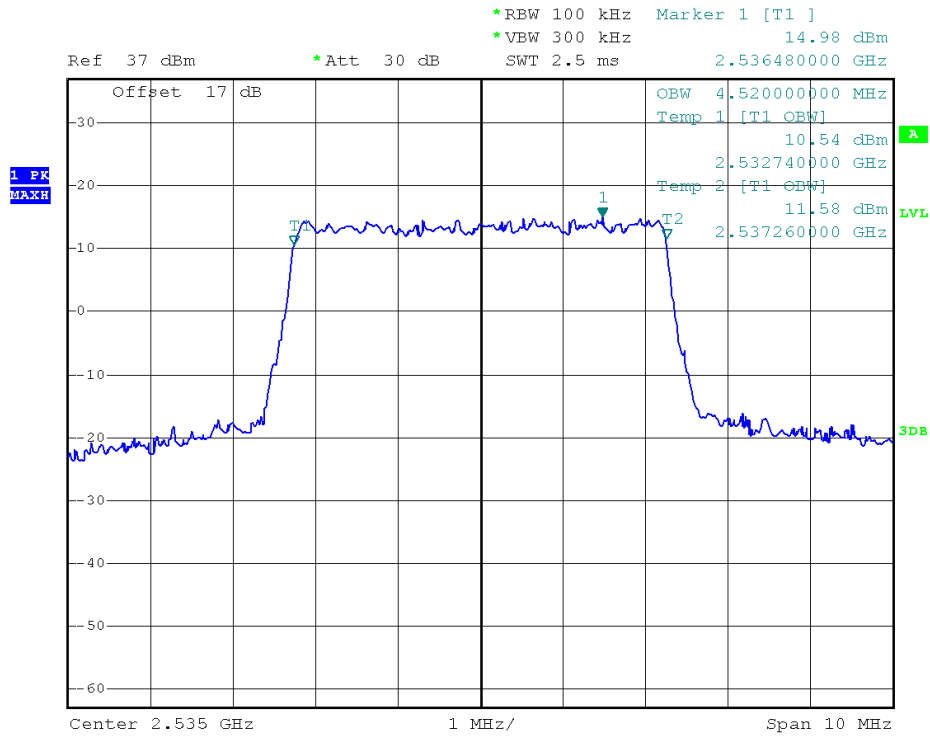
(Plot M1: 99% Occupied Bandwidth LTE Band 7/5MHz/QPSK)
