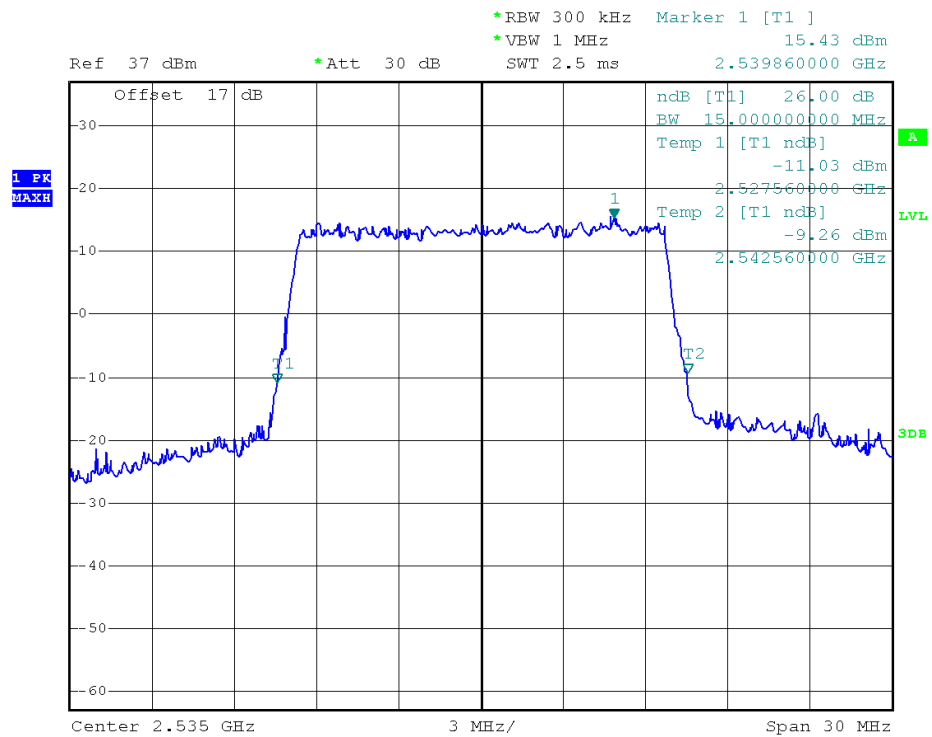
(Plot O4: 26dB Bandwidth LTE Band 7/15MHz/16QAM)
