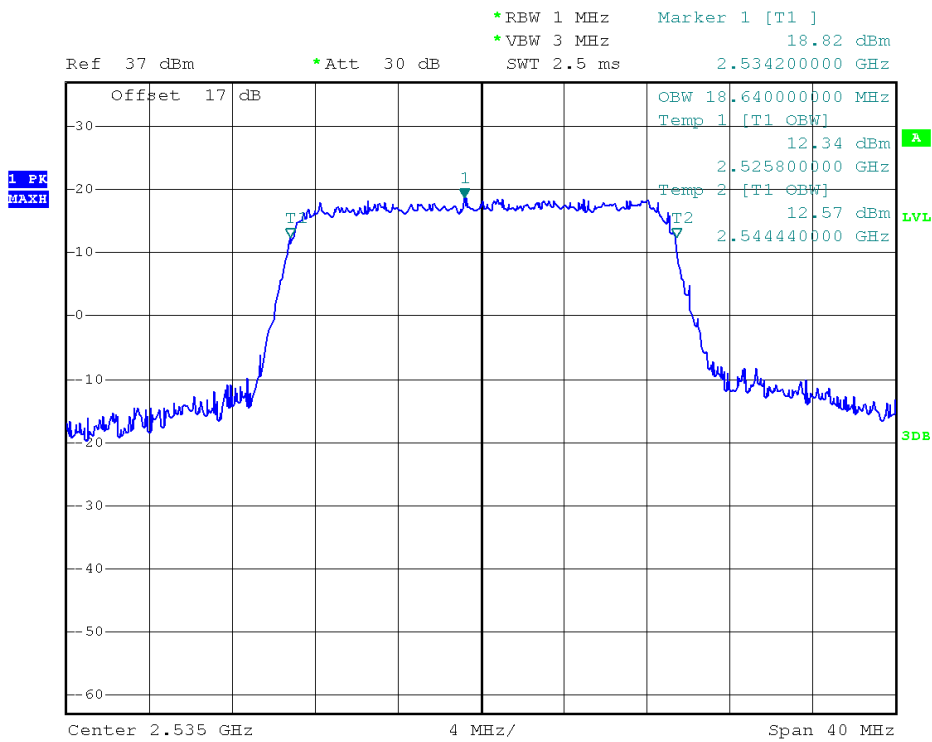
(Plot P3: 99% Occupied Bandwidth LTE Band 7/20MHz/16QAM)
