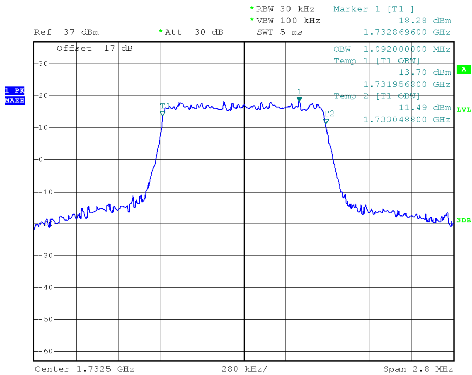
(Plot G1: 99% Occupied Bandwidth LTE Band 4/1.4MHz/QPSK)
