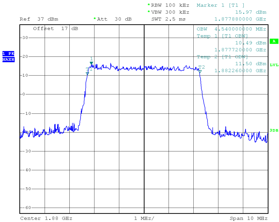
(Plot C3: 99% Occupied Bandwidth LTE Band 2/5MHz/16QAM)
