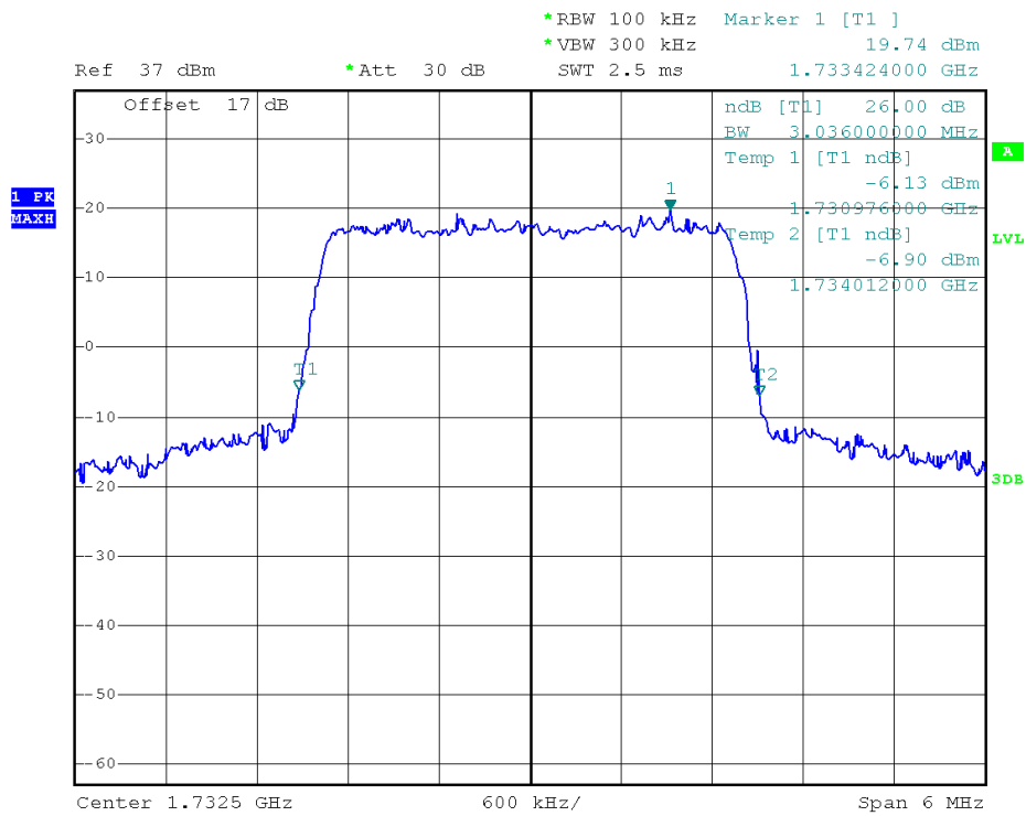
(Plot H4: 26dB Bandwidth LTE Band 4/3MHz/16QAM)
