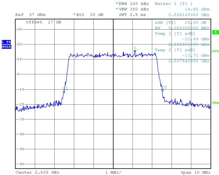
(Plot M2: 26dB Bandwidth LTE Band 7/5MHz/QPSK)
