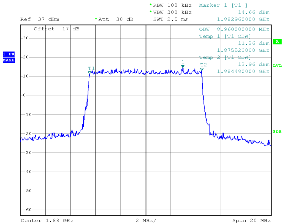
(Plot D1: 99% Occupied Bandwidth LTE Band 2/10MHz/QPSK)
