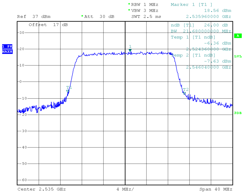
(Plot P4: 26dB Bandwidth LTE Band 7/20MHz/16QAM)
