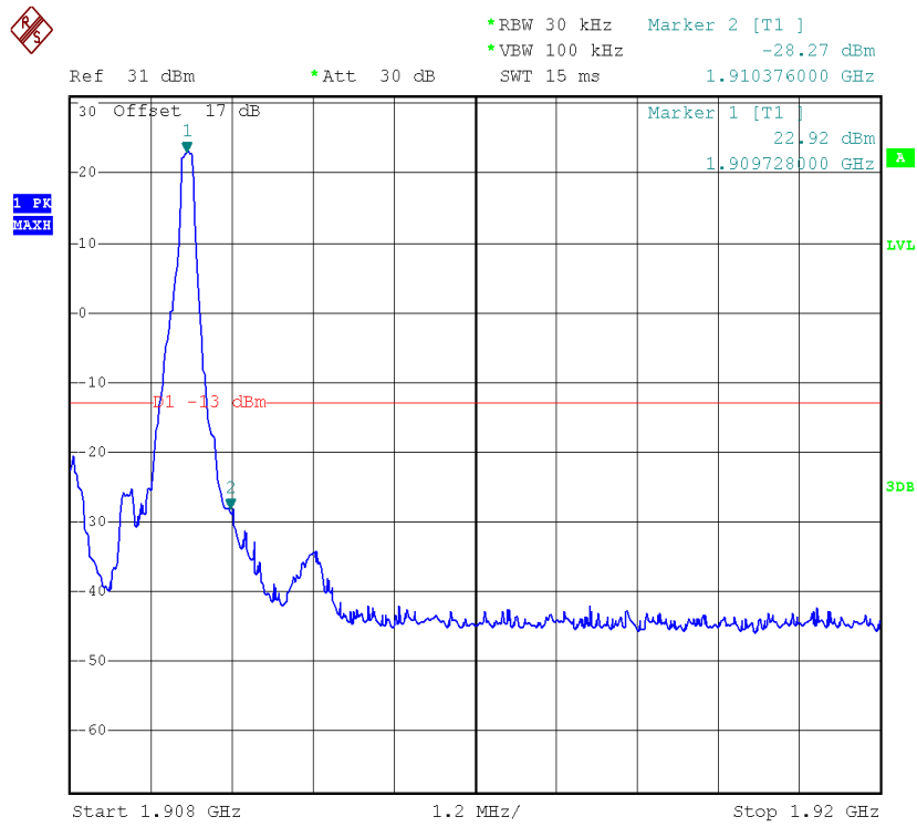
Higher Band Edge Plot for QPSK-RB Size 1, RB Offset 5
