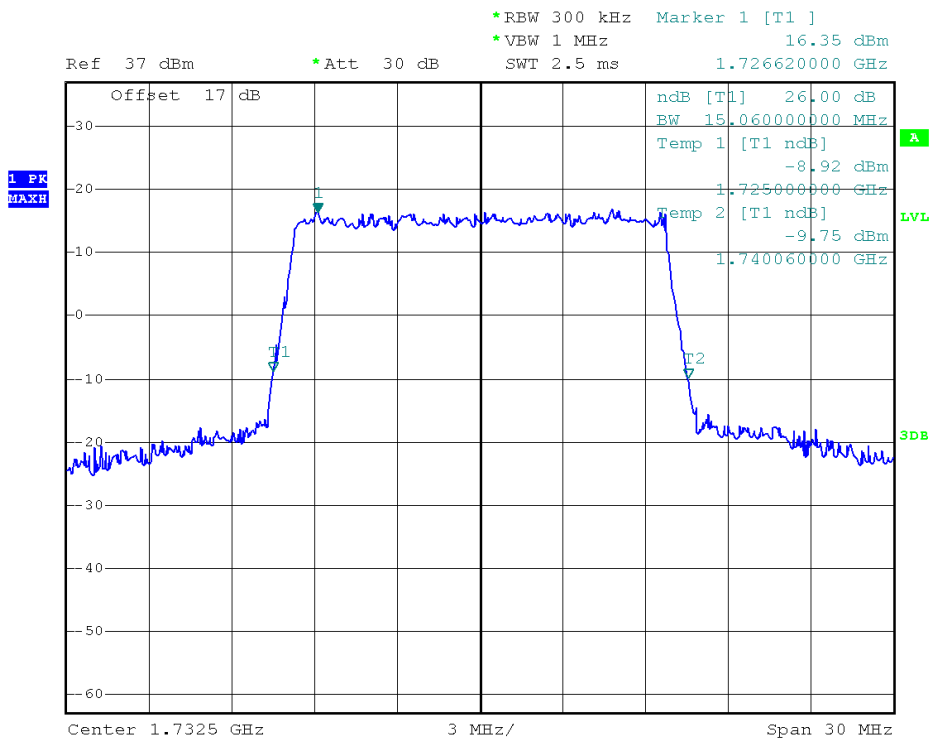
(Plot K4: 26dB Bandwidth LTE Band 4/15MHz/16QAM)
