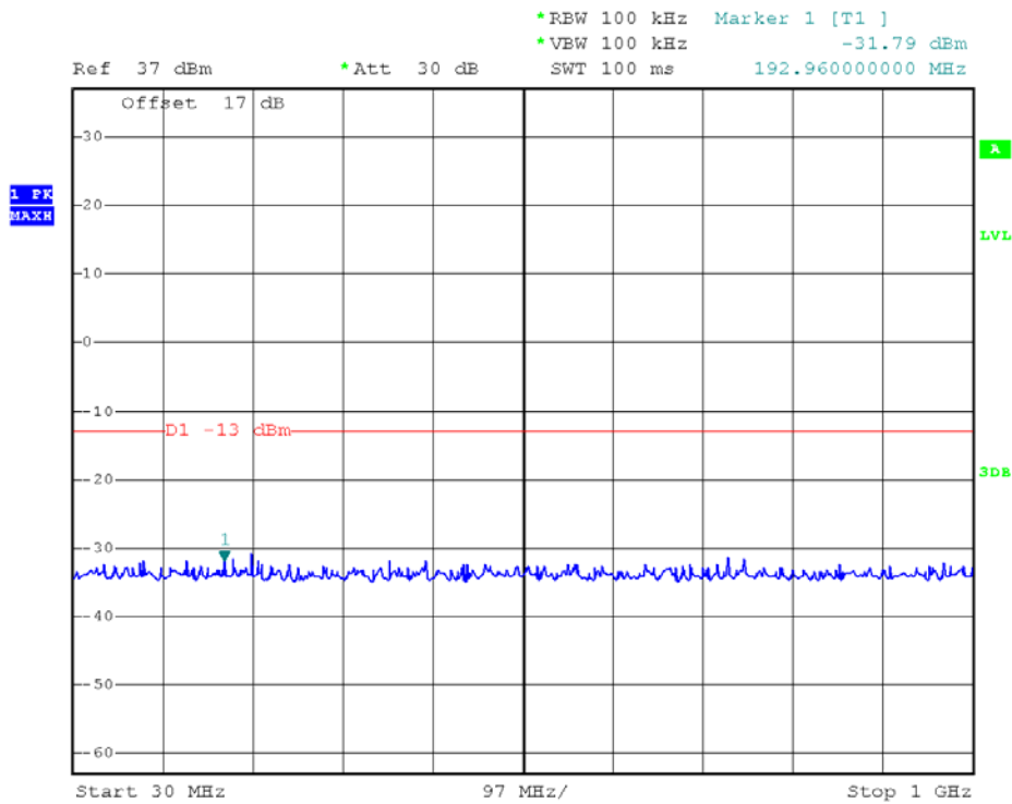
GSM 1900MHz Channel = 810, 30MHz to 1GHz
