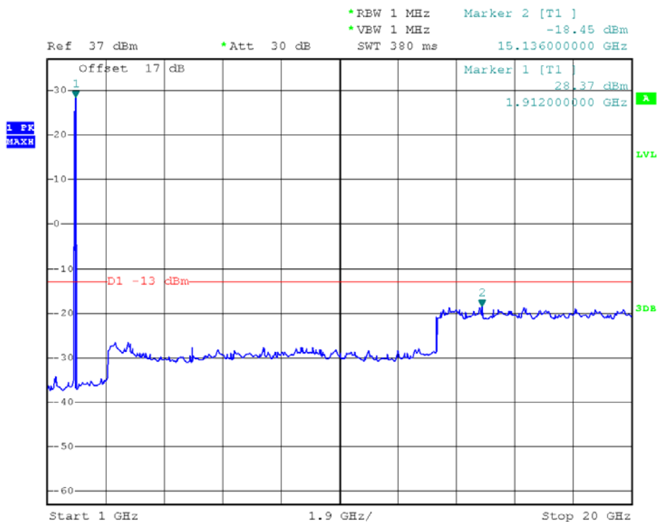
GSM 1900MHz Channel = 810, 1GHz to 20GHz
