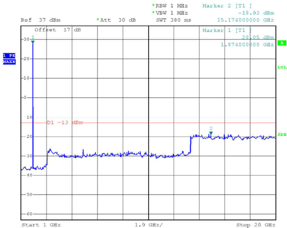
GSM 1900MHz Channel = 661, 1GHz to 20GHz
