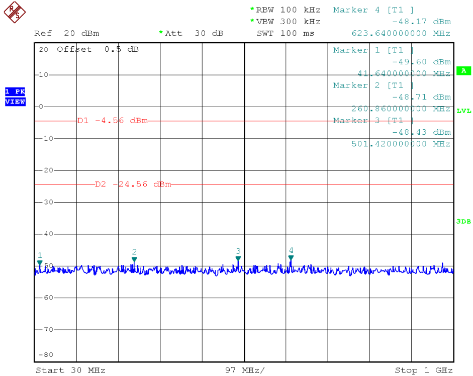
Channel = 3, 30MHz to 1GHz
