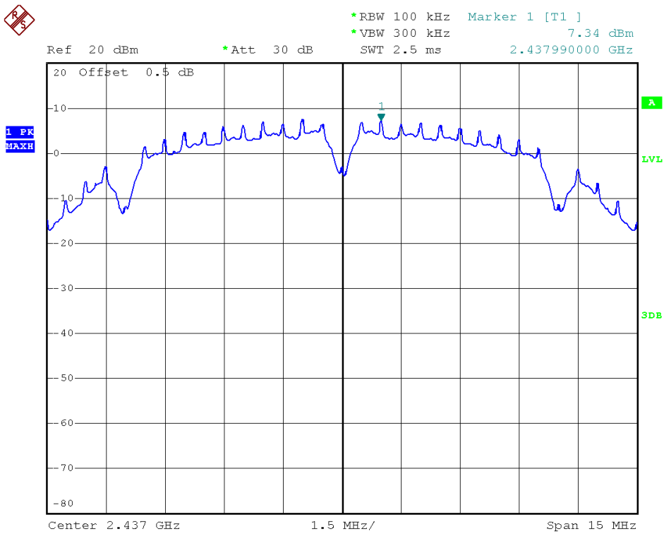
802.11b - PSD Plot on Channel 6
