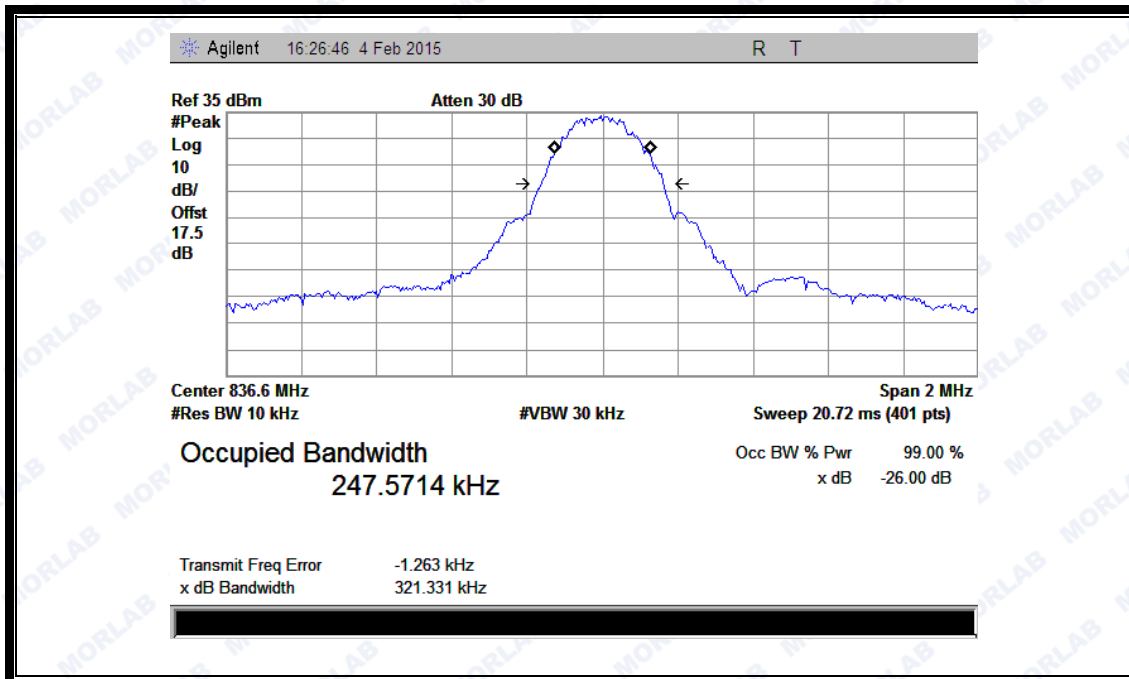
(Plot H: GPRS 850MHz Channel = 190)
