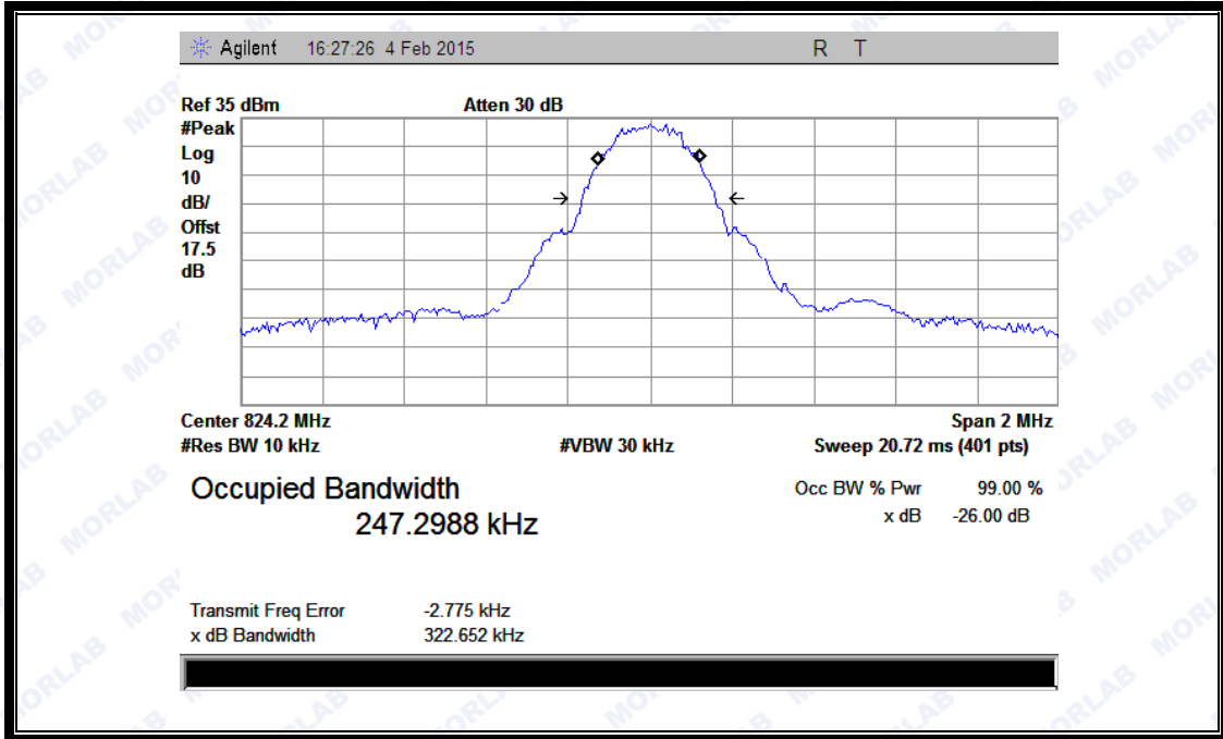
(Plot G: GPRS 850MHz Channel = 128)
