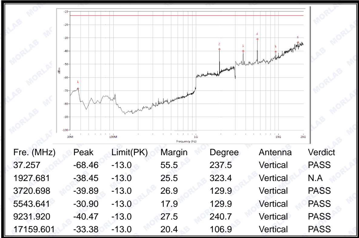
(Plot B.2: GSM 1900MHz Channel = 512, Test Antenna Vertical)
