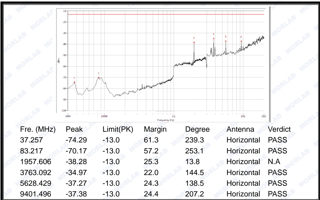
(Plot B.3: GSM 1900MHz Channel = 661, Test Antenna Horizontal)
