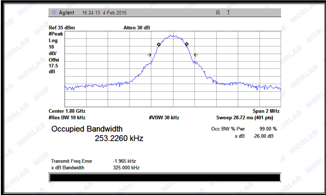
(Plot K: GPRS 1900MHz Channel = 661)
