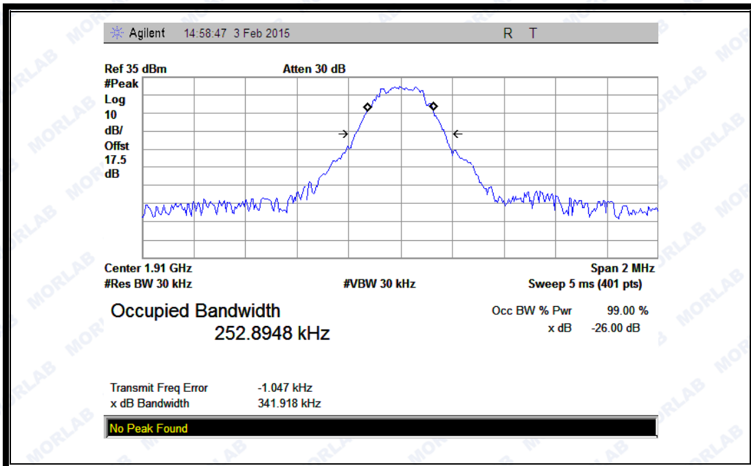
(Plot F: GSM 1900MHz Channel = 810)
