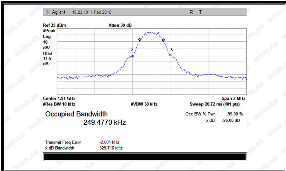
(Plot L: GPRS 1900MHz Channel = 810)
