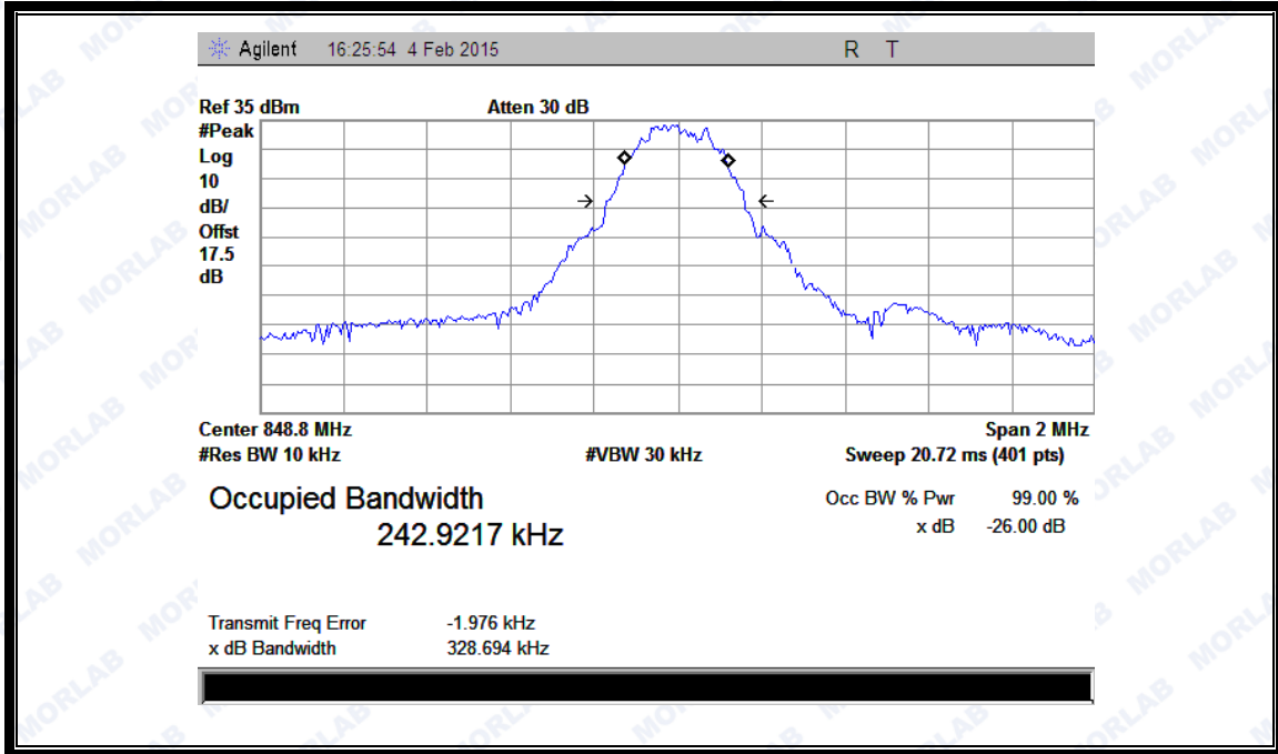
(Plot I: GPRS850MHz Channel = 251)
