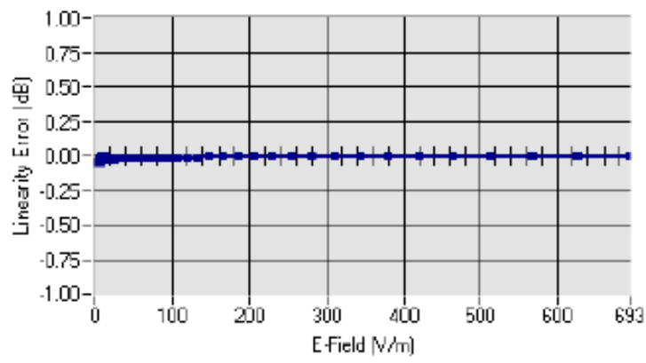
Linearity
