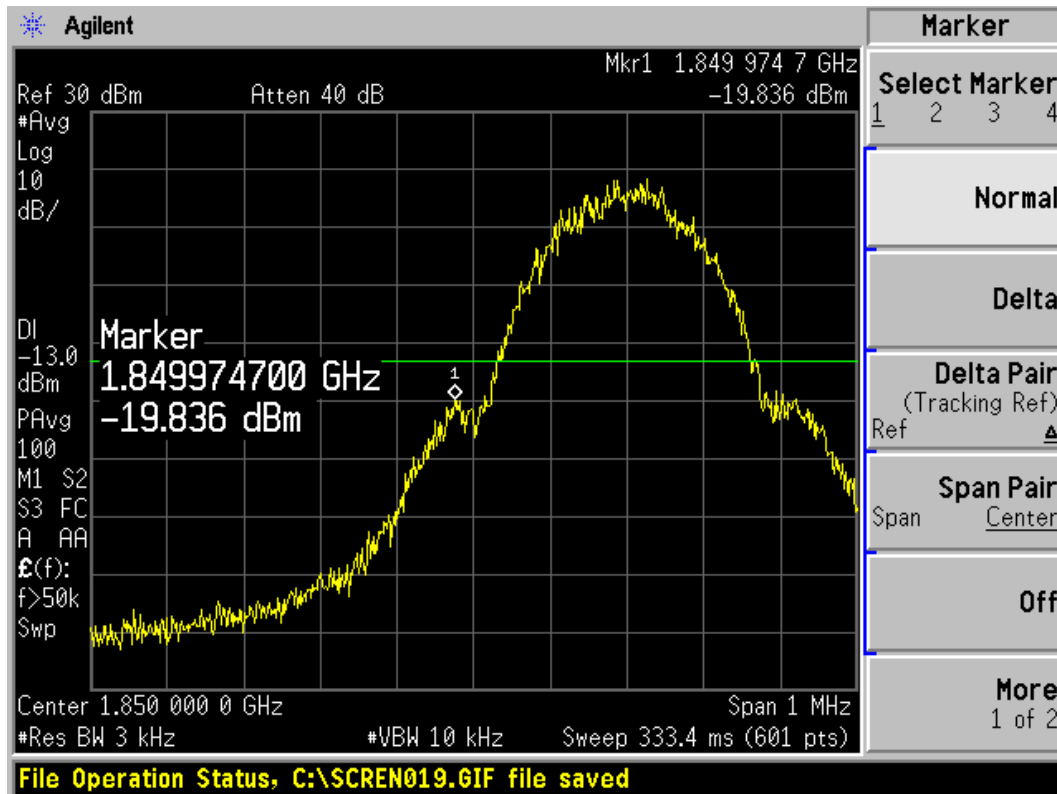
GSM 1900 512 Channel
