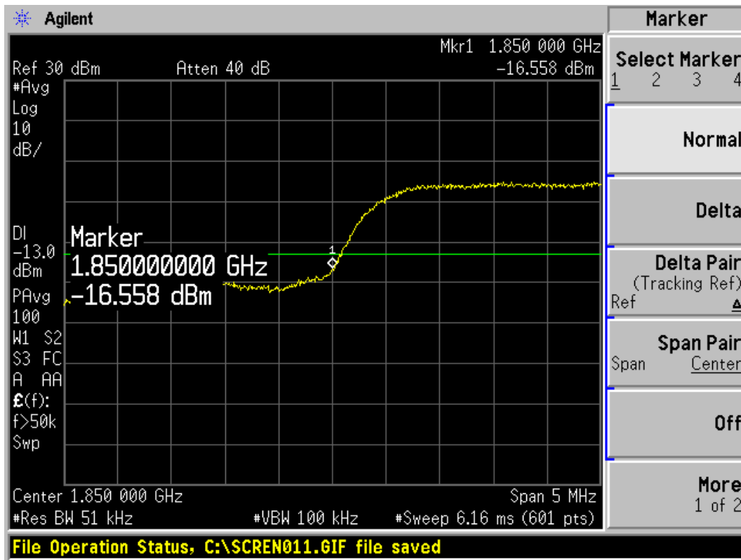
WCDMA Band II 9262 Channel
