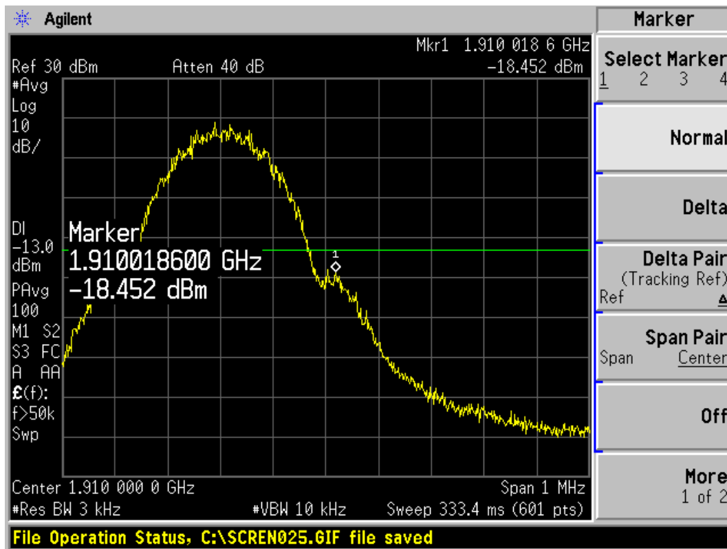
GSM1900 EGPRS 810 Channel
