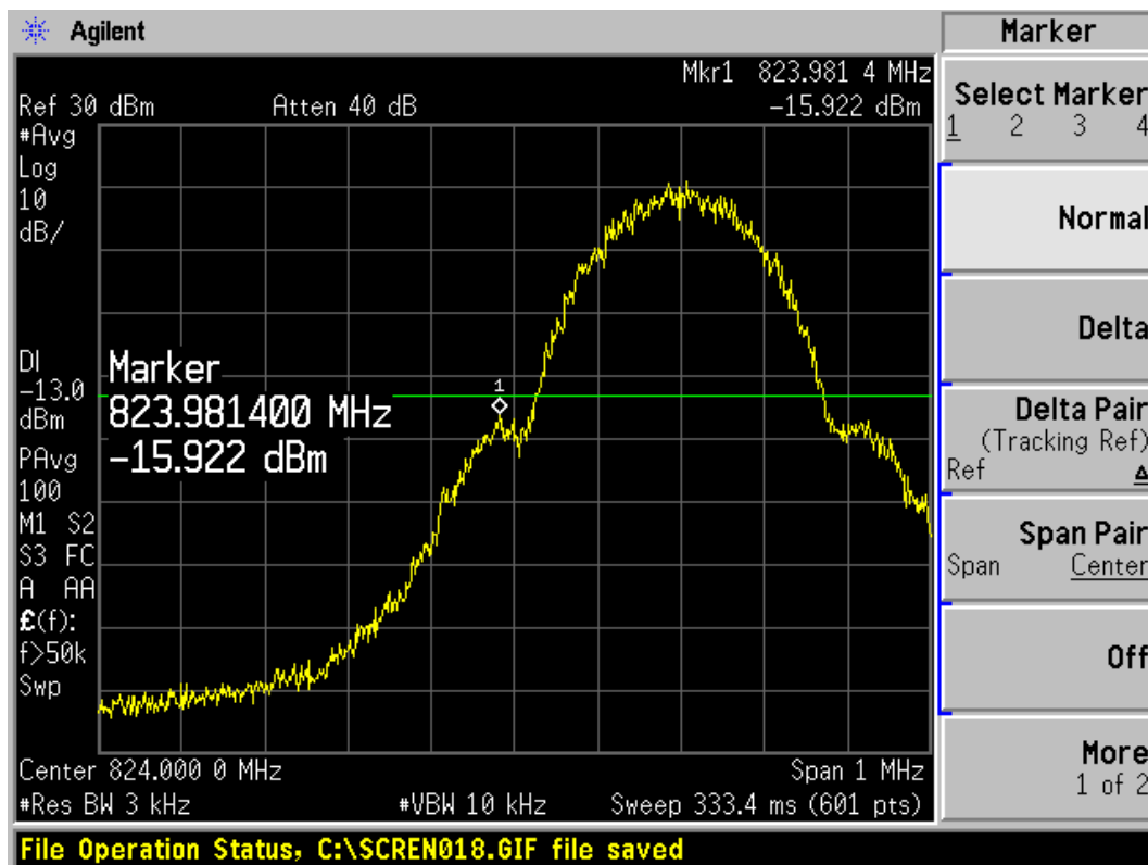
GSM 850 128 Channel
