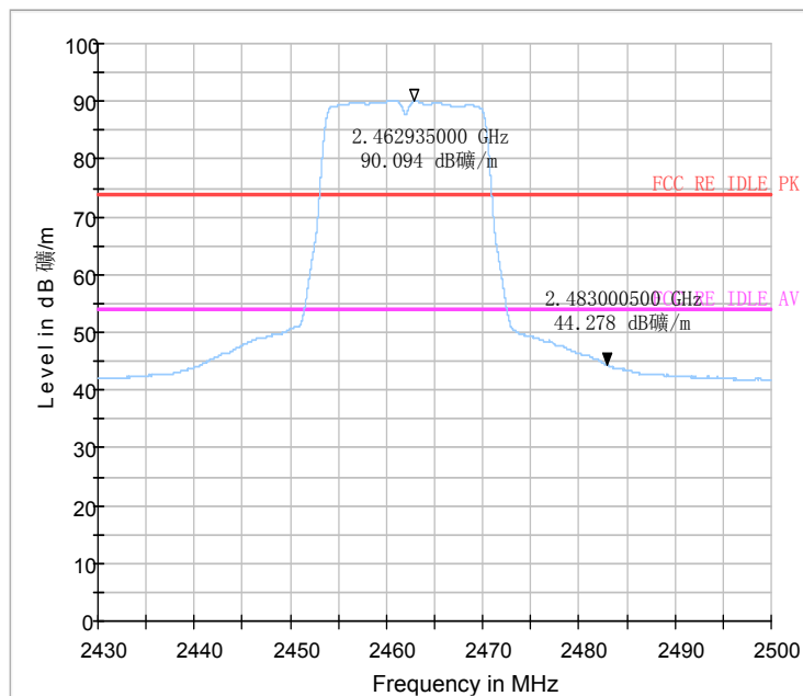
Fig.50 Radiated emission (Power): 802.11g, high channel
