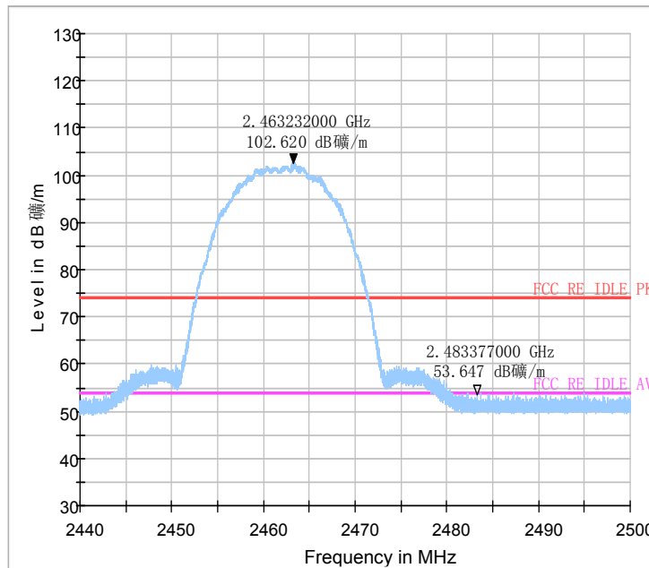
Fig.45 Radiated emission (Power): 802.11b, high channel
