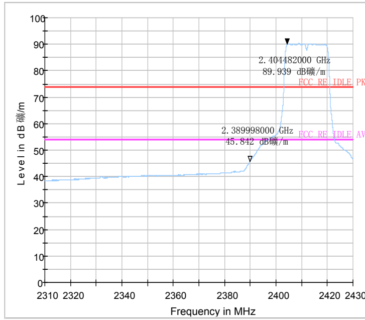
Fig.54 Radiated emission (Power): 802.11n, low channel
