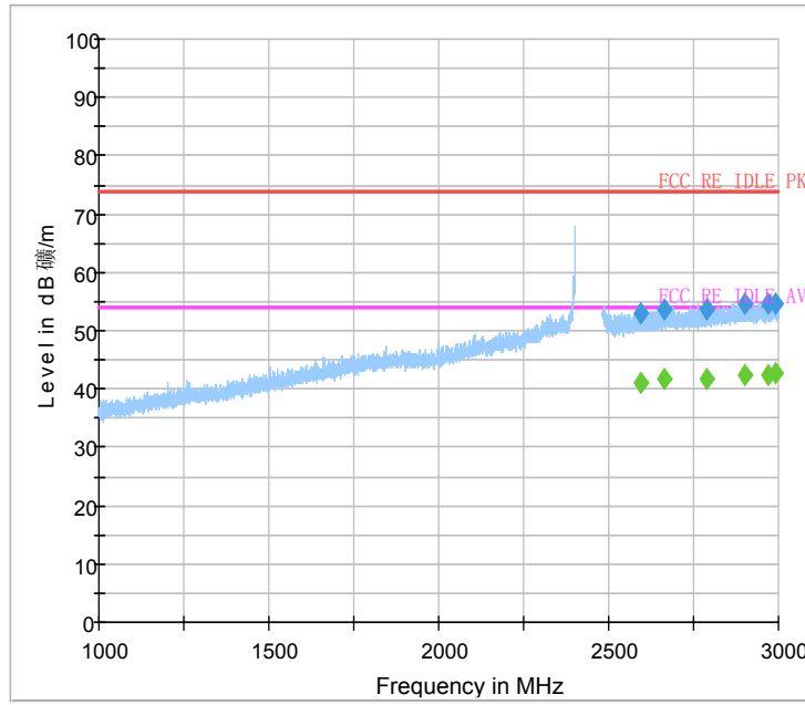
Fig.47 Radiated Spurious Emission (802.11b,Ch1,1GHz~3GHz)
