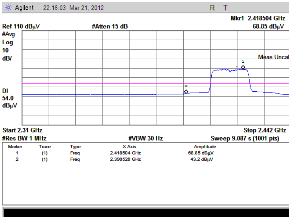
(Plot E2: Channel = 1 AVG @ 802.11n)
