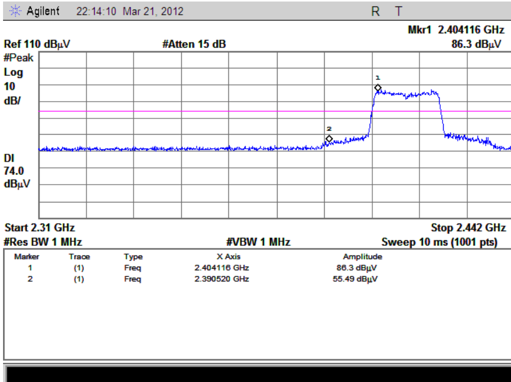
(Plot E1: Channel = 1 PEAK @ 802.11n)
