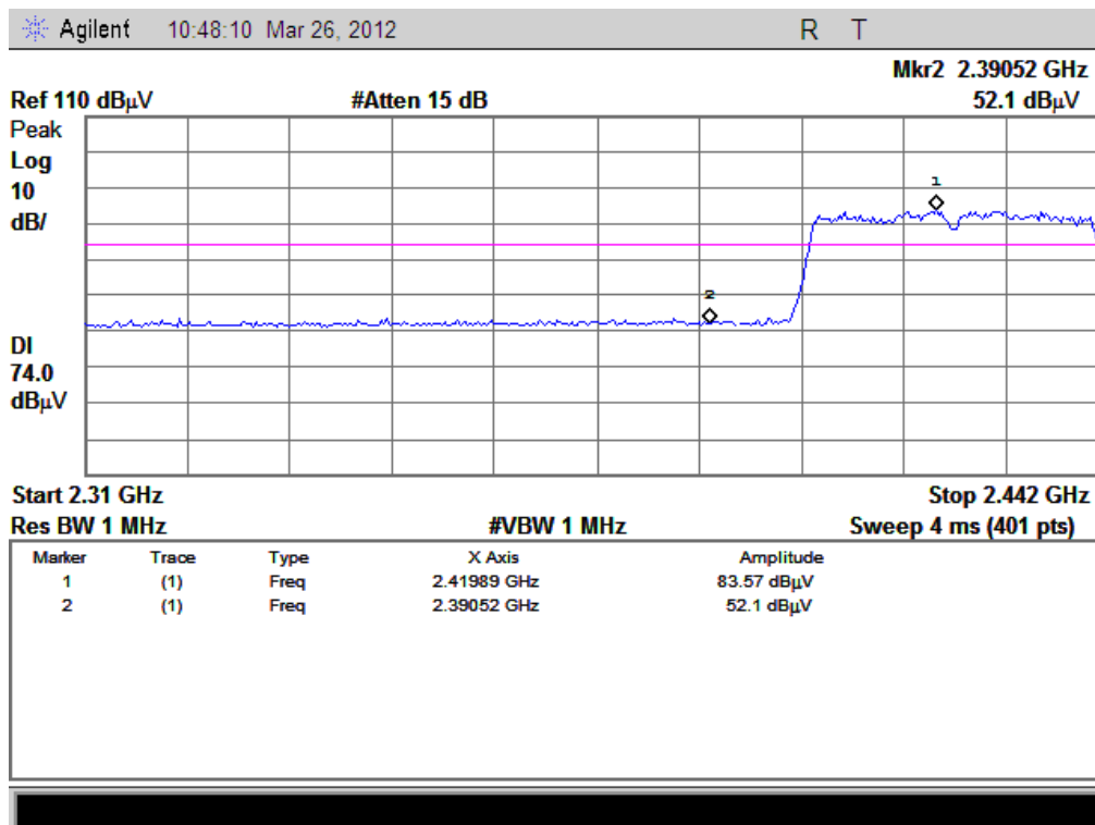
(Plot G1: Channel = 3 PEAK@802.11n)
