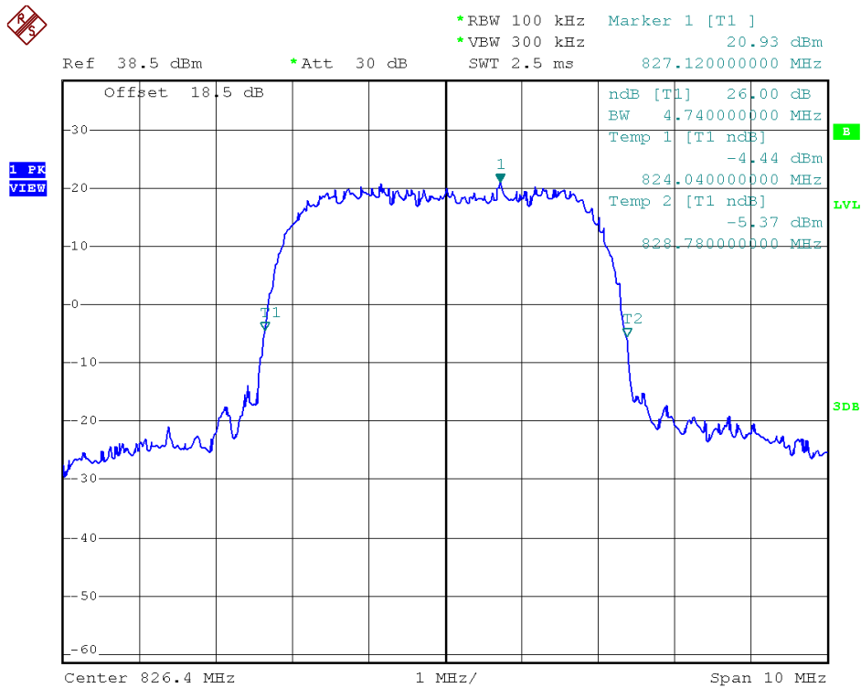
(Plot M1: HSPA+ 850MHz Channel = 4132)
