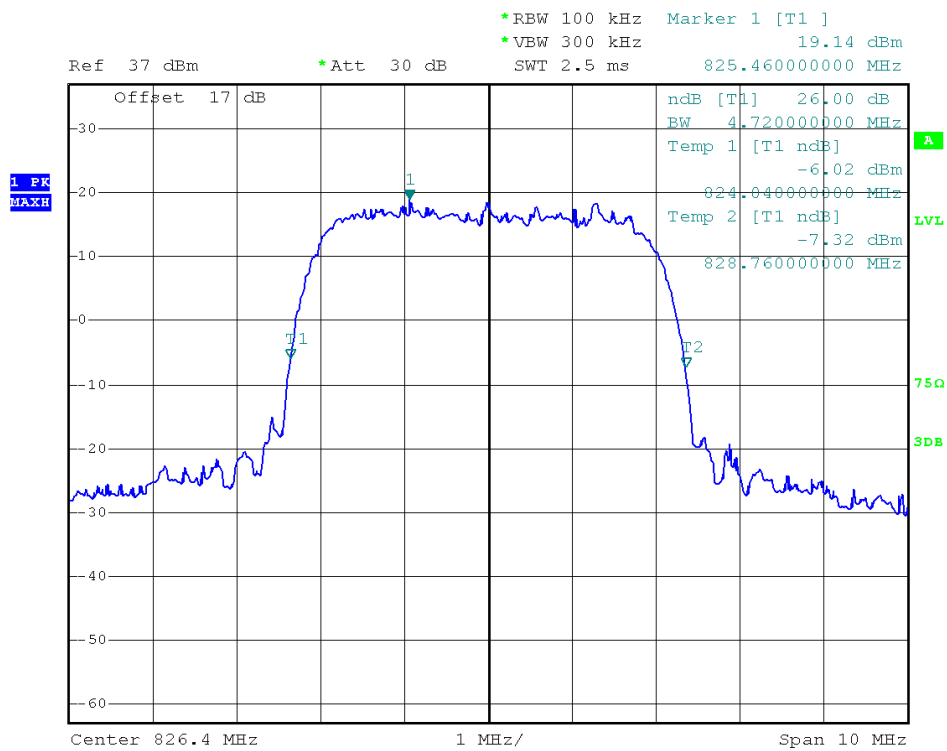
(Plot G1: WCDMA 850MHz Channel = 4132)
