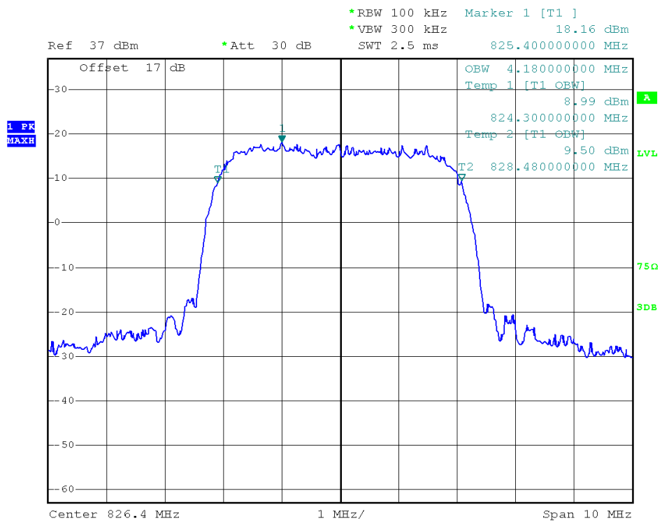
(Plot G2: WCDMA 850MHz Channel = 4132)
