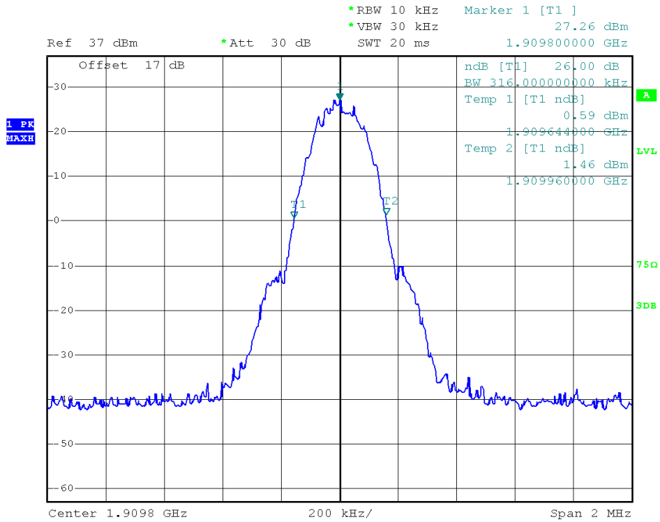
(Plot F5: EDGE 1900MHz Channel = 810)
