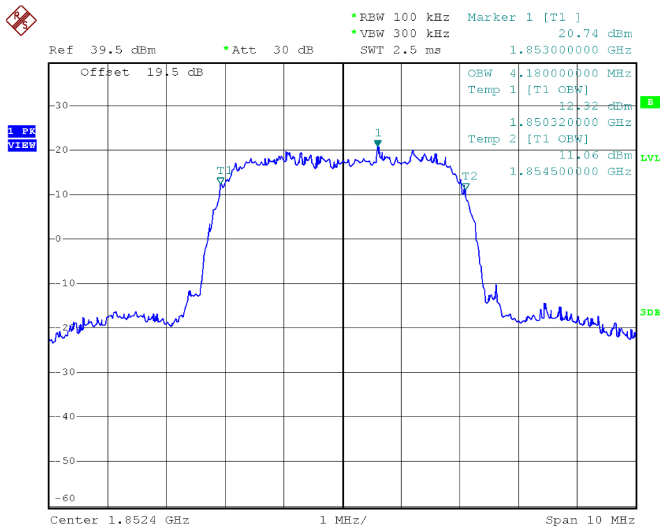
(Plot N2: HSPA+ 1900MHz Channel = 9262)
