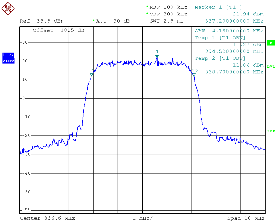
(Plot M4: HSPA+ 850 MHz Channel = 4183)
