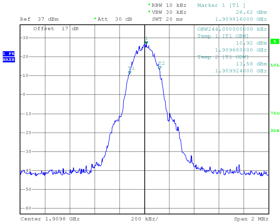
(Plot F6: EDGE 1900MHz Channel = 810)
