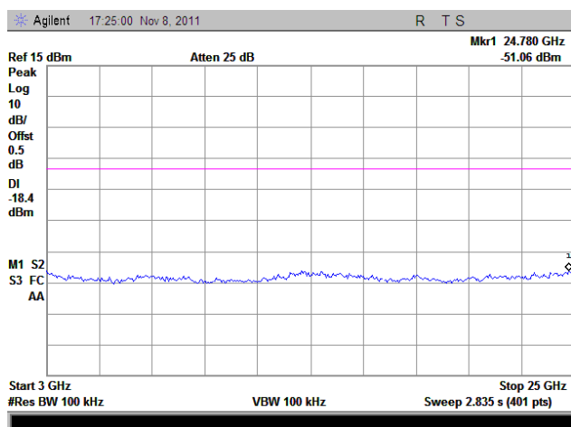
(Plot B.2: Channel = 6, 3GHz to 25GHz)
