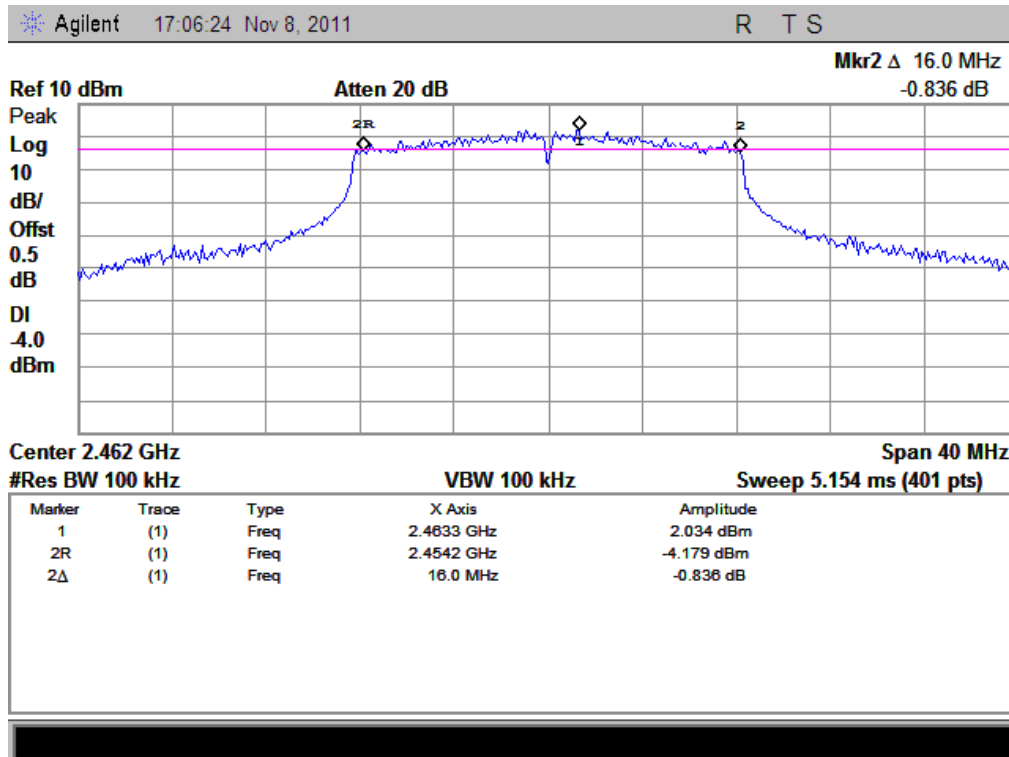
(Plot C: Chain1_Channel 11: 2462MHz)
