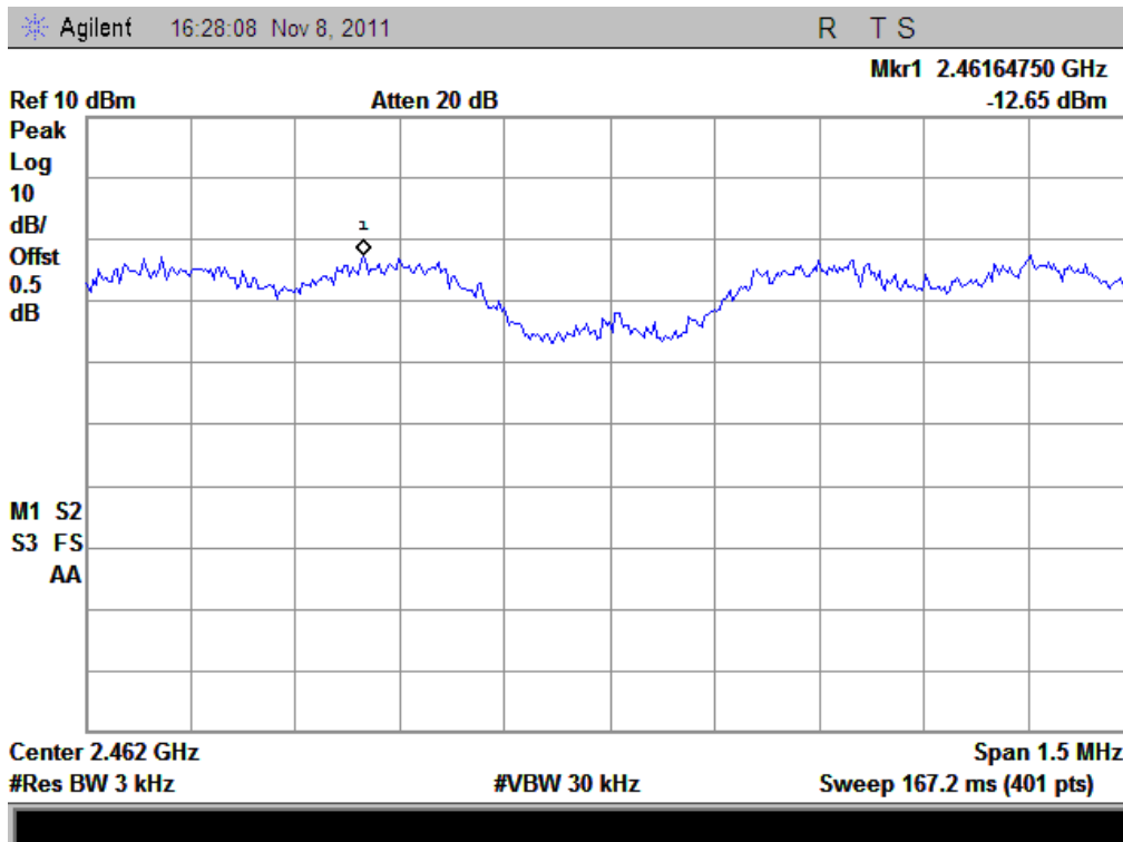
(Plot E: Chain1_Channel = 11)
