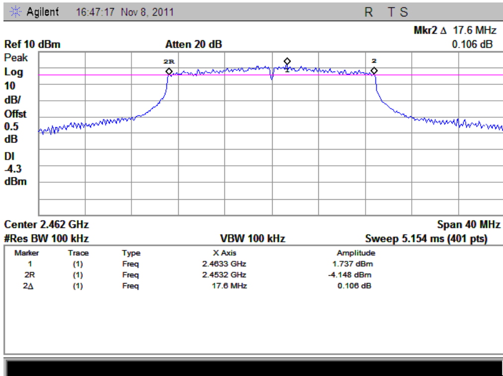
(Plot C: Chain1_Channel 11: 2462MHz)
