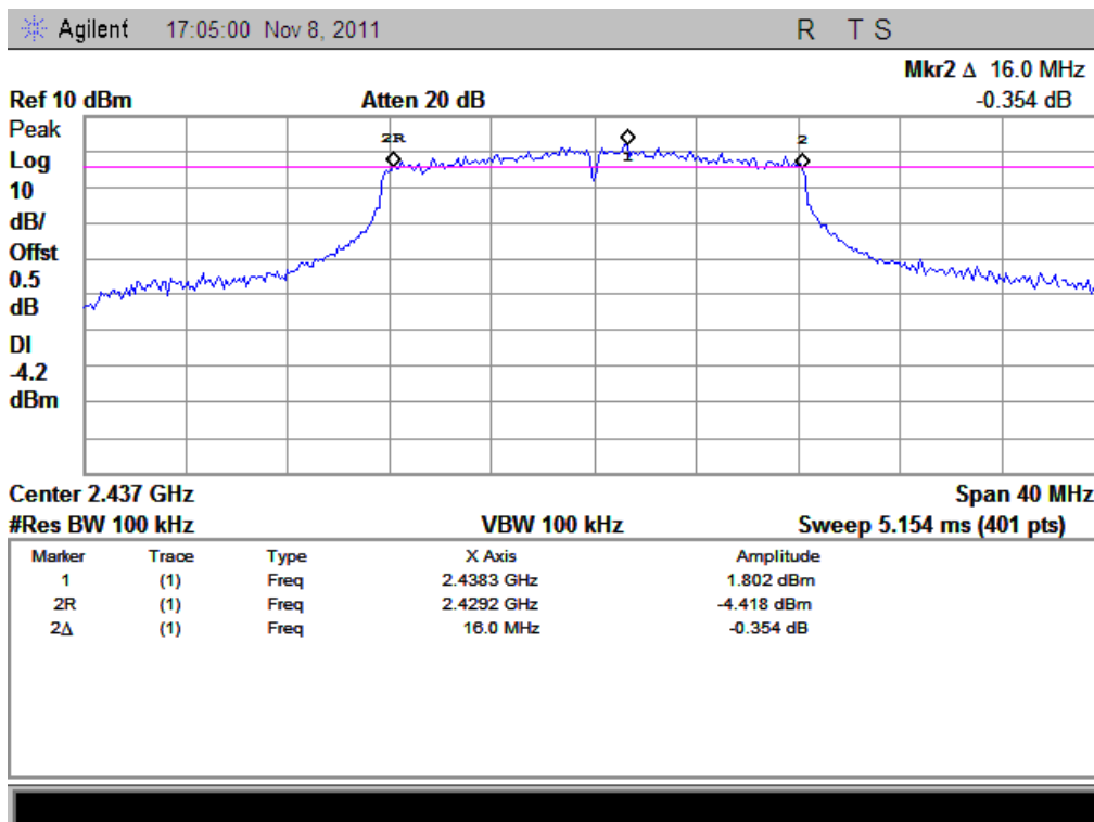
(Plot B: Chain1_Channel 6: 2437 MHz)
