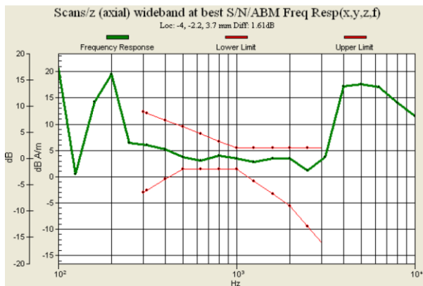
Fig. 9.5 GSM1900 Ch661
