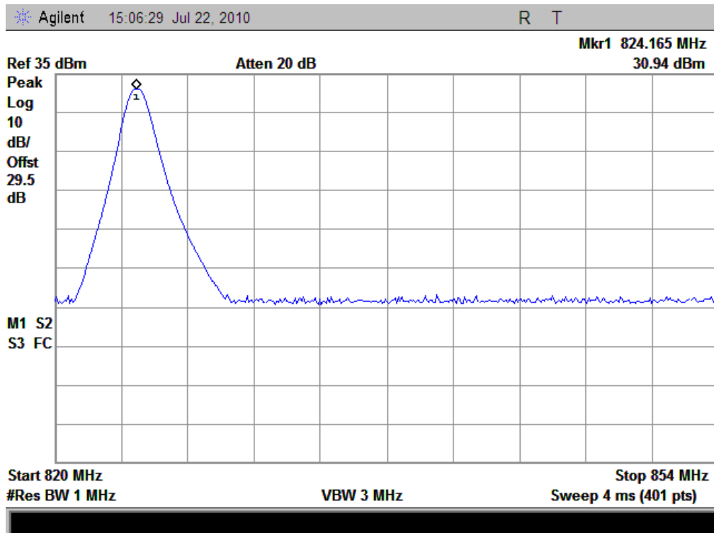
(Plot G: GPRS-4TX 850MHz Channel = 128)
