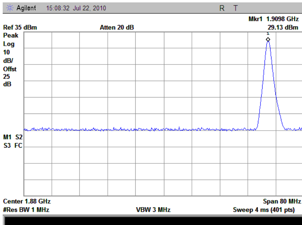
(Plot L: GPRS-4TX 1900MHz Channel = 810)
