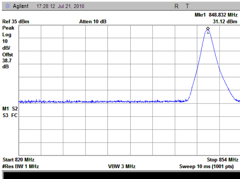
(Plot I: GPRS-4TX 850MHz Channel = 251)
