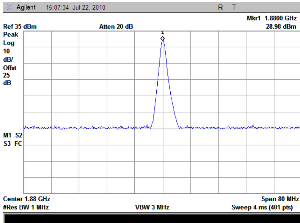
(Plot K: GPRS-4TX 1900MHz Channel = 661)
