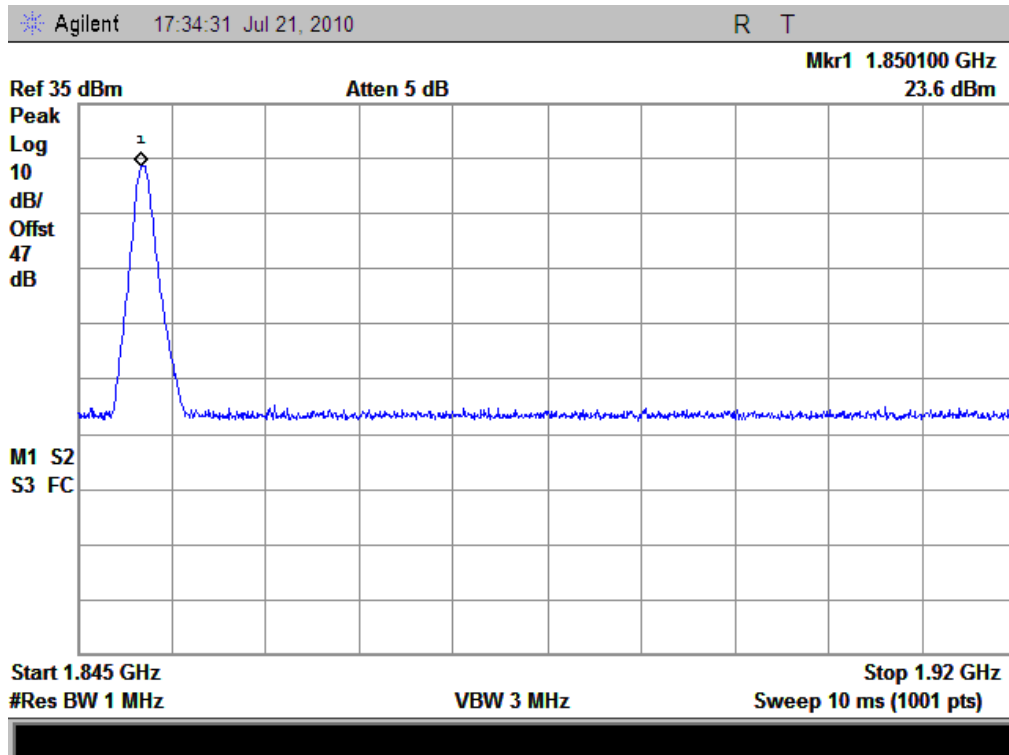
(Plot J: GPRS-4TX 1900MHz Channel = 512)
