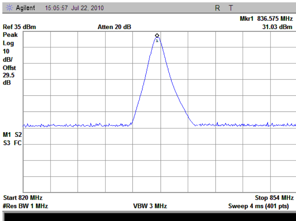
(Plot H: GPRS-4TX 850MHz Channel = 190)
