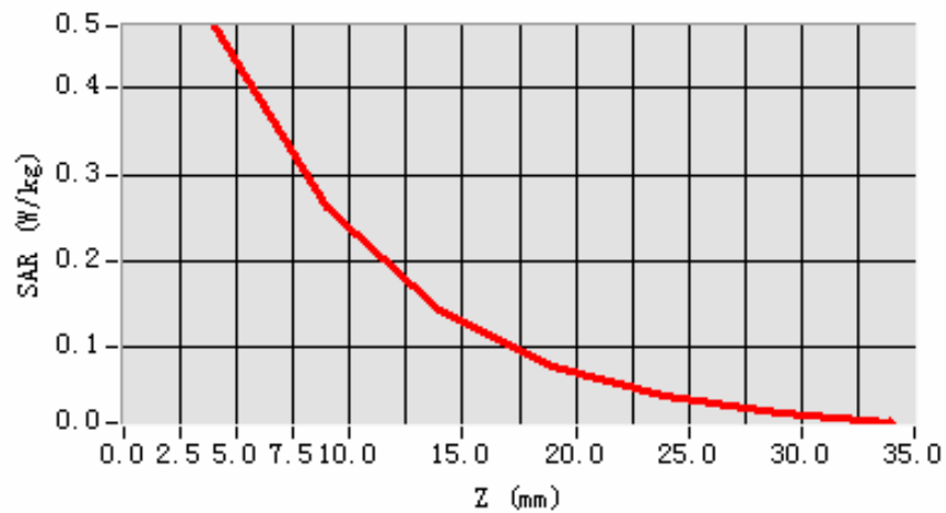
SAR, Z Axis Scan (X = -16, Y = 5)
