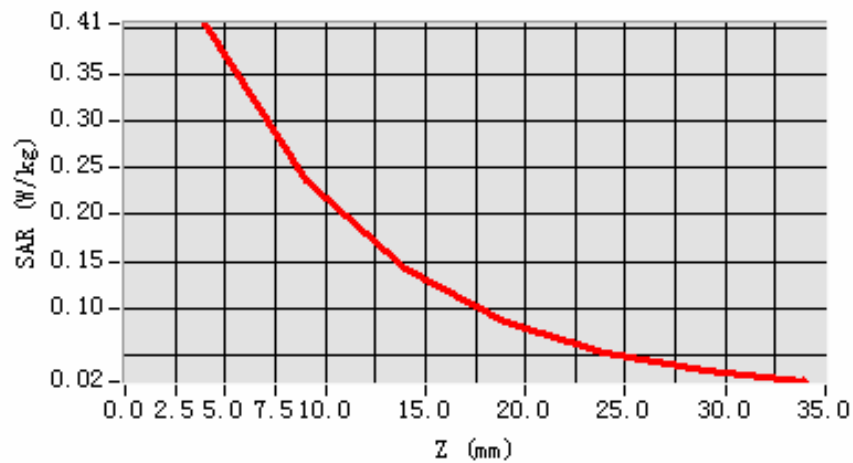
SAR, Z Axis Scan (X = 9, Y = 26)
