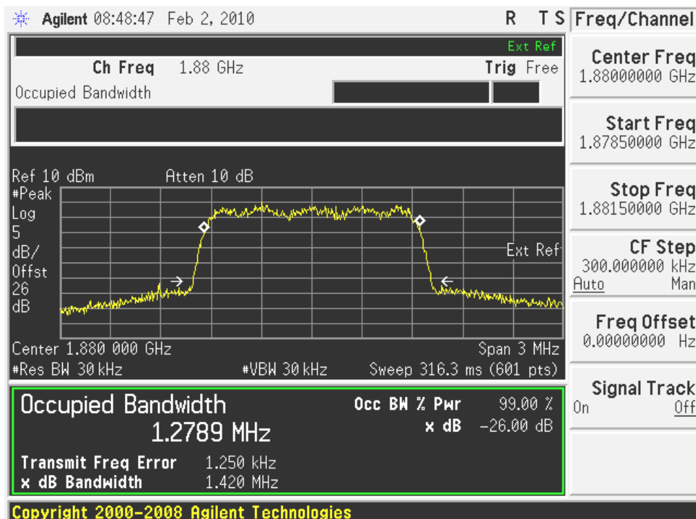
(Plot K: CDMA 1900-EVDO Channel = 600)
