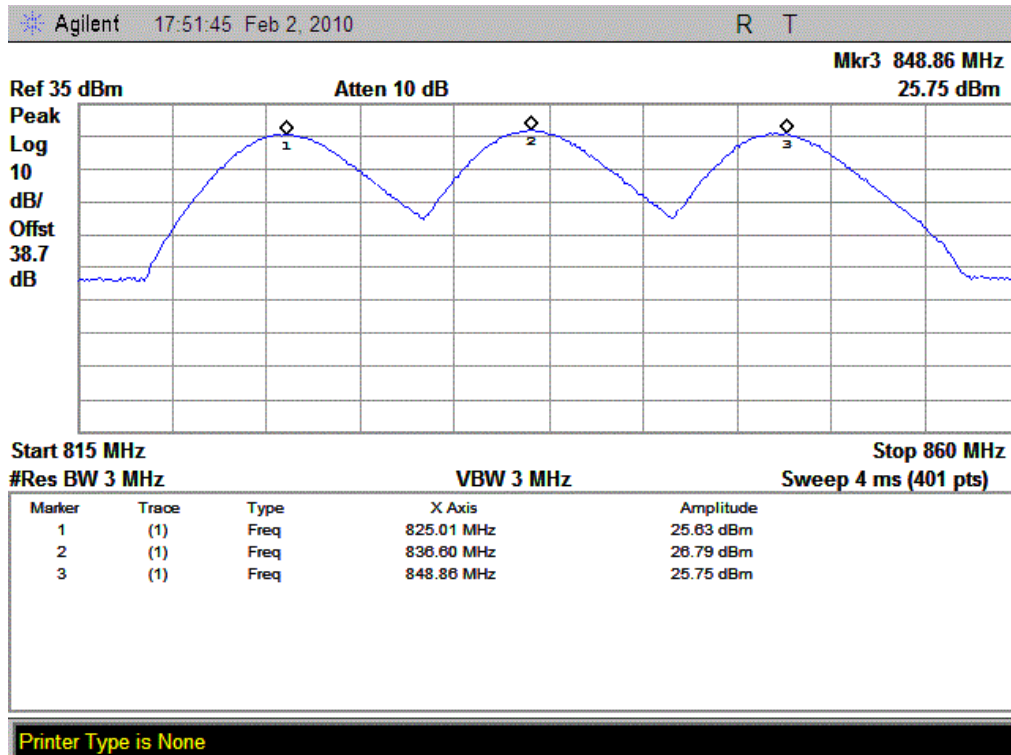
(Plot C: CDMA 800-EVDO Channel = 1013, 384, 777)
