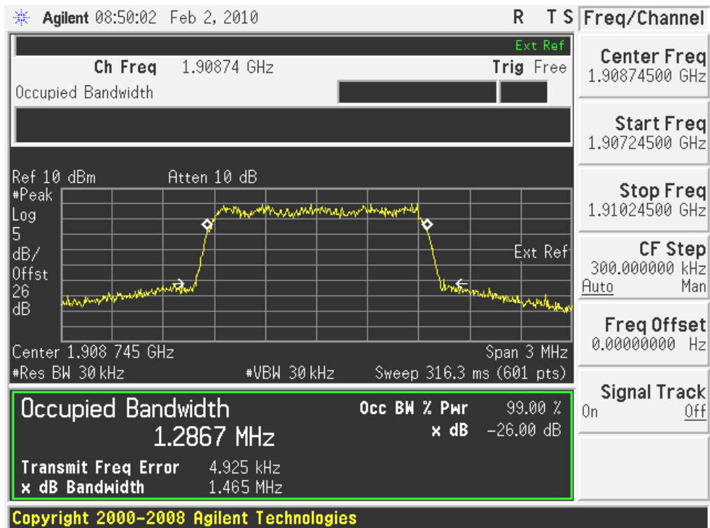
(Plot L: CDMA 1900-EVDO Channel = 1175)
