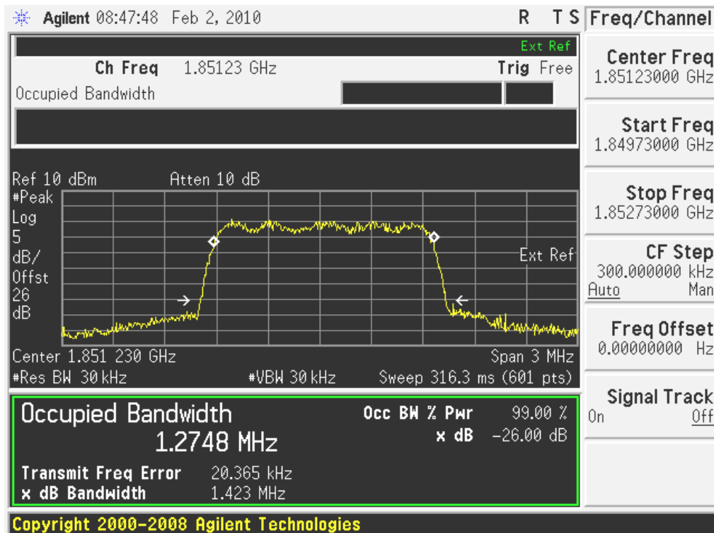
(Plot J: CDMA 1900-EVDO Channel = 25)
