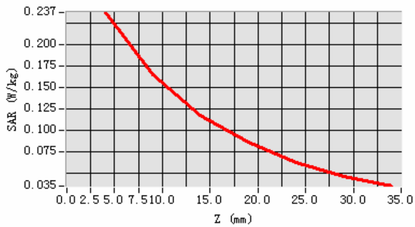
SAR, Z Axis Scan (X = -38, Y = -25)
