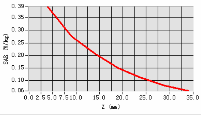
SAR, Z Axis Scan (X = -25, Y = -10)
