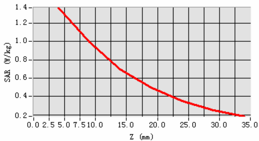
SAR, Z Axis Scan (X = -47, Y = -33)
