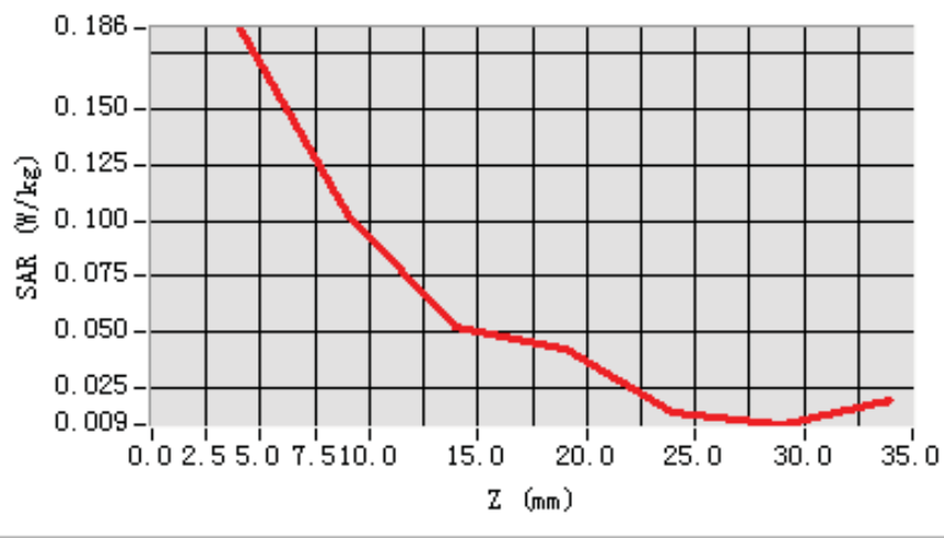
SAR, Z Axis Scan (X = -9, Y = -33)
