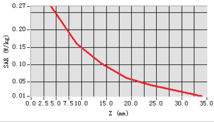
SAR, Z Axis Scan (X = -6, Y = -33)
