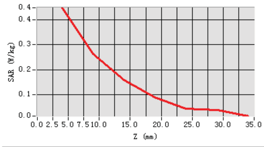
SAR, Z Axis Scan (X = -22, Y = -1)
