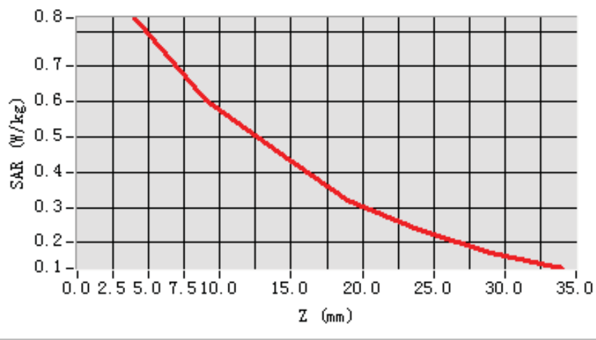
SAR, Z Axis Scan (X = -26, Y = -16)
