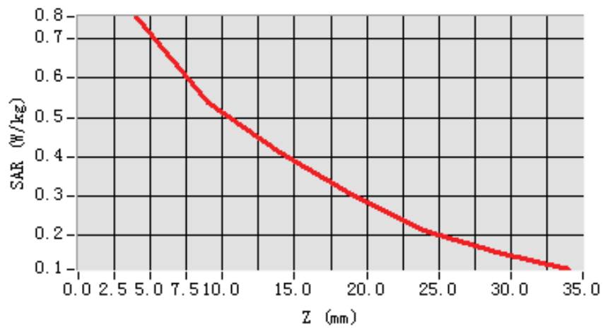
SAR, Z Axis Scan (X = -20, Y = -11)
