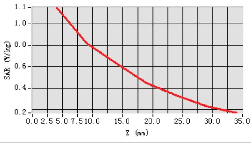
SAR, Z Axis Scan (X = -30, Y = -17)
