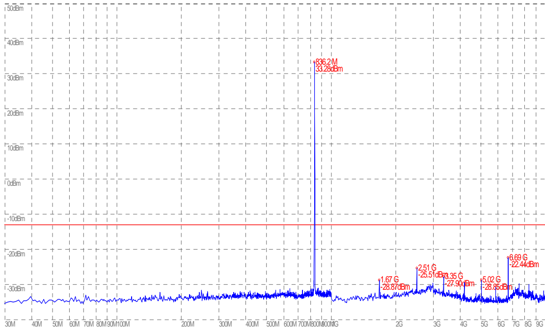
(Plot B: GSM 850MHz Channel = 190, 30MHz to 9GHz)
