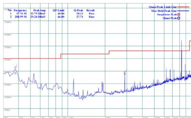
(Plot B: Test Antenna Horizontal)
