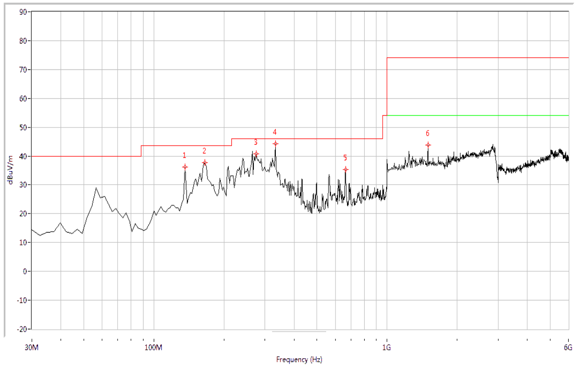
(Plot B: 30MHz – 6GHz, Test Antenna Horizontal)
