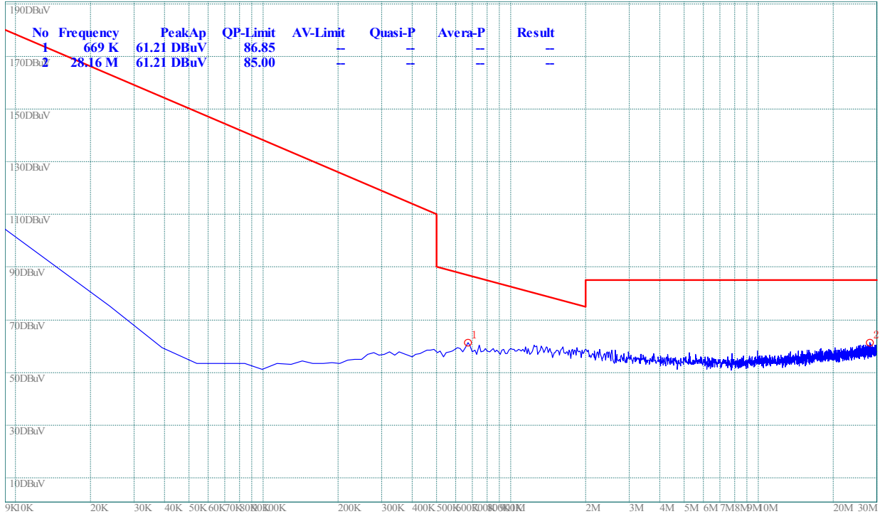
(Plot B.0: 9kHz to 30MHz @ GFSK, channel 39)
