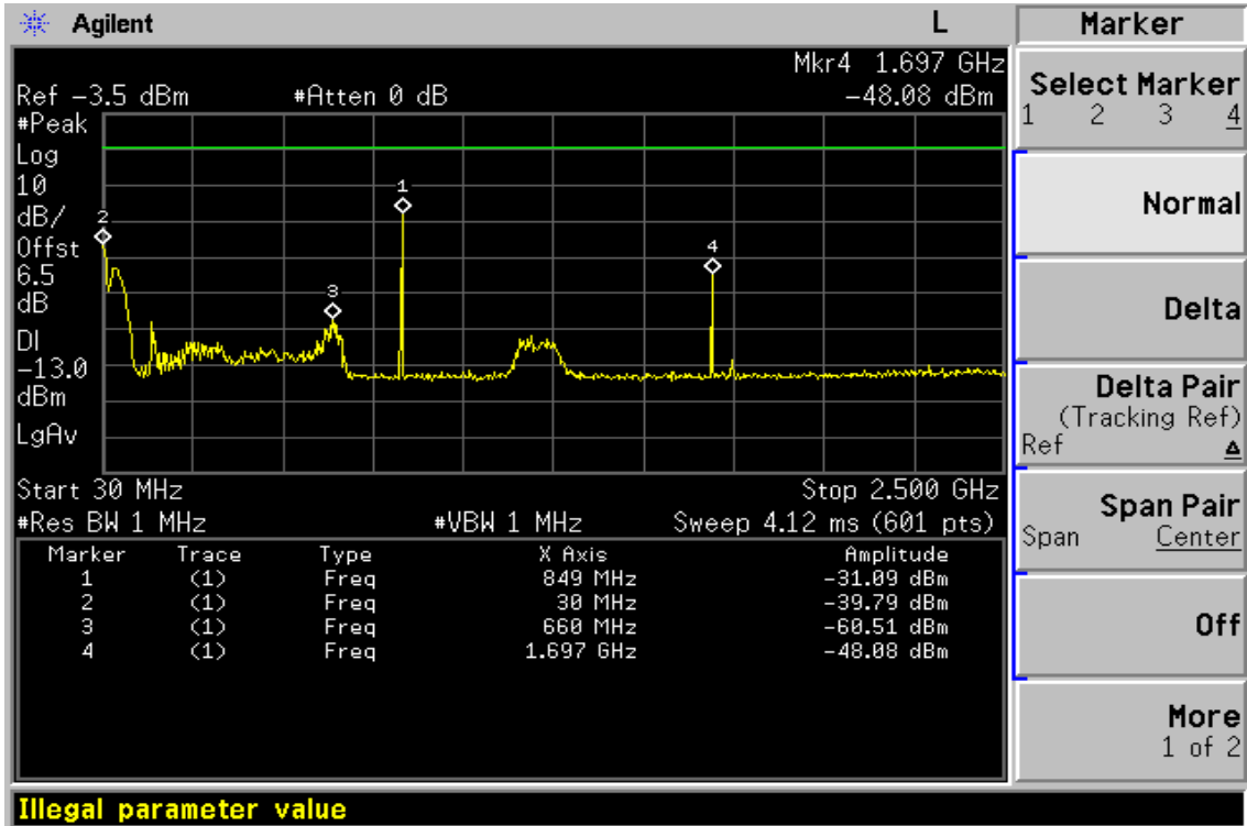
Figure 8-5: Out of Band emission at antenna terminals–GSM 850 Channel High
