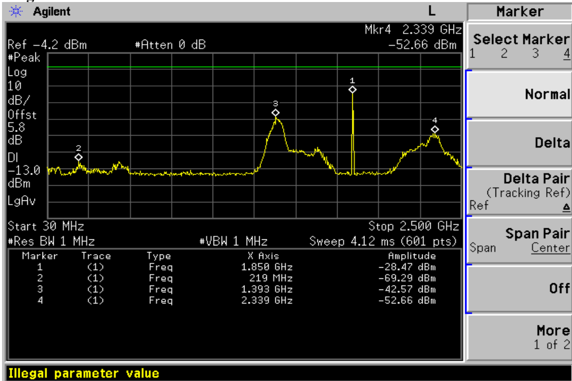
Figure 8-10: Out of Band emission at antenna terminals– PCS 1900 Channel Low
