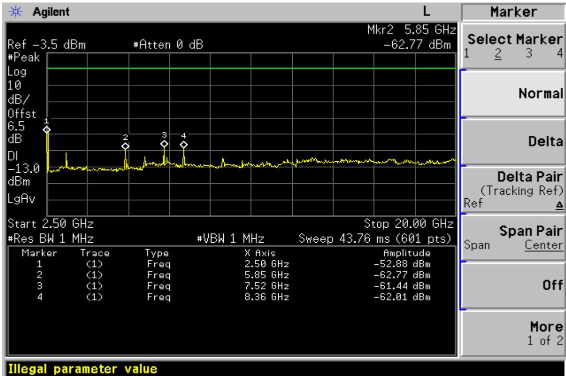
Figure 8-4: Out of Band emission at antenna terminals –GSM 850 Channel Mid
