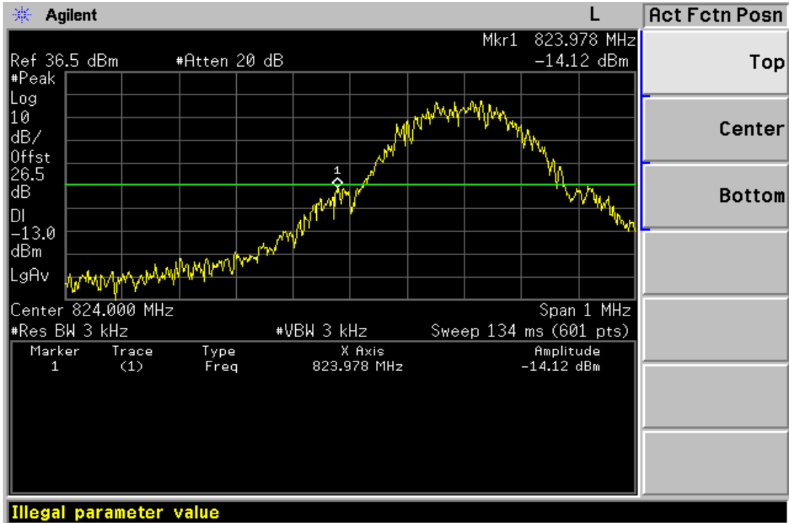
Figure 8-7: Band edge emission at antenna terminals – GSM 850 CH Lowest
