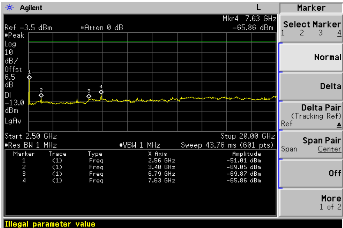
Figure 8-6: Out of Band emission at antenna terminals–GSM 850 Channel High
