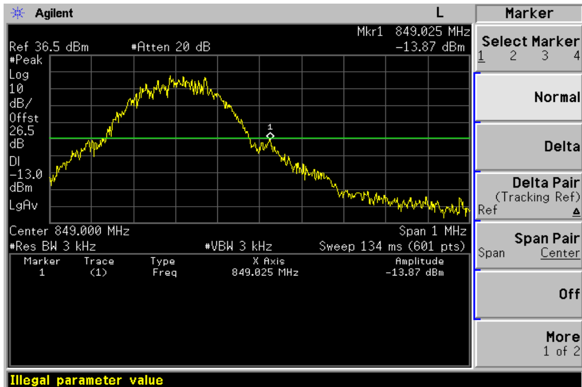
Figure 8-8: Band edge emission at antenna terminals – GSM 850 CH Hightest
