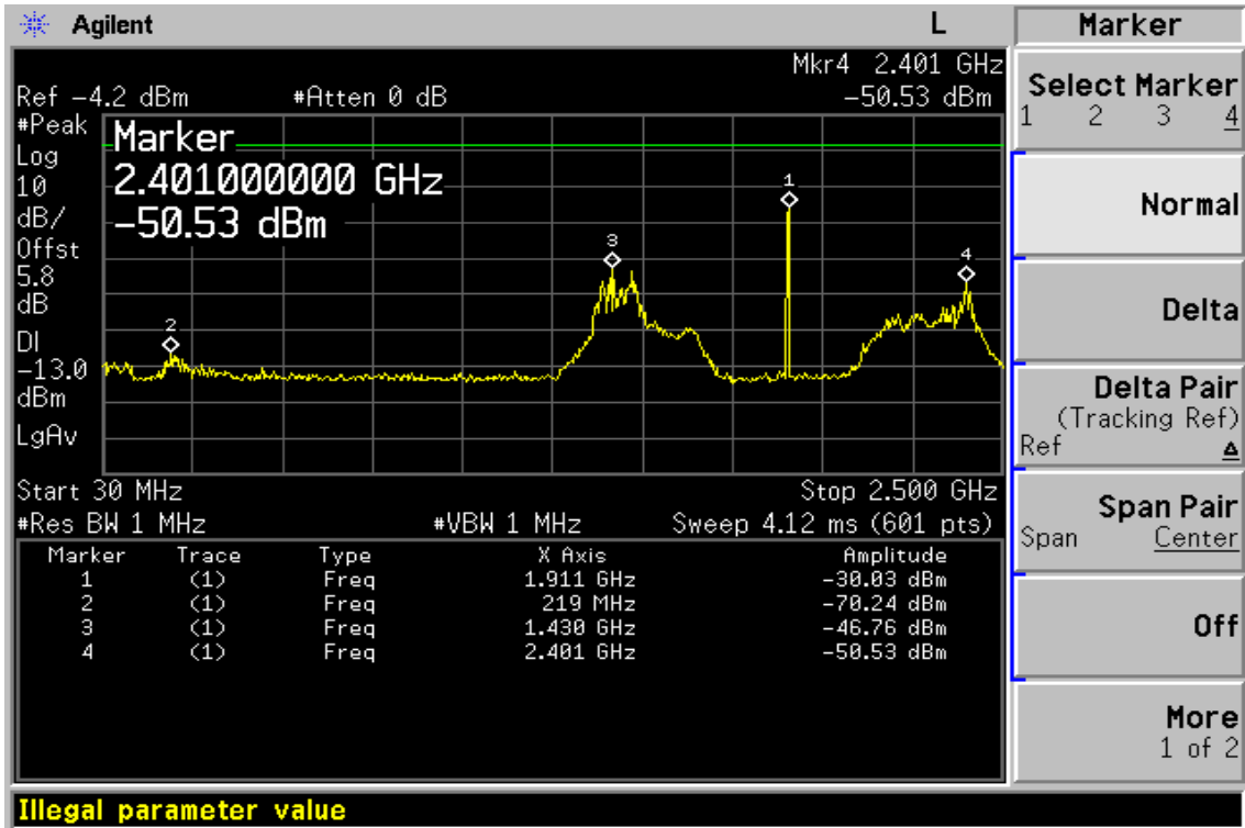
Figure 8-14: Out of Band emission at antenna terminals–PCS 1900 Channel High
