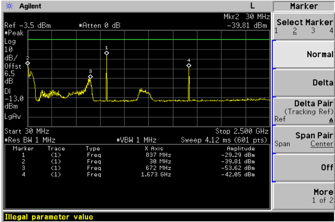
Figure 8-3: Out of Band emission at antenna terminals –GSM 850 Channel Mid
