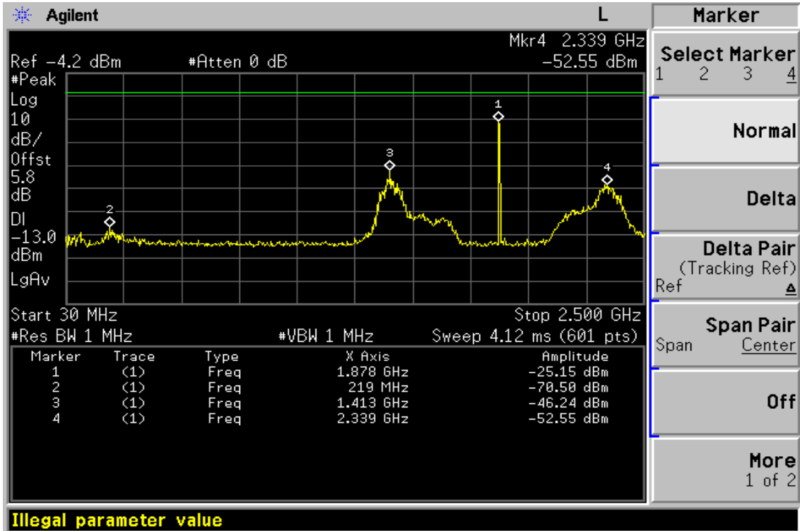
Figure 8-12: Out of Band emission at antenna terminals –PCS 1900 Channel Mid
