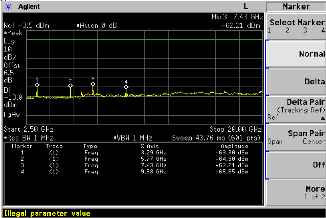
Figure 8-2: Out of Band emission at antenna terminals– GSM 850 Channel Low
