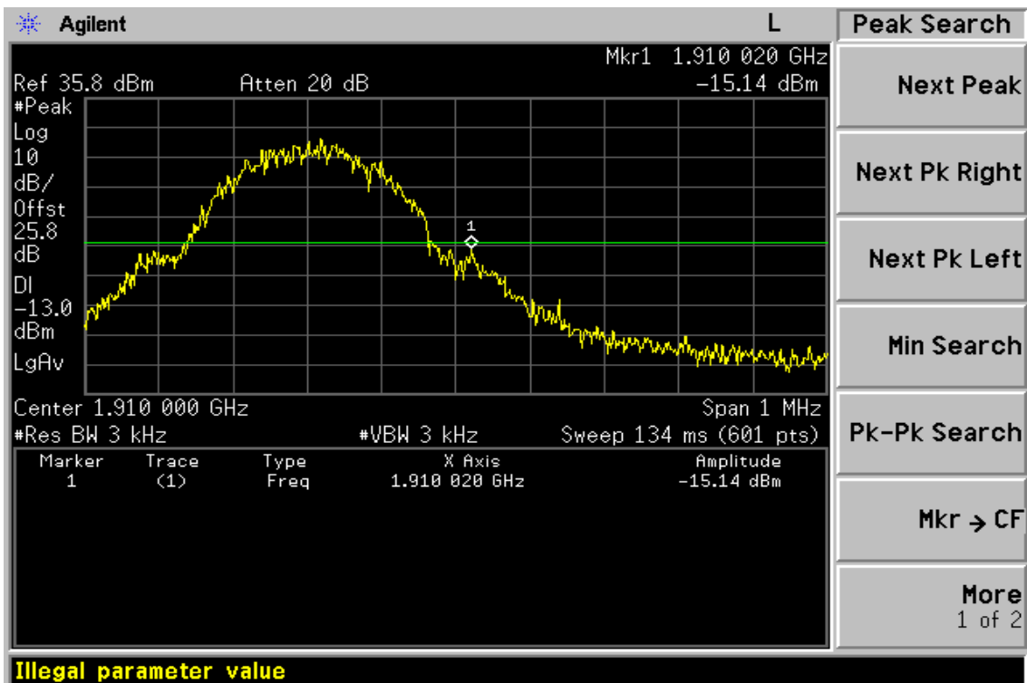
Figure 8-16: Band edge emission at antenna terminals – PCS 1900 CH Highest
