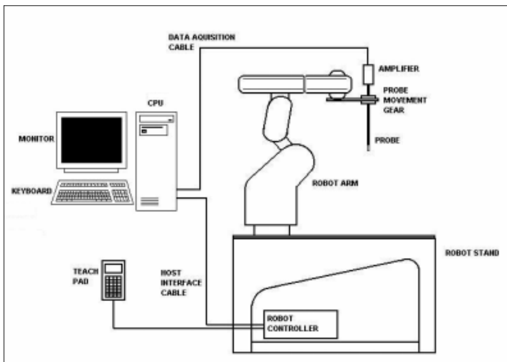
Figure1. SAR Lab Test Measurement Set-up
