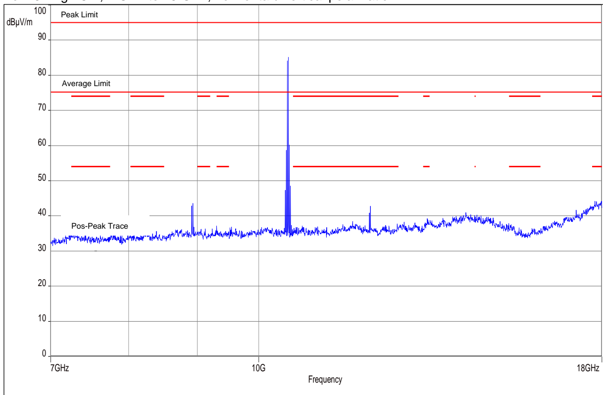
Plot No. 16: High Ch., 7 GHz to 18 GHz, horizontal / vertical polarization
