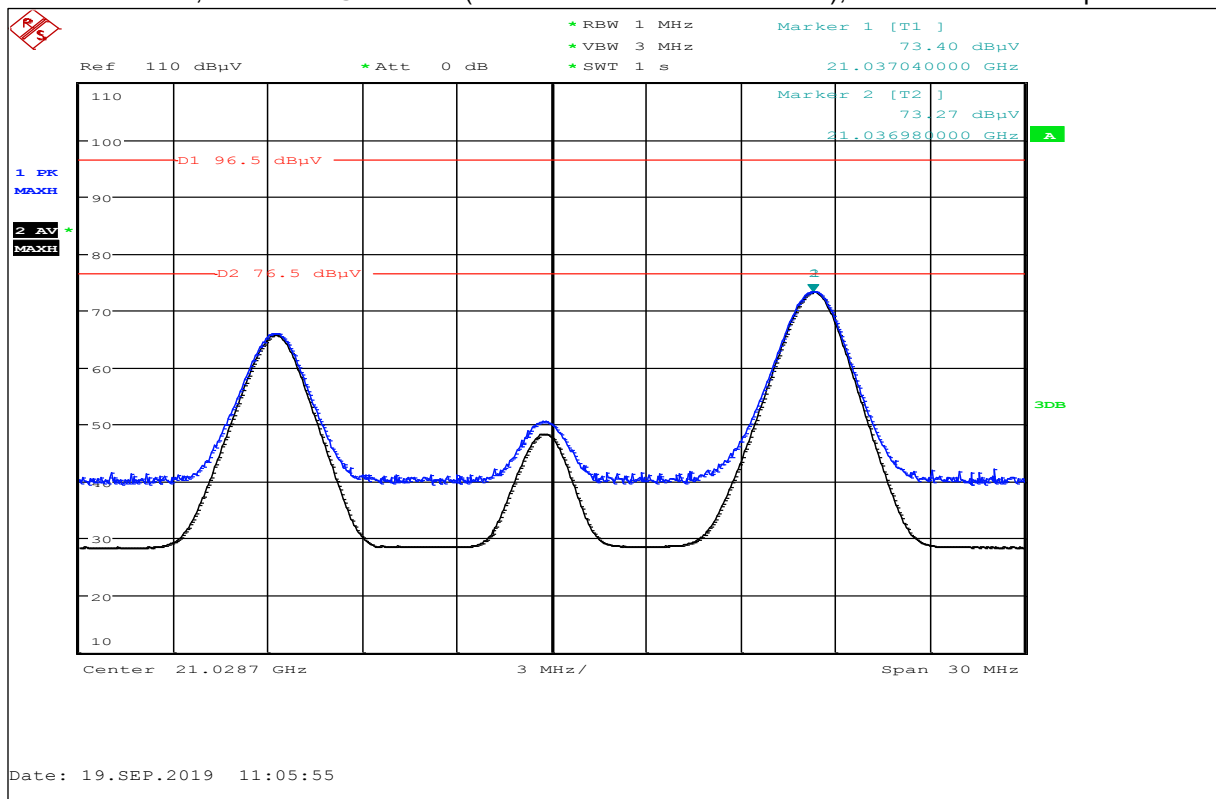
Plot No. 20: Low Ch., Harmonic @ 21 GHz (restricted band 17.7-21.4 GHz), horizontal / vertical polarization
