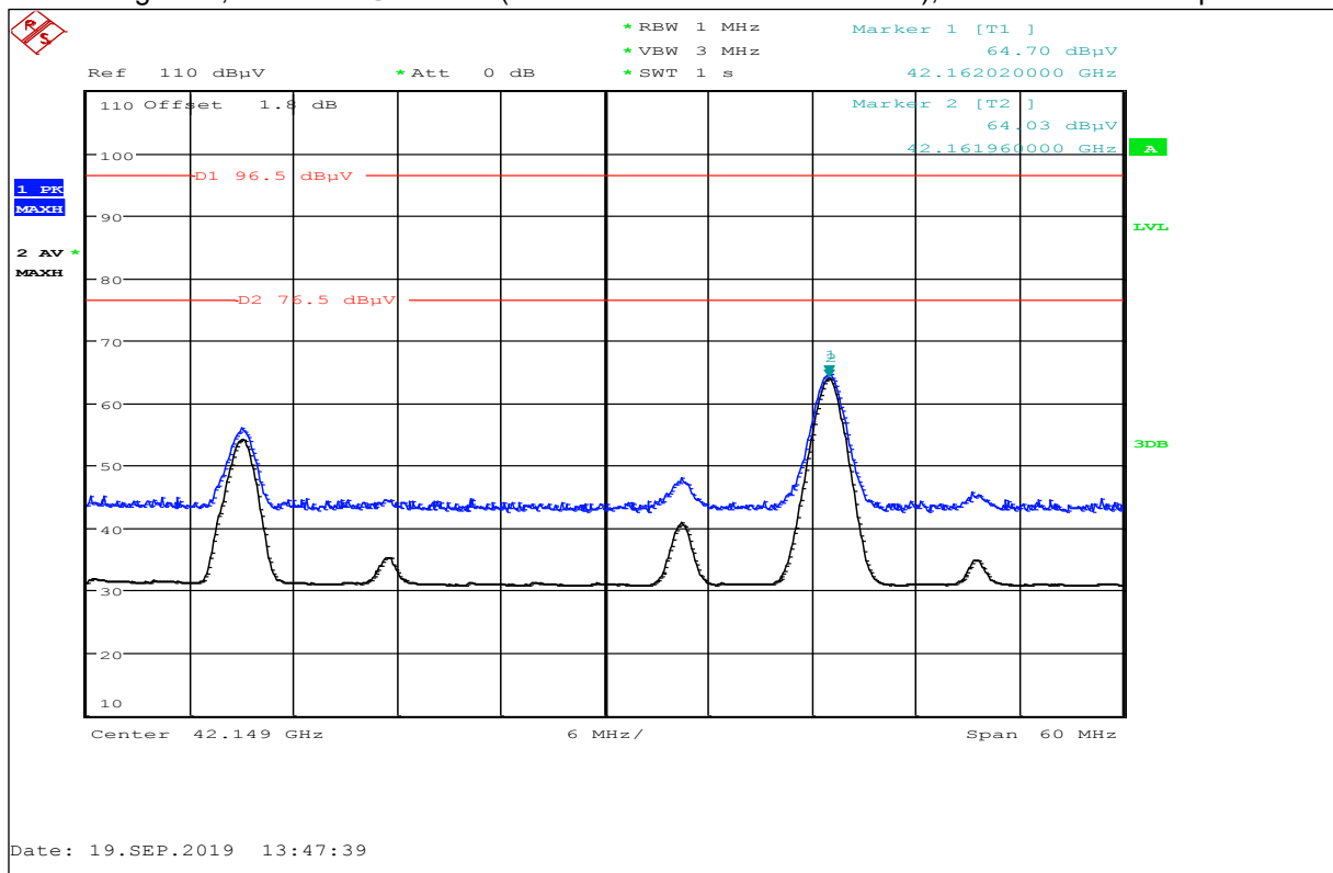
Plot No. 30: High Ch., Harmonic@42 GHz (restricted band above 38.6 GHz), horizontal / vertical polarization
