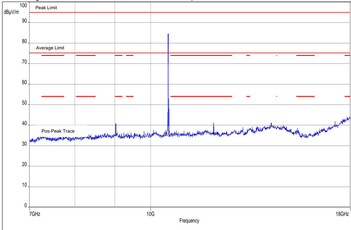
Plot shows the wanted signal at Middle Channel
