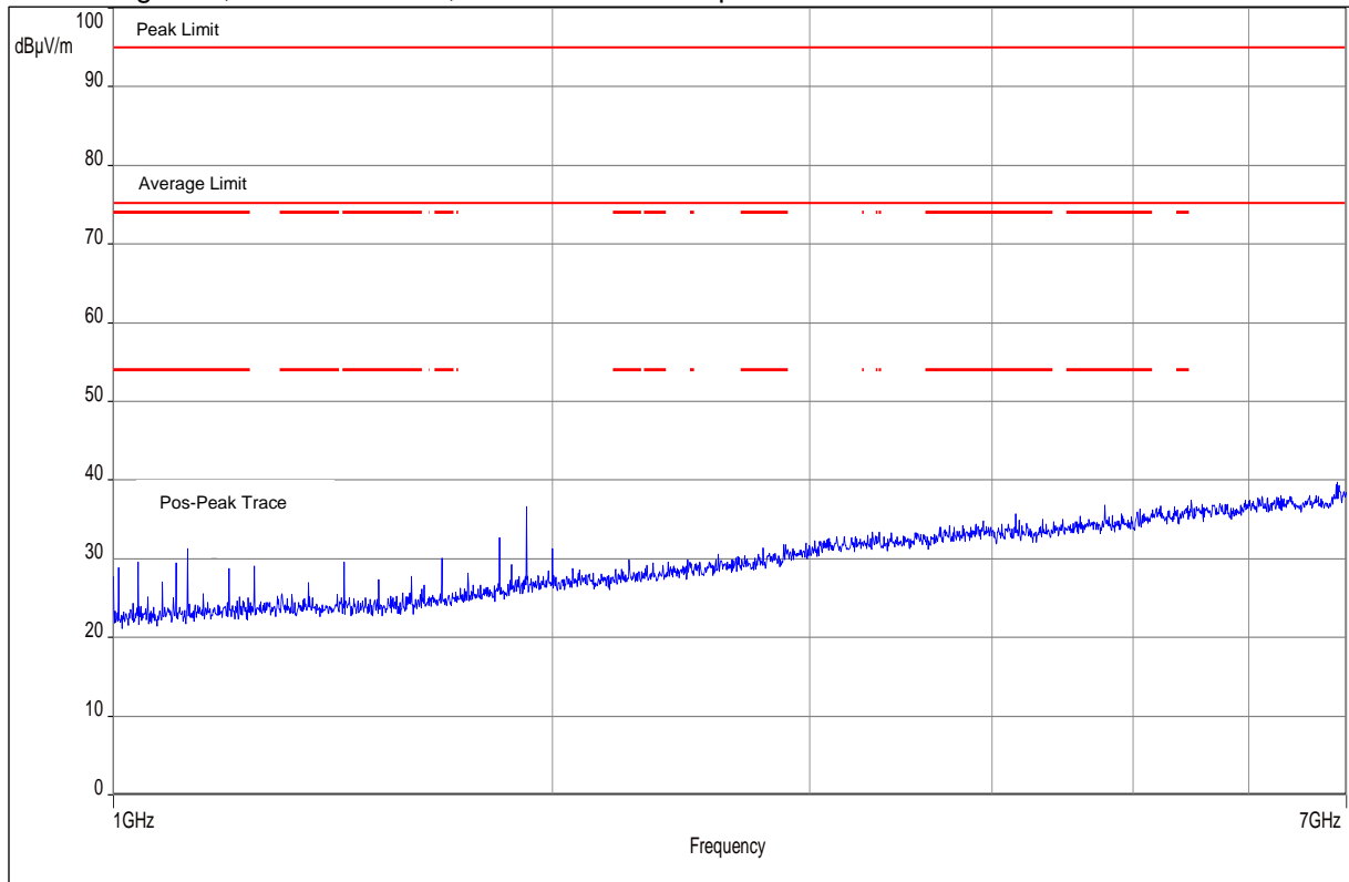
Plot No. 15: High Ch., 1 GHz to 7 GHz, horizontal / vertical polarization
