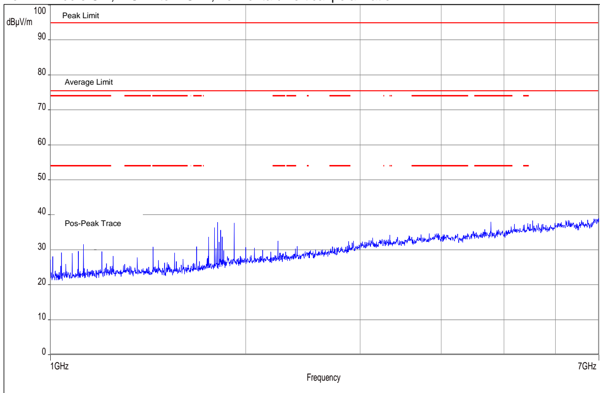
Plot No. 14: Middle Ch., 1 GHz to 7 GHz, horizontal / vertical polarization
