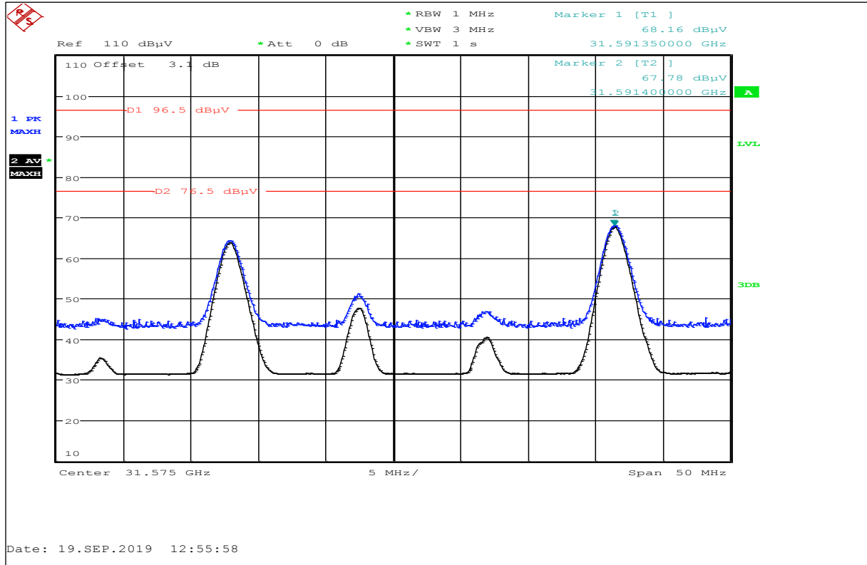
Plot No. 25: Middle Ch., Harmonic @ 31 GHz (restricted band 31.2-31.8 GHz), horizontal / vertical polarization
