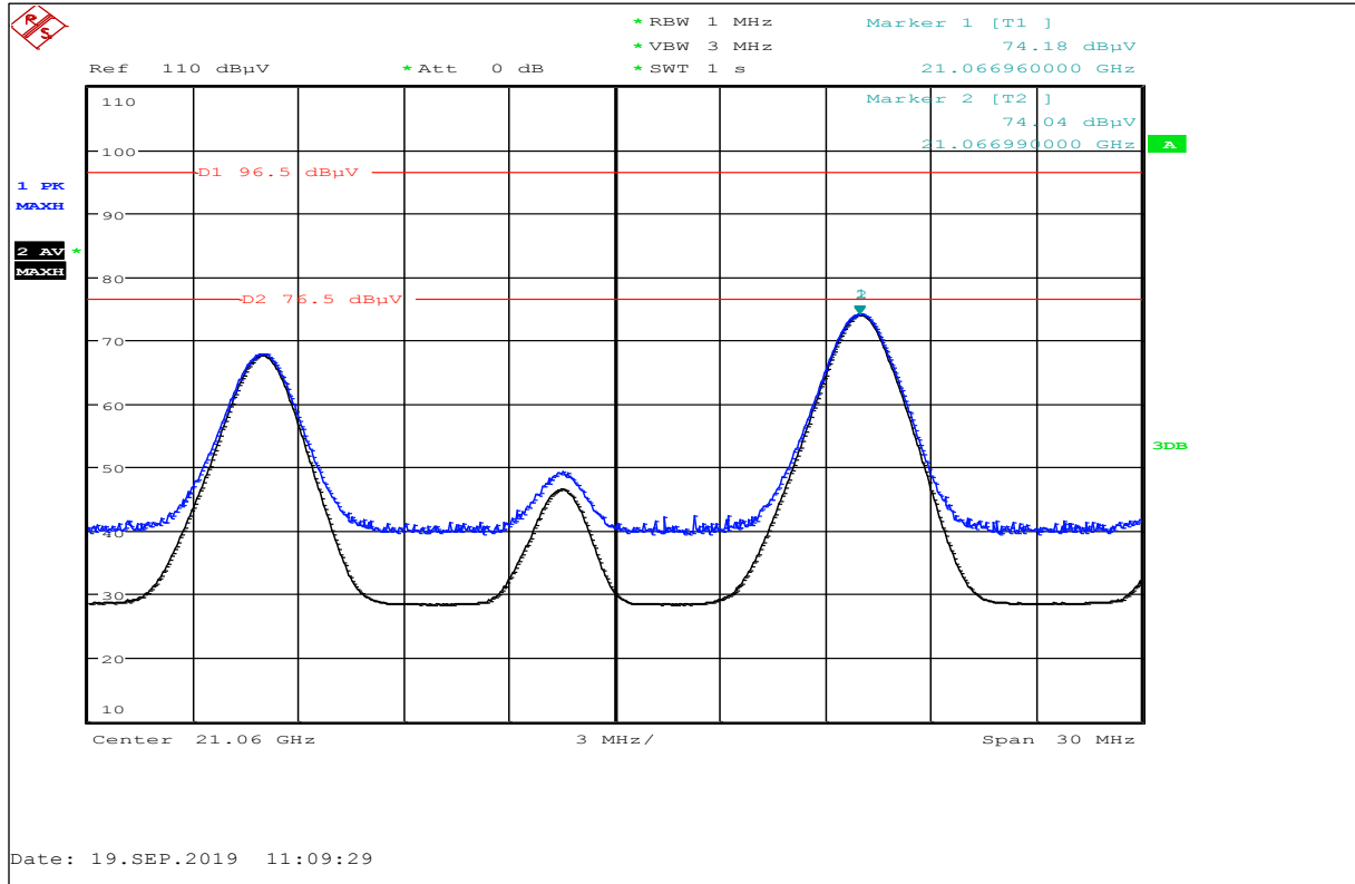
Plot No. 21: Middle Ch., Harmonic @ 21 GHz (restricted band 17.7-21.4 GHz), horizontal / vertical polarization
