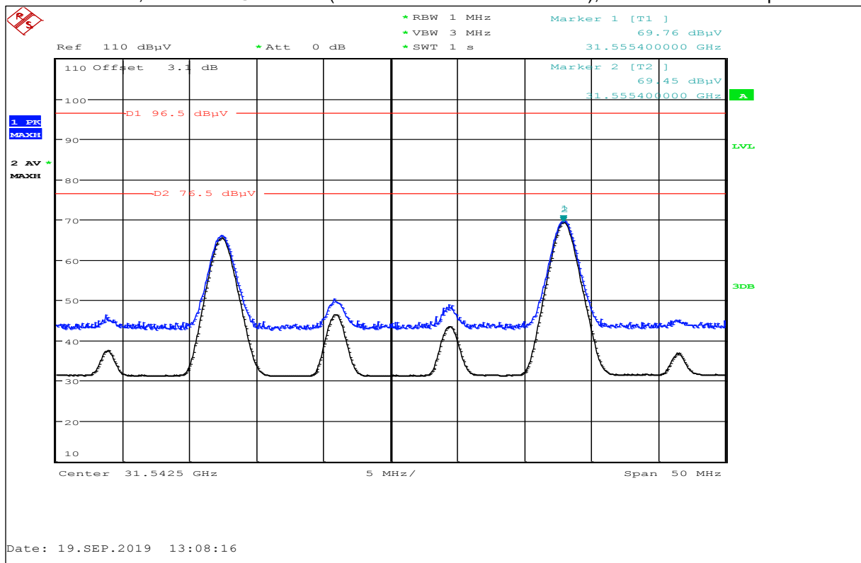
Plot No. 24: Low Ch., Harmonic @ 31 GHz (restricted band 31.2-31.8 GHz), horizontal / vertical polarization
