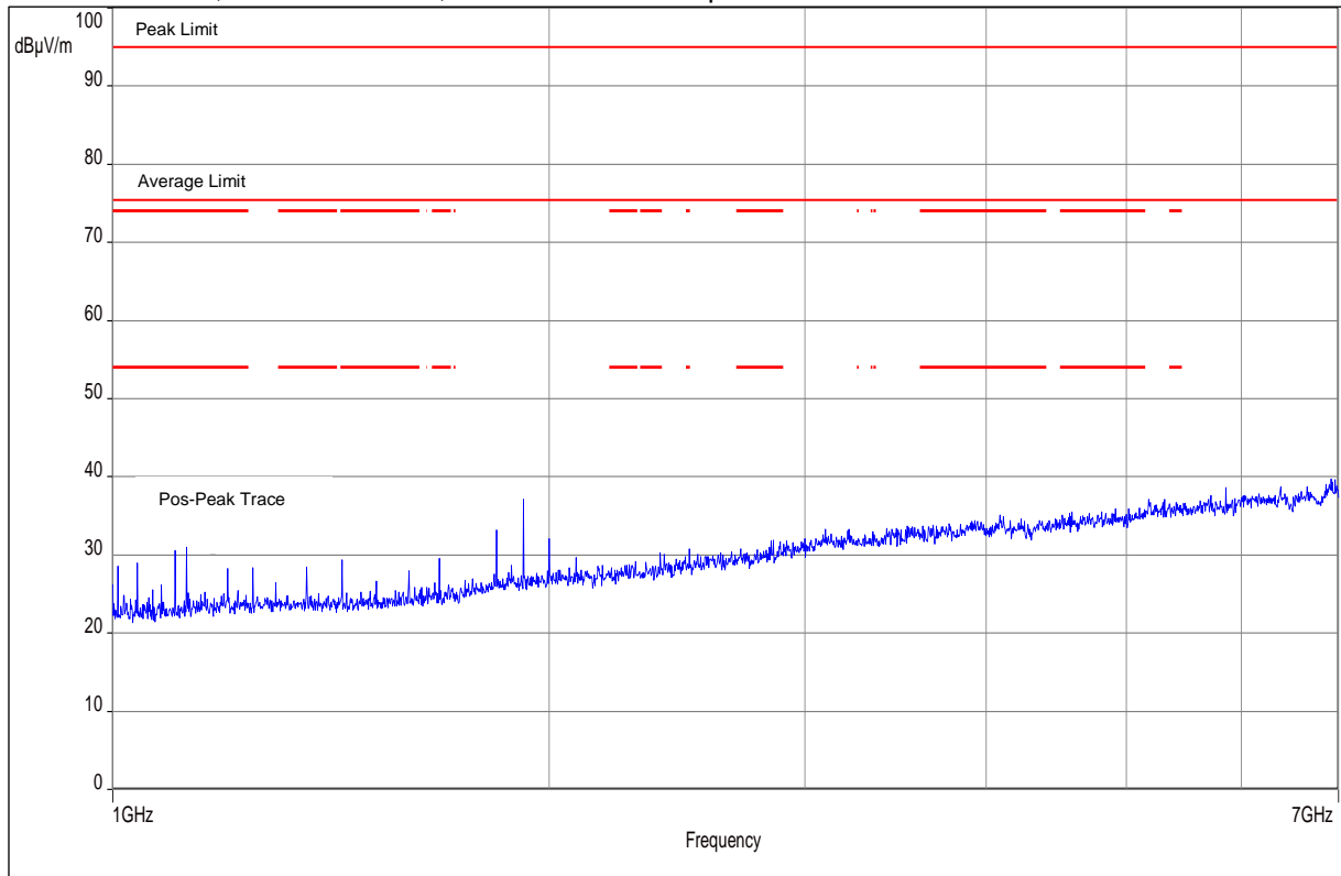
Plot No. 13: Low Ch., 1 GHz to 7 GHz, horizontal / vertical polarization
