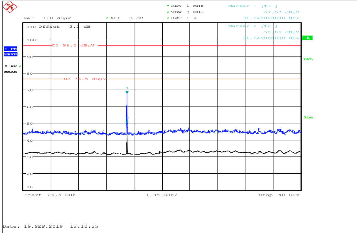
Plot No. 23: Valid for all Channels, 26.5 GHz to 40 GHz, horizontal / vertical polarization
