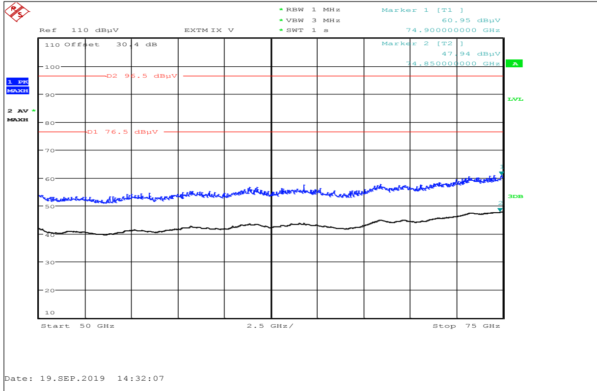
Plot No. 31: Valid for all Channels, 50 GHz to 75 GHz, horizontal / vertical polarization
