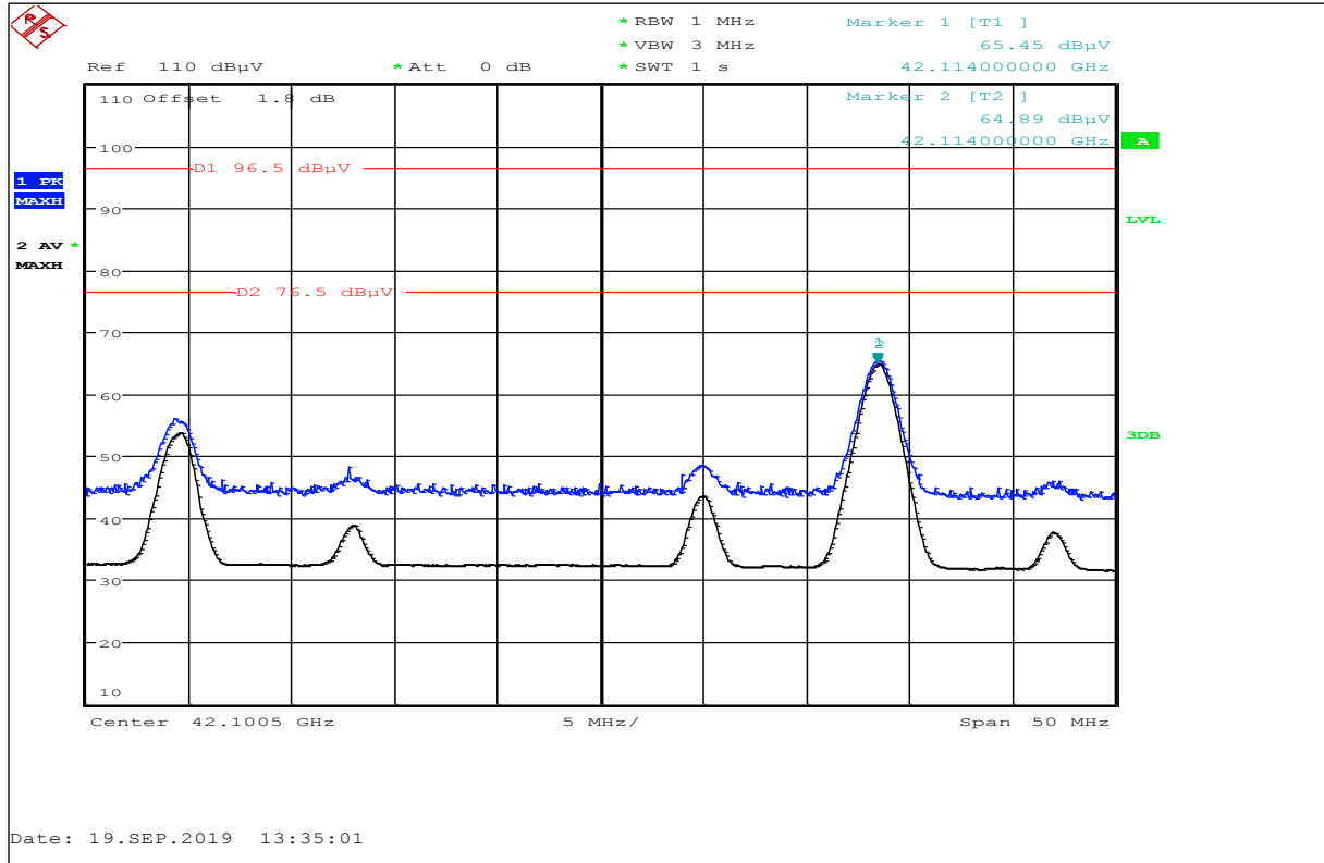
Plot No. 29: Middle Ch., Harmonic@42 GHz (restricted band above 38.6 GHz), horizontal / vertical polarization
