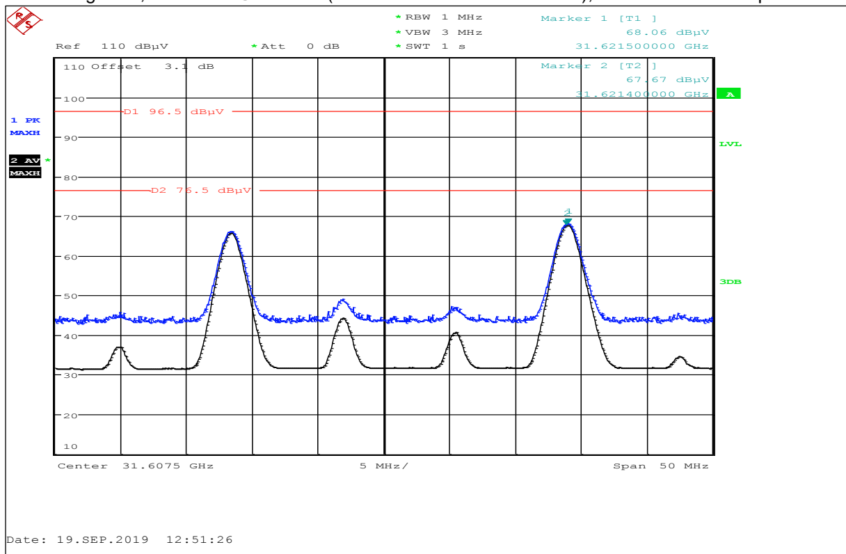
Plot No. 26: High Ch., Harmonic @ 31 GHz (restricted band 31.2-31.8 GHz), horizontal / vertical polarization
