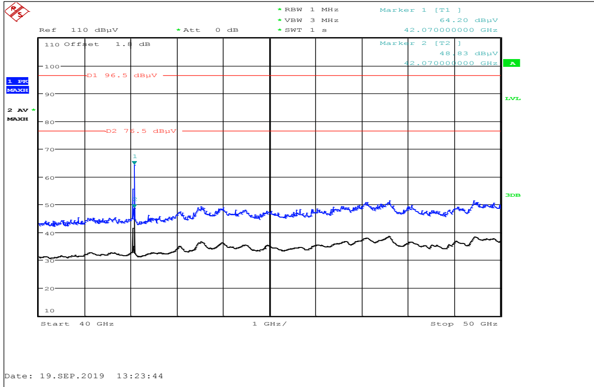
Plot No. 27: Valid for all Channels, 40 GHz to 50 GHz, horizontal / vertical polarization
