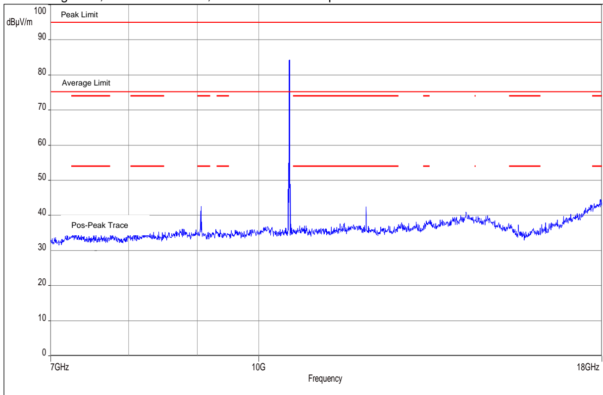
Plot shows the wanted signal at High Channel
