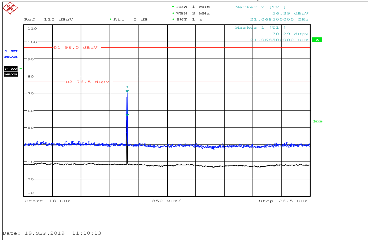
Plot No. 19: Valid for all Channels, 18 GHz to 26.5 GHz, horizontal / vertical polarization
