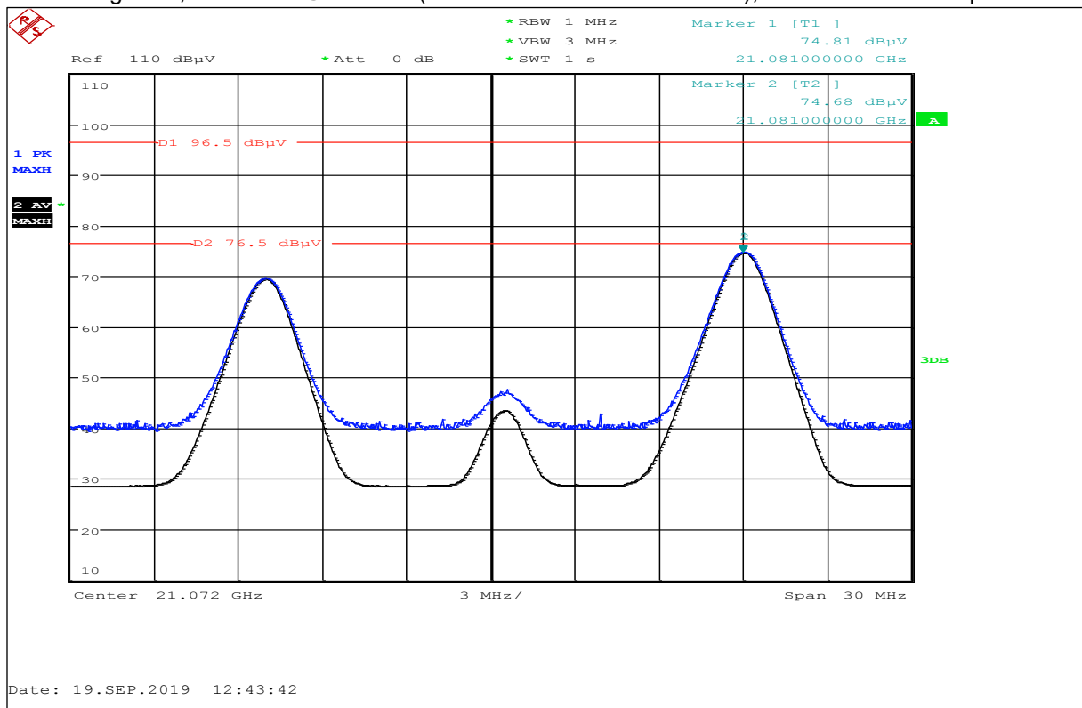
Plot No. 22: High Ch., Harmonic @ 21 GHz (restricted band 17.7-21.4 GHz), horizontal / vertical polarization
