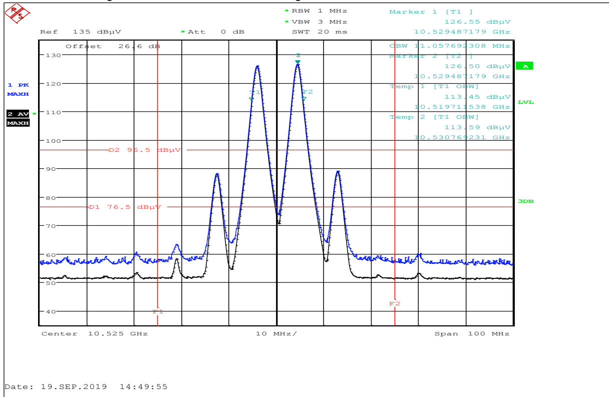
Plot No. 2: Field Strength Middle Ch., Peak and Average detector, T_{nom} / V_{nom}
