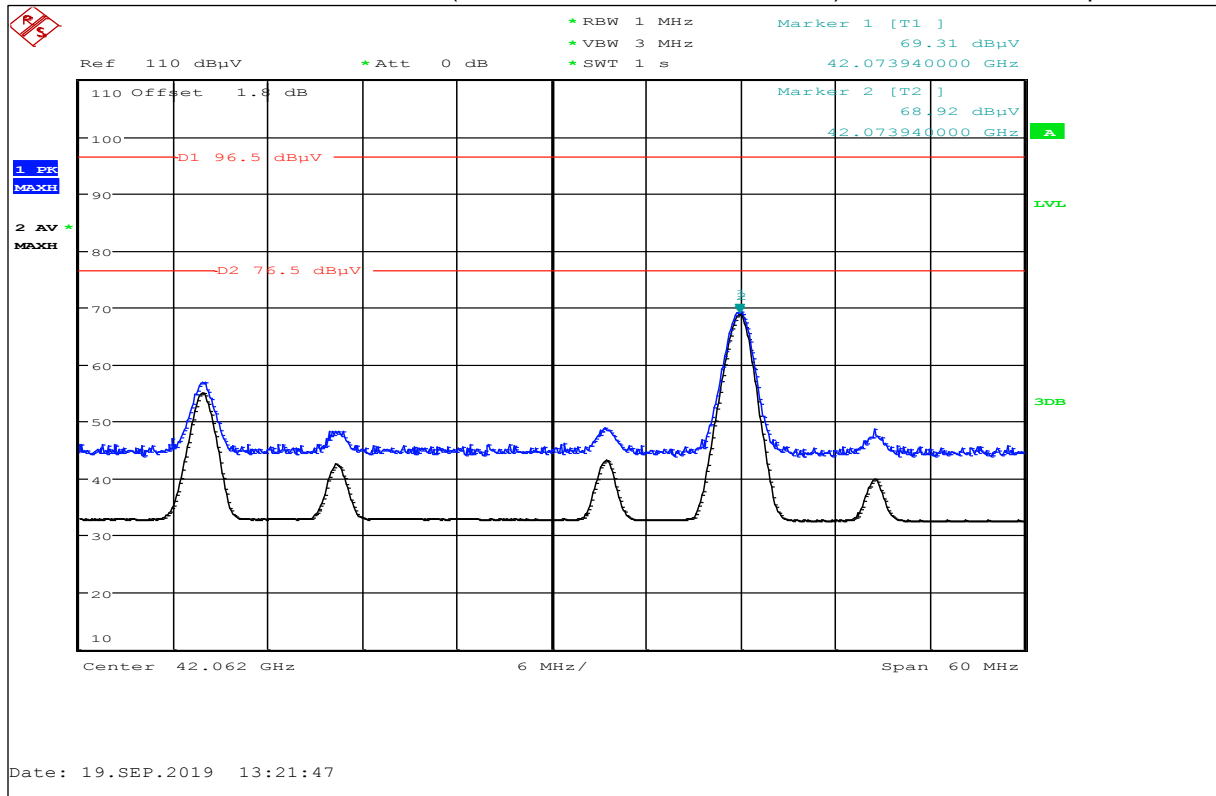
Plot No. 28: Low Ch., Harmonic@42 GHz (restricted band above 38.6 GHz), horizontal / vertical polarization
