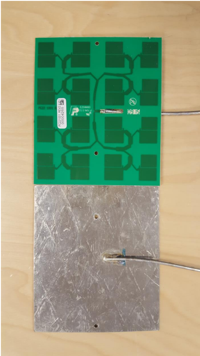
TX/RX antennas & RCM board with SMA-view
