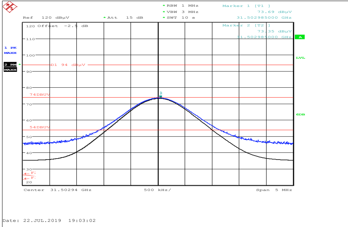
Plot No. 22: Low Ch., Harmonic @ 31 GHz (restricted band 31.2-31.8 GHz), horizontal / vertical polarization
