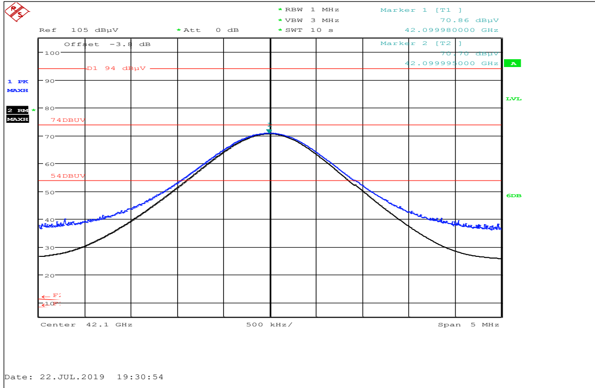
Plot No. 30: Middle Ch., Harmonic@42 GHz (restricted band above 38.6 GHz), horizontal / vertical polarization
