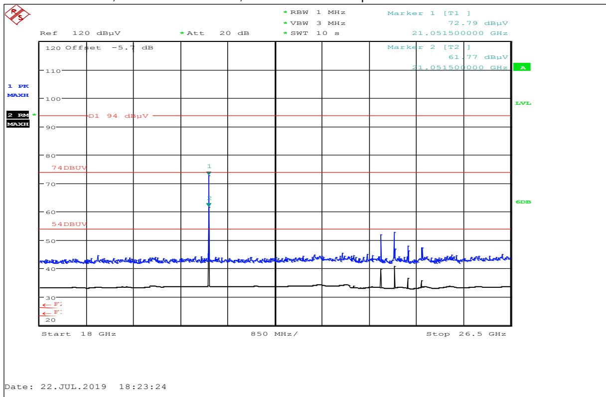
Plot No. 17: Middle Ch., 18 GHz to 26.5 GHz, horizontal / vertical polarization
