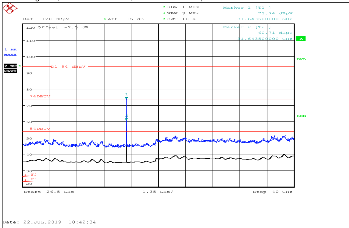
Plot No. 25: High Ch., 26.5 GHz to 40 GHz, horizontal / vertical polarization
