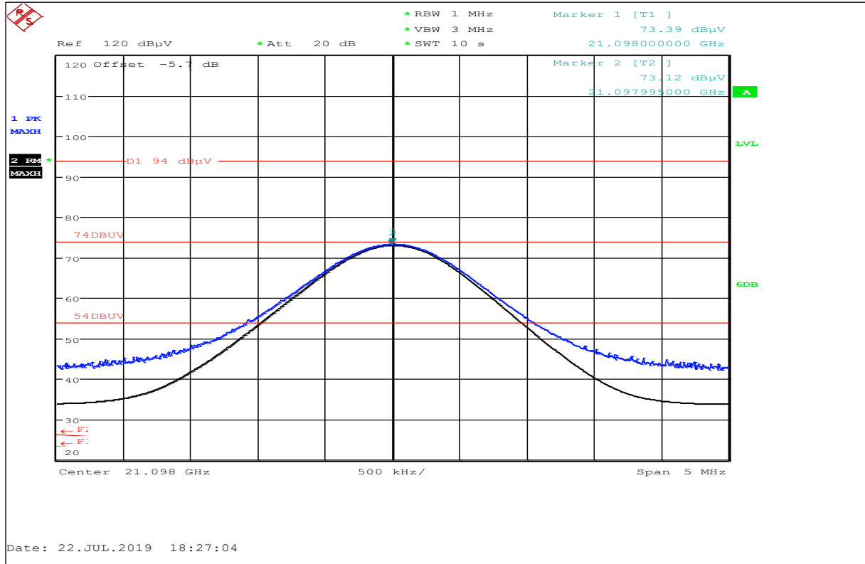
Plot No. 20: High Ch., Harmonic @ 21 GHz (restricted band 17.7-21.4 GHz), horizontal / vertical polarization
