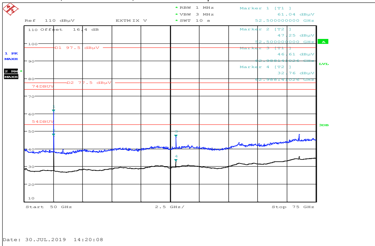
Plot No. 33: Low Ch., 50 GHz to 75 GHz, horizontal / vertical polarization
