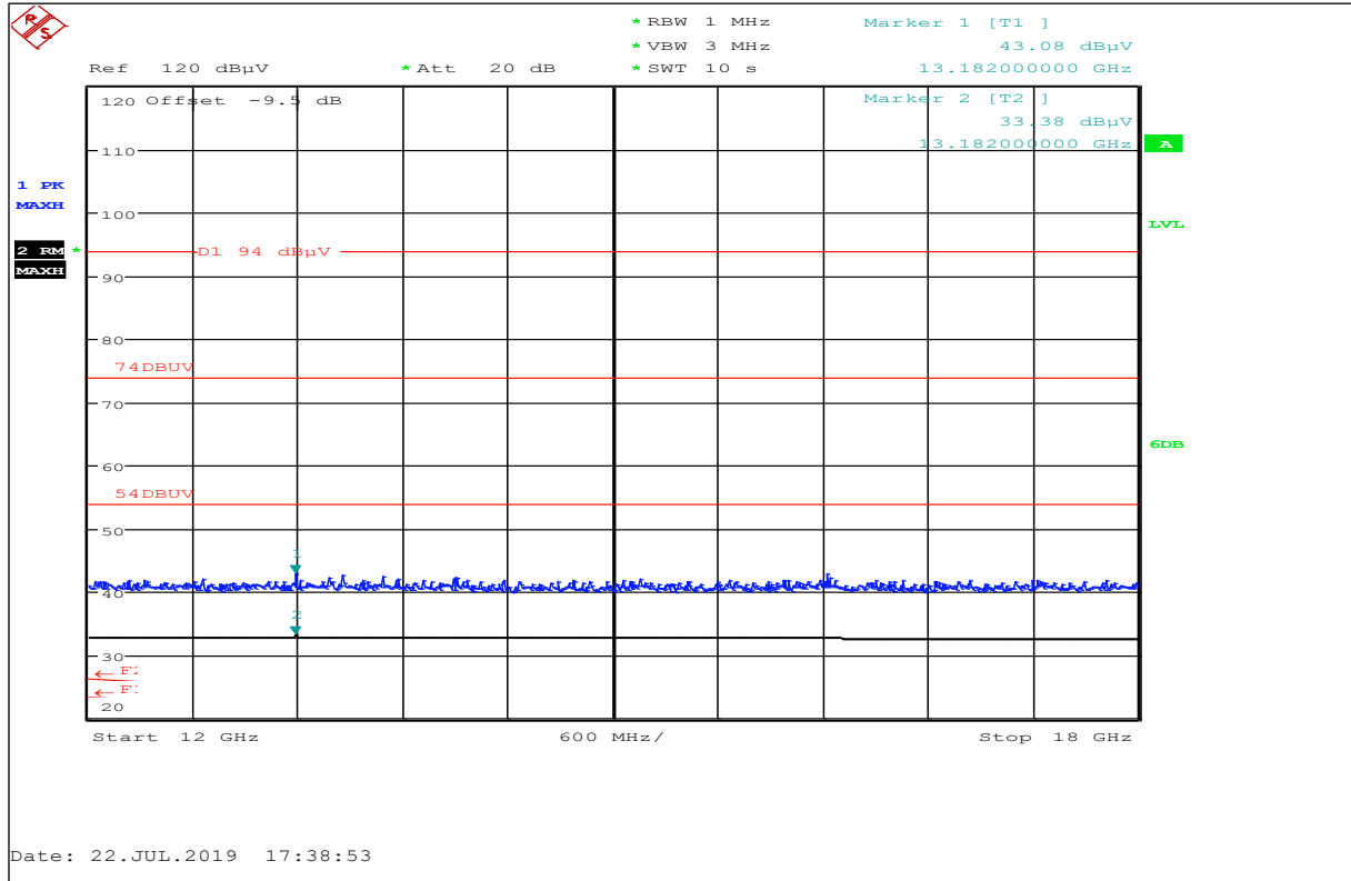
Plot No. 14: Valid for all Channels, 12 GHz to 18 GHz, horizontal / vertical polarization
