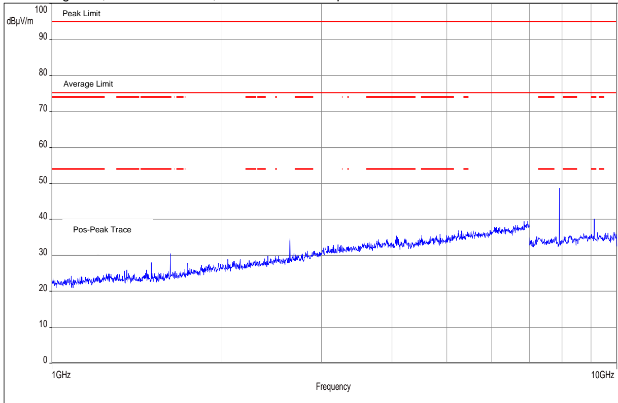
Plot No. 12: High Ch., 1 GHz to 10 GHz, horizontal / vertical polarization
