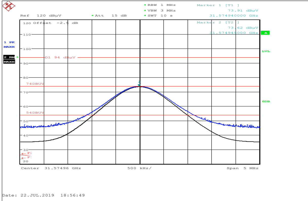
Plot No. 24: Middle Ch., Harmonic @ 31 GHz (restricted band 31.2-31.8 GHz), horizontal / vertical polarization
