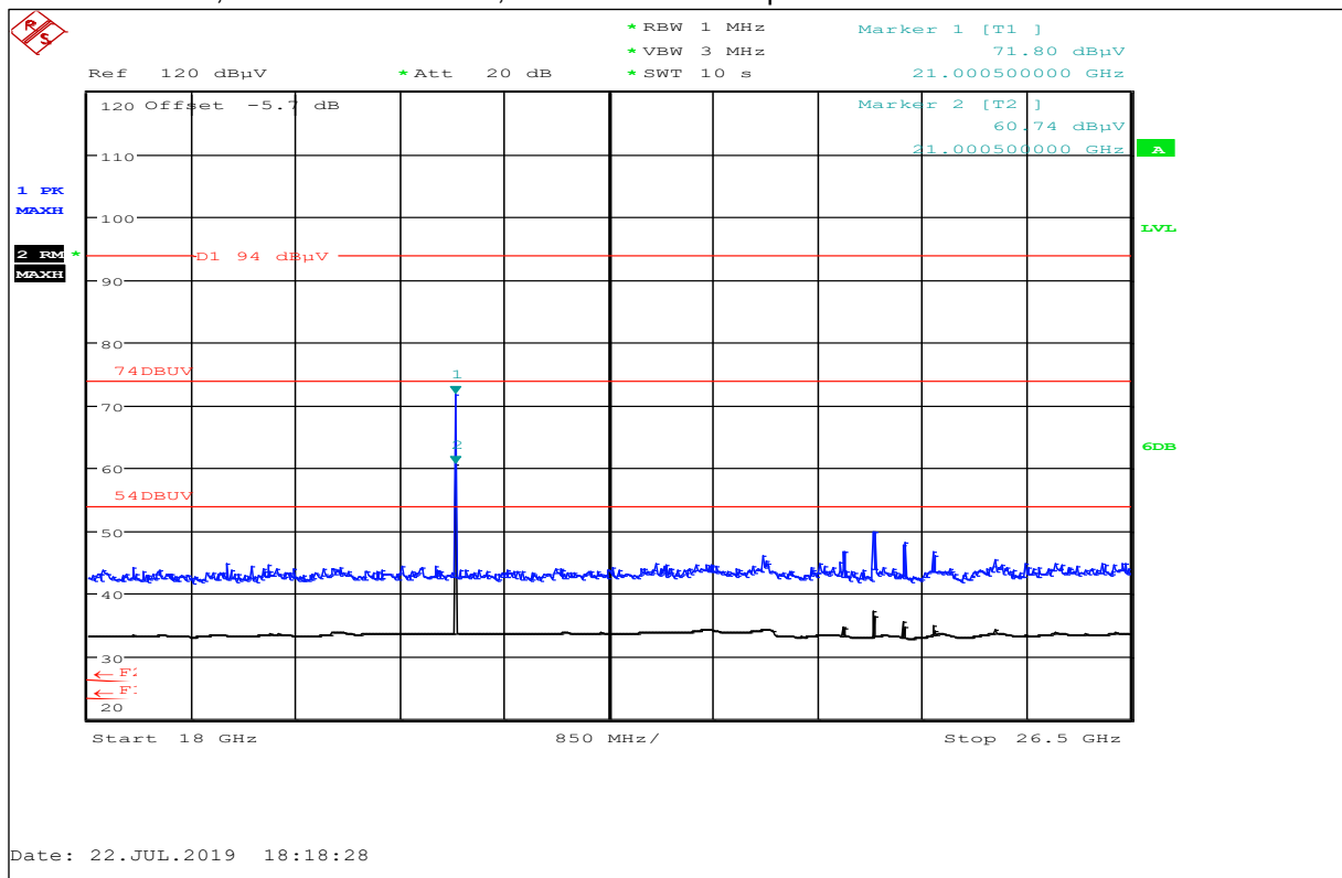
Plot No. 15: Low Ch., 18 GHz to 26.5 GHz, horizontal / vertical polarization
