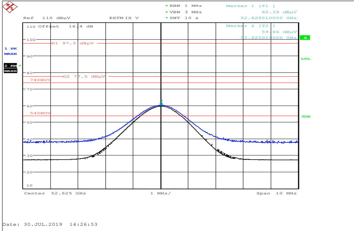
Plot No. 36: Middle Ch., Harmonic@52 GHz (restricted band above 38.6 GHz), horizontal / vertical polarization
