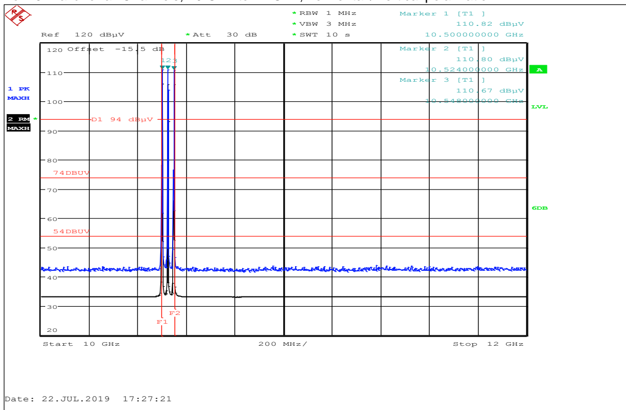
Plot No. 13: Valid for all Channels, 10 GHz to 12 GHz, horizontal / vertical polarization
