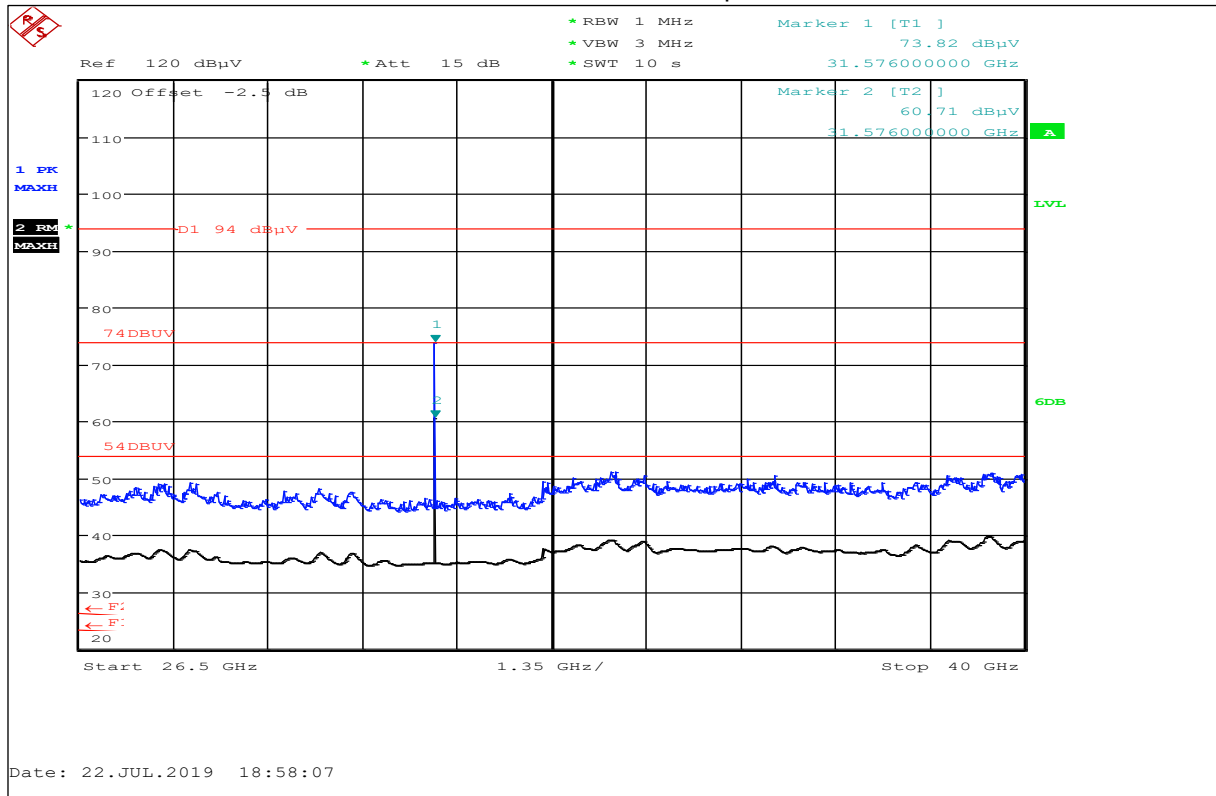
Plot No. 23: Middle Ch., 26.5 GHz to 40 GHz, horizontal / vertical polarization
