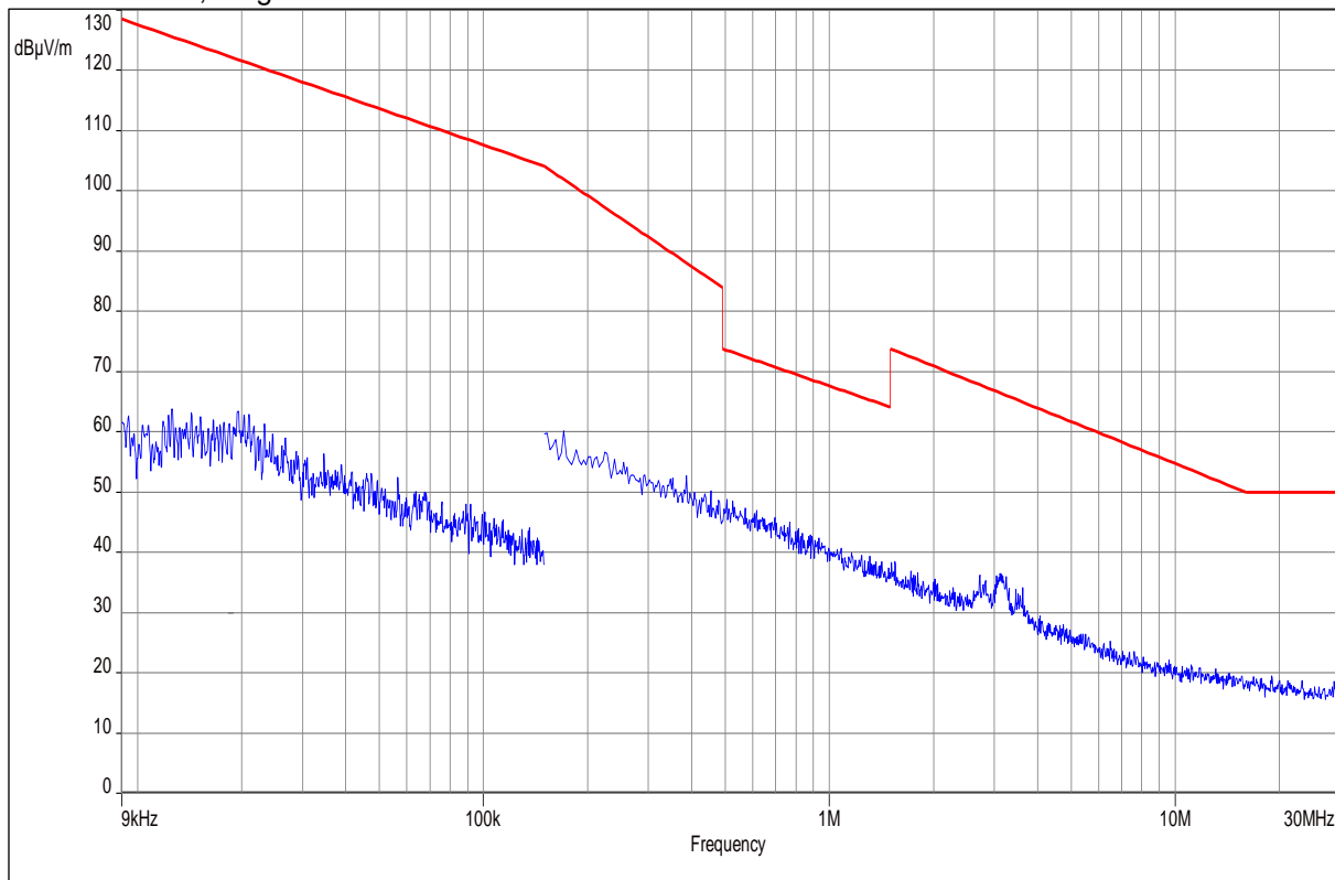
Plot No. 4: Low Ch., Magnetic: 9 kHz - 30 MHz
