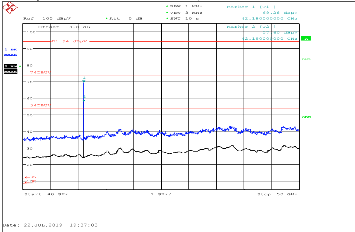
Plot No. 31: High Ch., 40 GHz to 50 GHz, horizontal / vertical polarization
