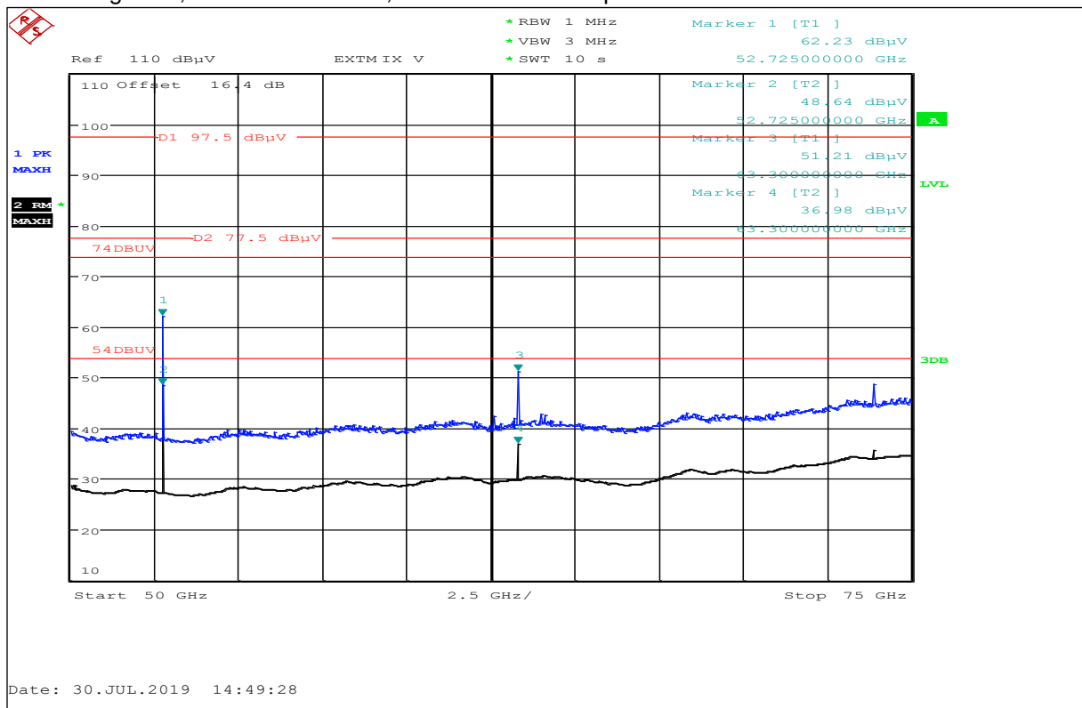
Plot No. 37: High Ch., 50 GHz to 75 GHz, horizontal / vertical polarization
