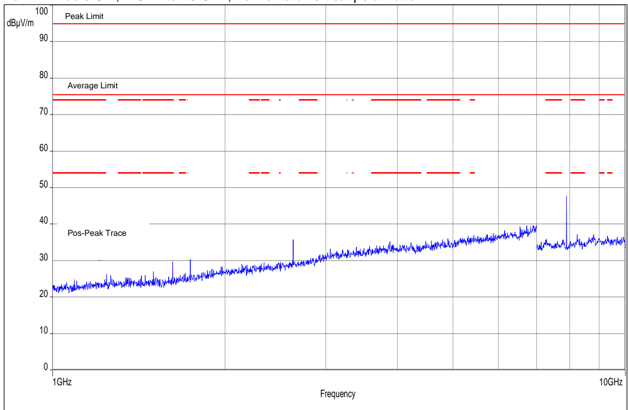
Plot No. 11: Middle Ch., 1 GHz to 10 GHz, horizontal / vertical polarization
