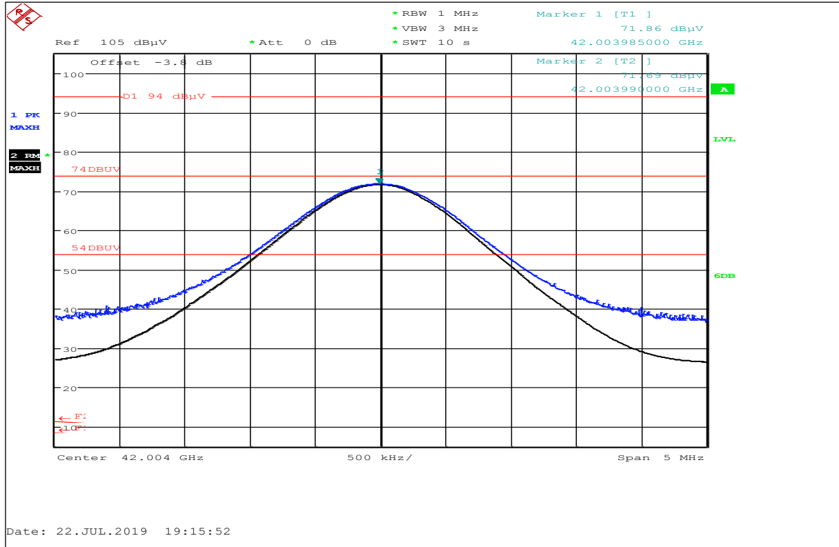
Plot No. 28: Low Ch., Harmonic@42 GHz (restricted band above 38.6 GHz), horizontal / vertical polarization
