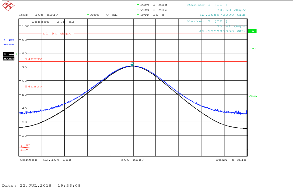
Plot No. 32: High Ch., Harmonic@42 GHz (restricted band above 38.6 GHz), horizontal / vertical polarization
