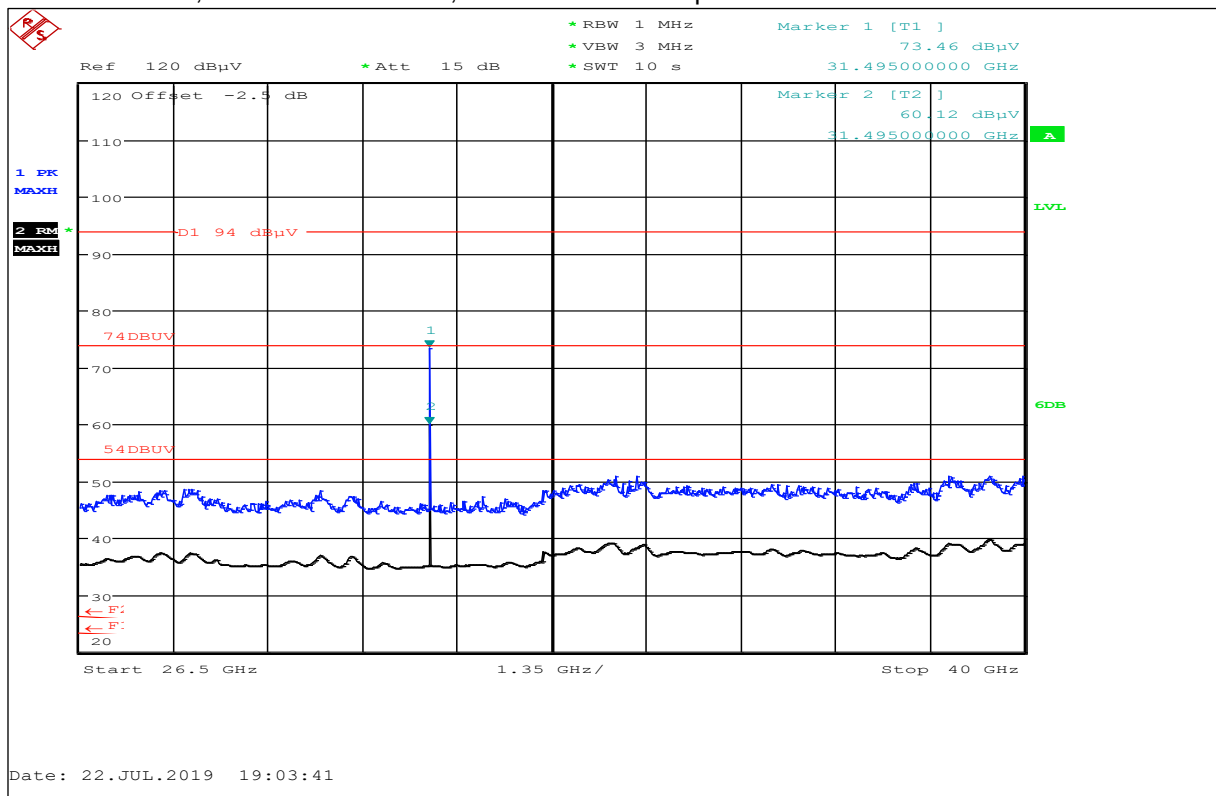
Plot No. 21: Low Ch., 26.5 GHz to 40 GHz, horizontal / vertical polarization
