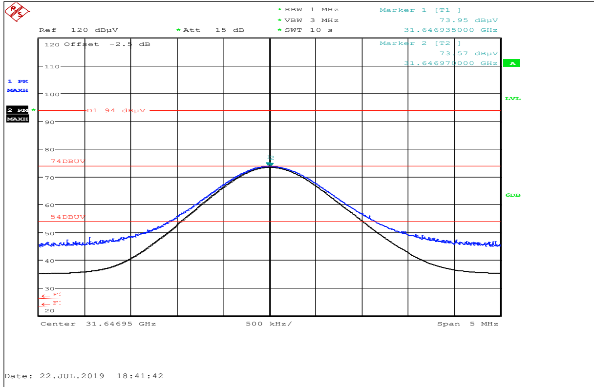
Plot No. 26: High Ch., Harmonic @ 31 GHz (restricted band 31.2-31.8 GHz), horizontal / vertical polarization
