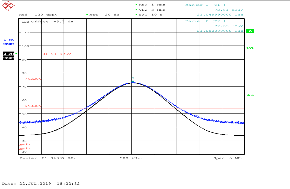
Plot No. 18: Middle Ch., Harmonic @ 21 GHz (restricted band 17.7-21.4 GHz), horizontal / vertical polarization
