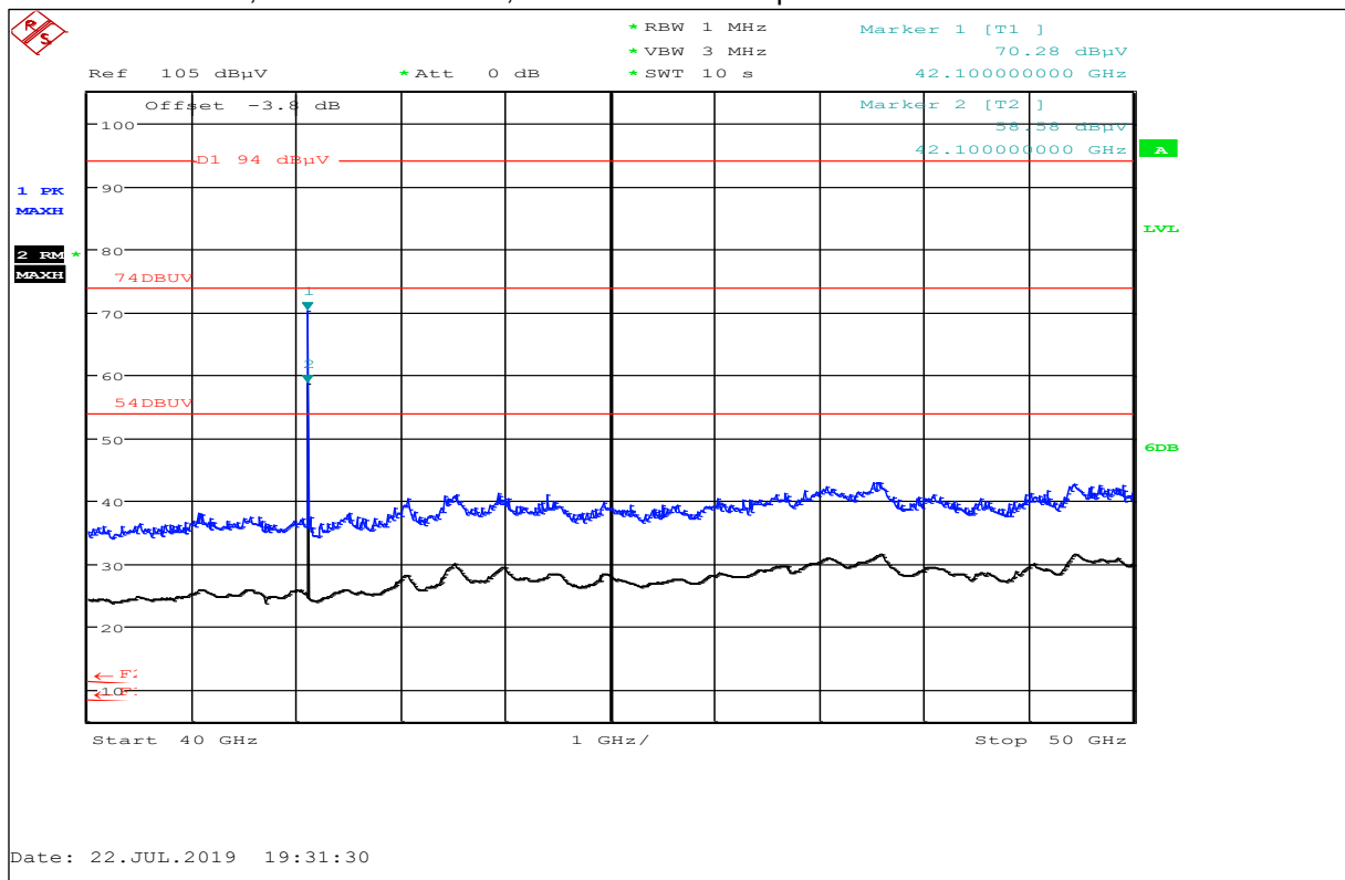
Plot No. 29: Middle Ch., 40 GHz to 50 GHz, horizontal / vertical polarization
