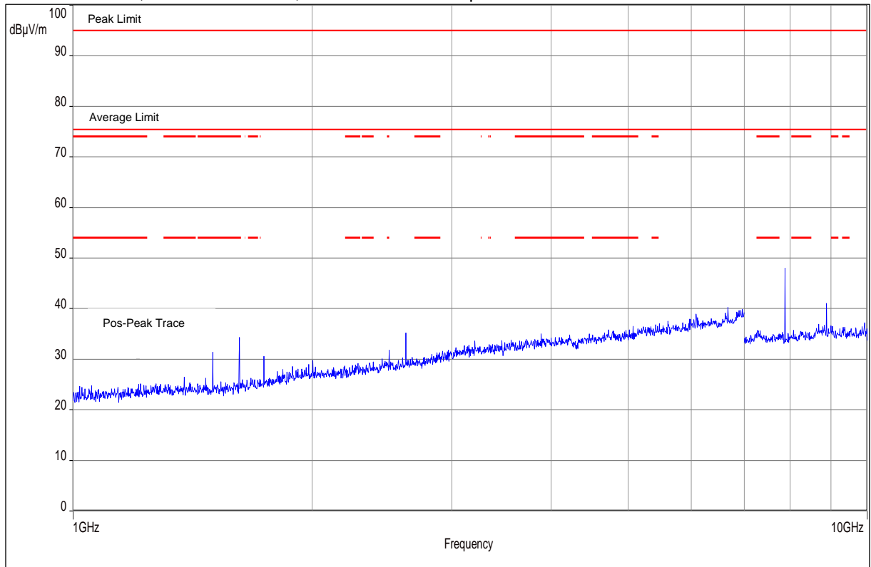
Plot No. 10: Low Ch., 1 GHz to 10 GHz, horizontal / vertical polarization
