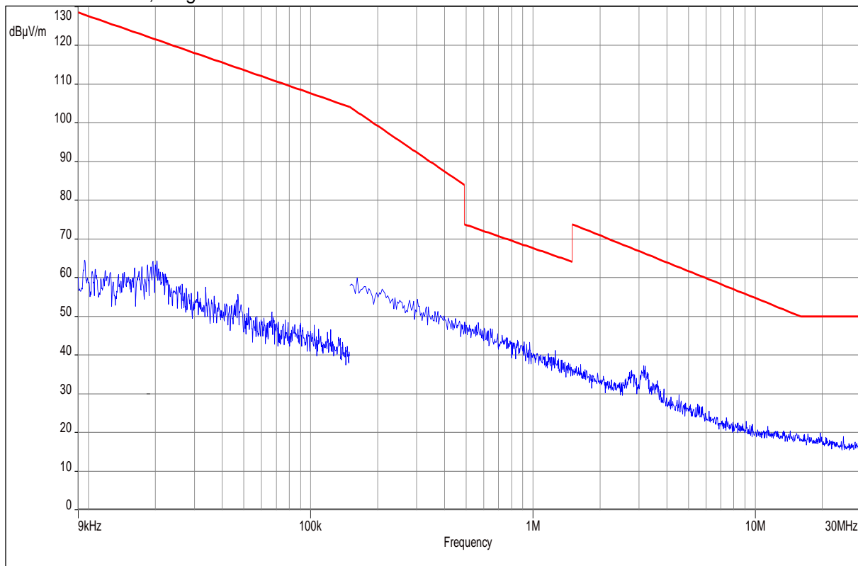
Plot No. 5: Middle Ch., Magnetic: 9 kHz - 30 MHz
