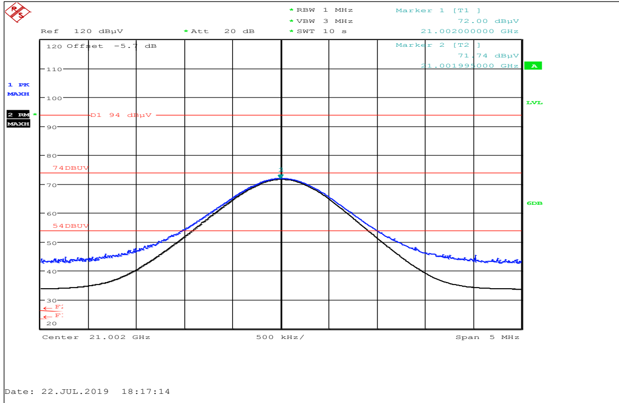
Plot No. 16: Low Ch., Harmonic @ 21 GHz (restricted band 17.7-21.4 GHz), horizontal / vertical polarization
