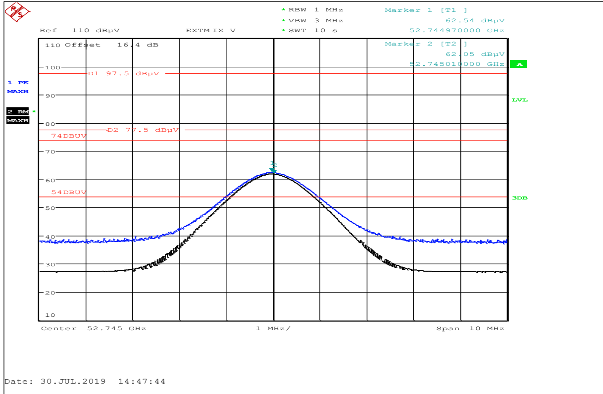
Plot No. 38: High Ch., Harmonic@52 GHz (restricted band above 38.6 GHz), horizontal / vertical polarization
