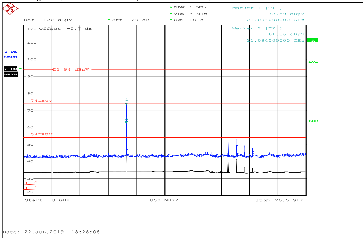
Plot No. 19: High Ch., 18 GHz to 26.5 GHz, horizontal / vertical polarization
