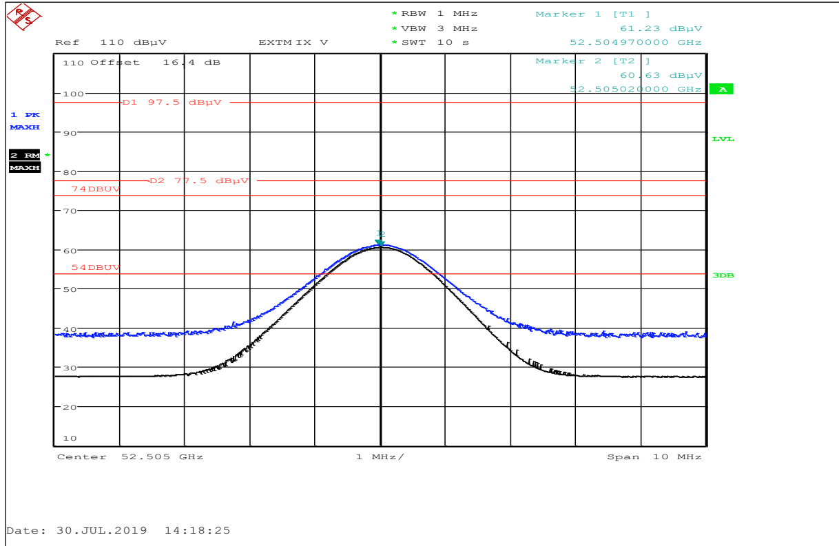
Plot No. 34: Low Ch., Harmonic@52 GHz (restricted band above 38.6 GHz), horizontal / vertical polarization
