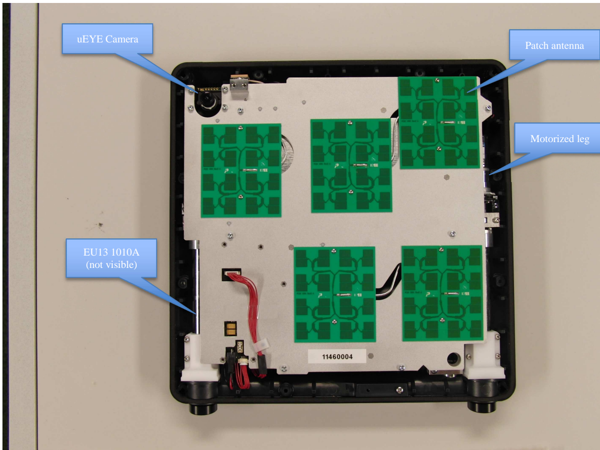
TMA3A, Antenna plate mounted in cabinet (front cover removed)
