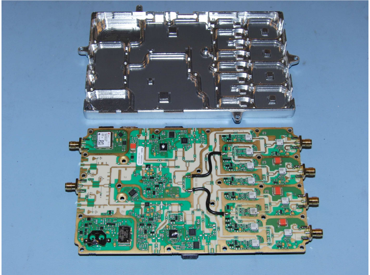
EU33 2001C seen from TOP side
