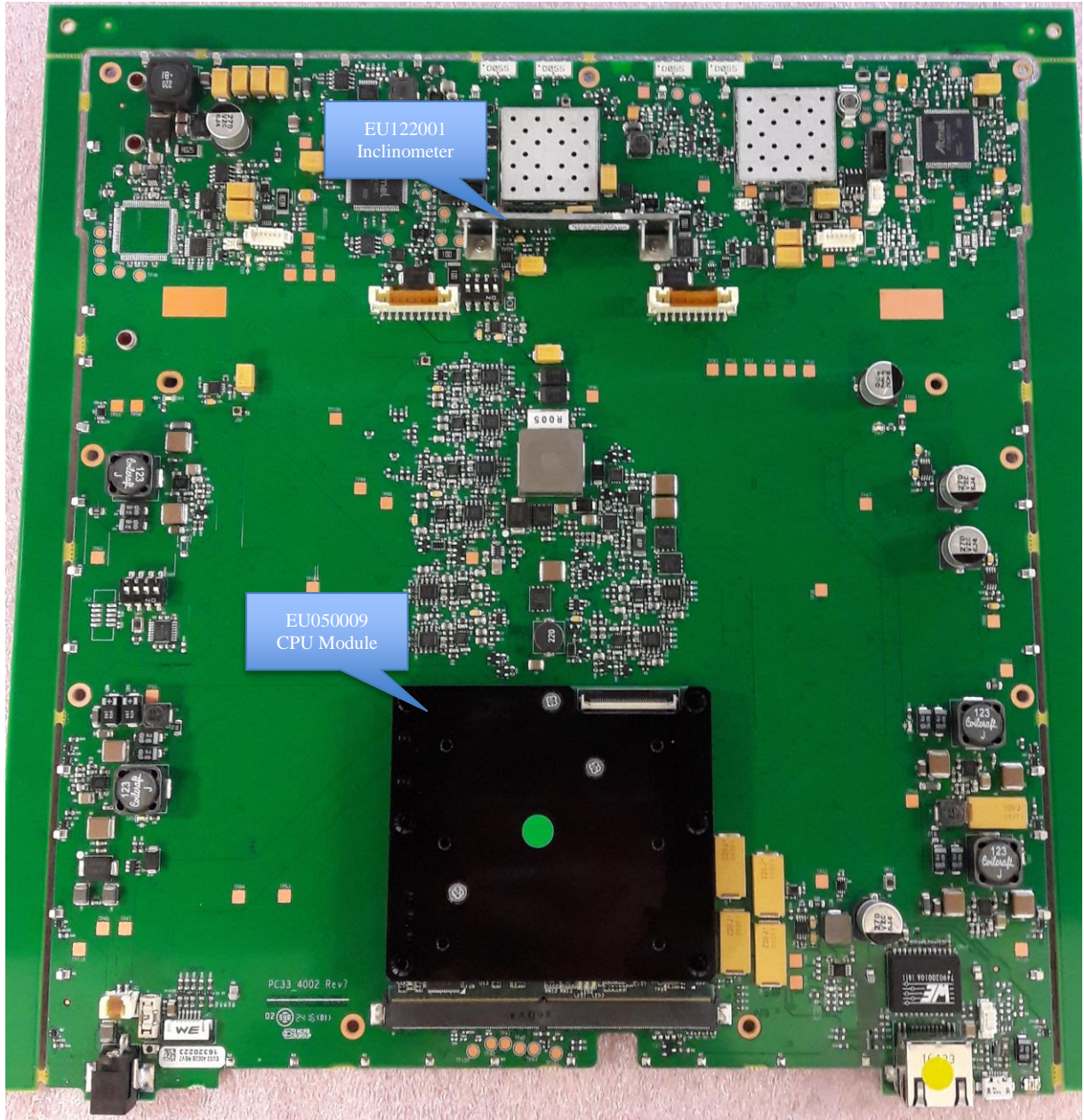
TMA4A PCB – EU334002 seen from back
