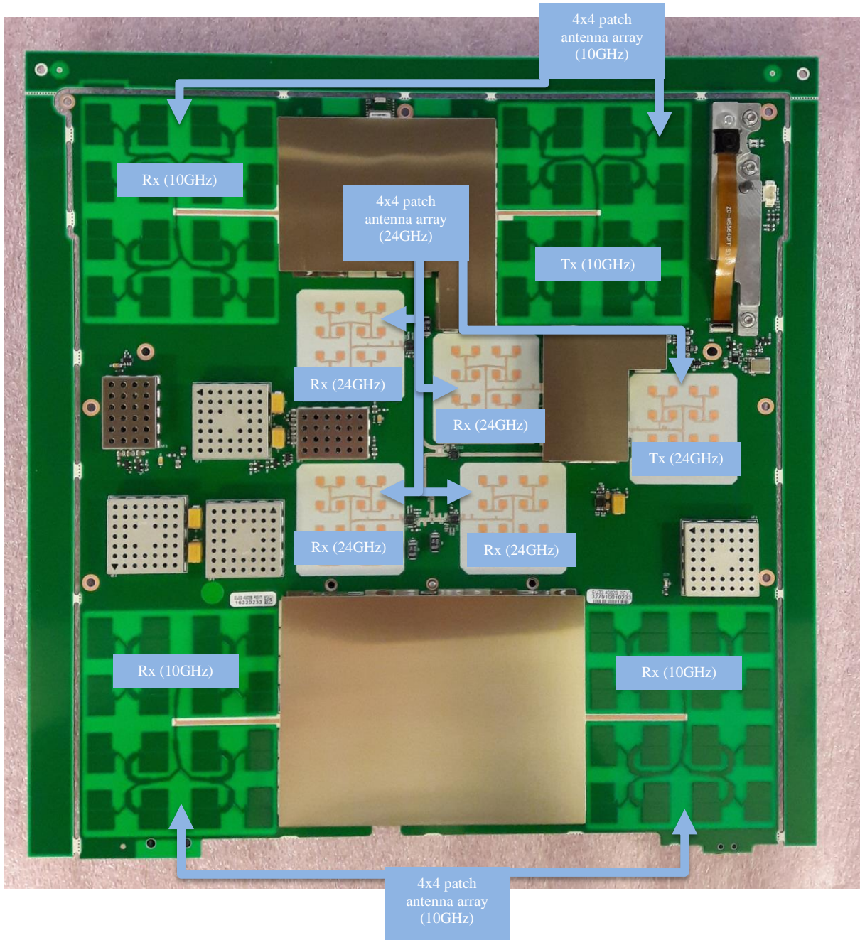
TMA4A PCB – EU334002 seen from front
