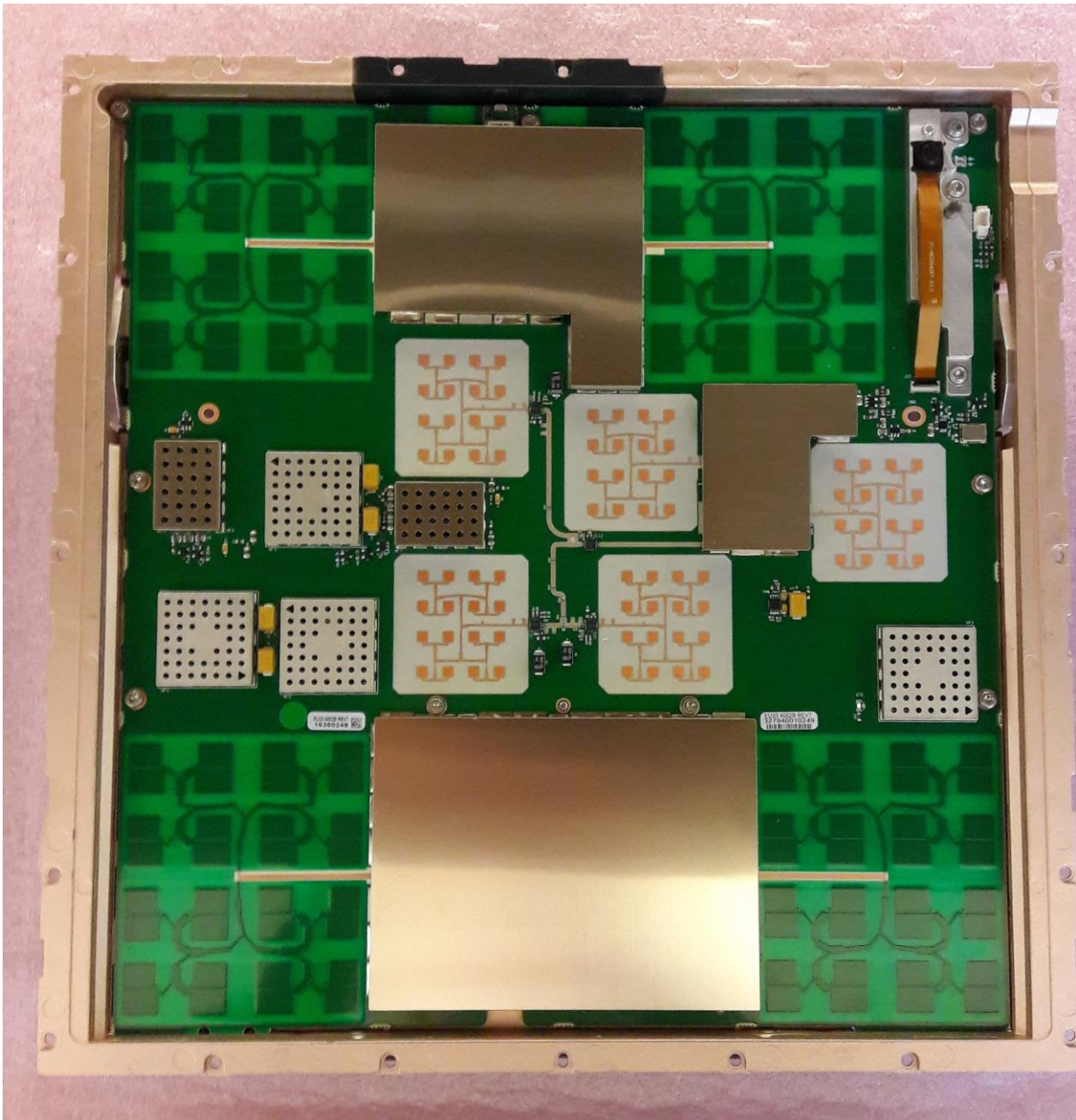
TMA4A PCB – EU334002 inside mechanical housing, seen from front
