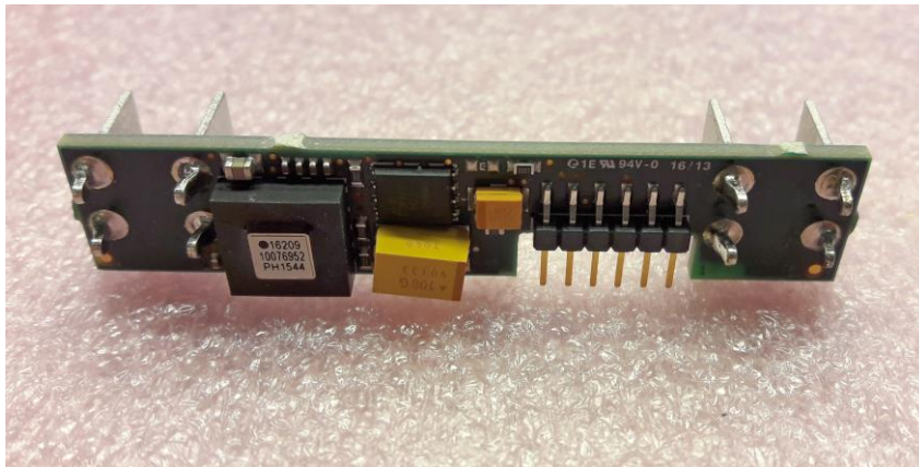
TMA4A Inclinometer module – EU122001, seen from back
