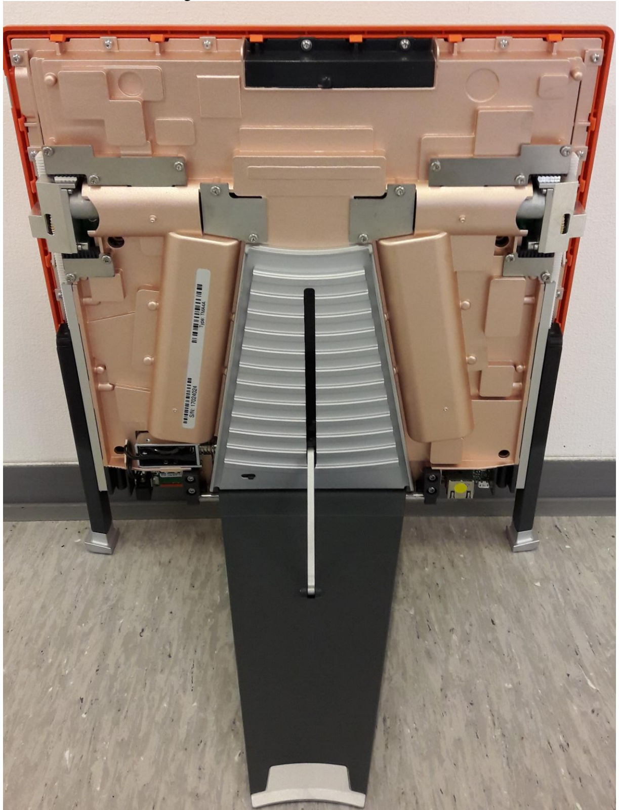
TMA4A mechanical housing with PCB – EU334002, seen from back
