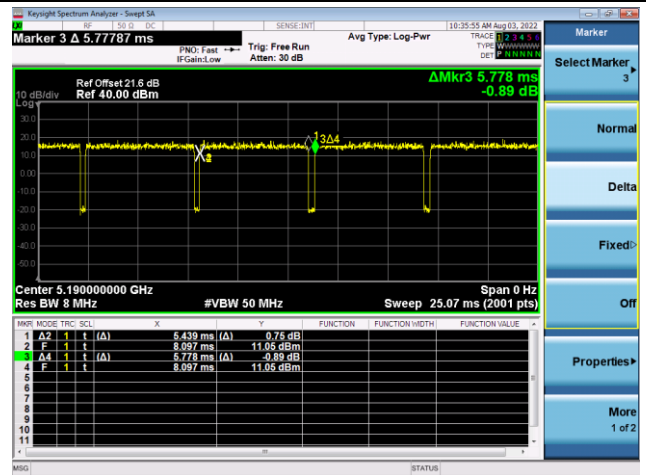
802.11ax-HE40 (T = 5.439ms)
