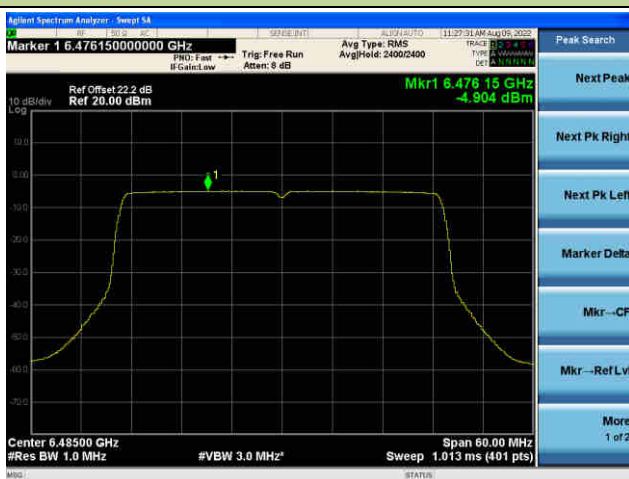
Channel 107 (6485MHz)
