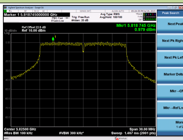
Channel 165 (5825MHz)
