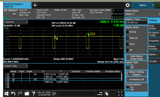
802.11ax-HE160 (T = 5.450ms)
