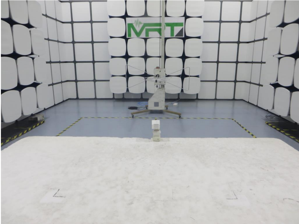
Description: Radiated Spurious Emission Test Setup for 1GHz ~ 18GHz (WF-402CB)
