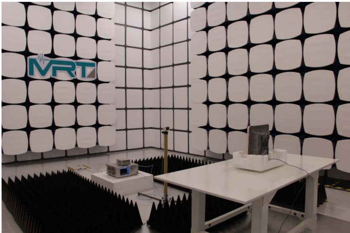
Description: Radiated Emission Test Setup for 18GHz ~ 40GHz
