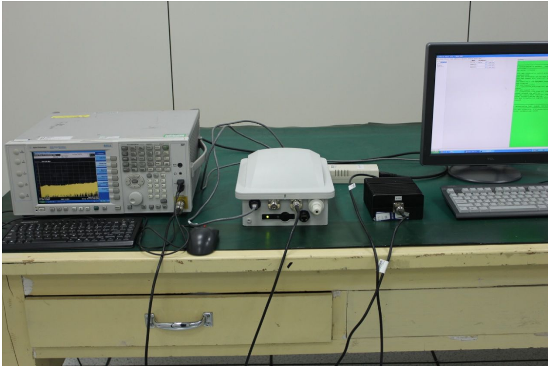
RF test
