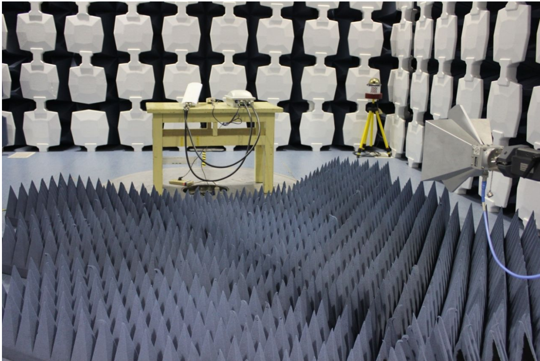
WF-3220-Z1 radiated emission high frequency
