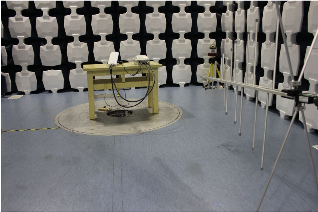
WF-3220-Z1 radiated emission low frequency
