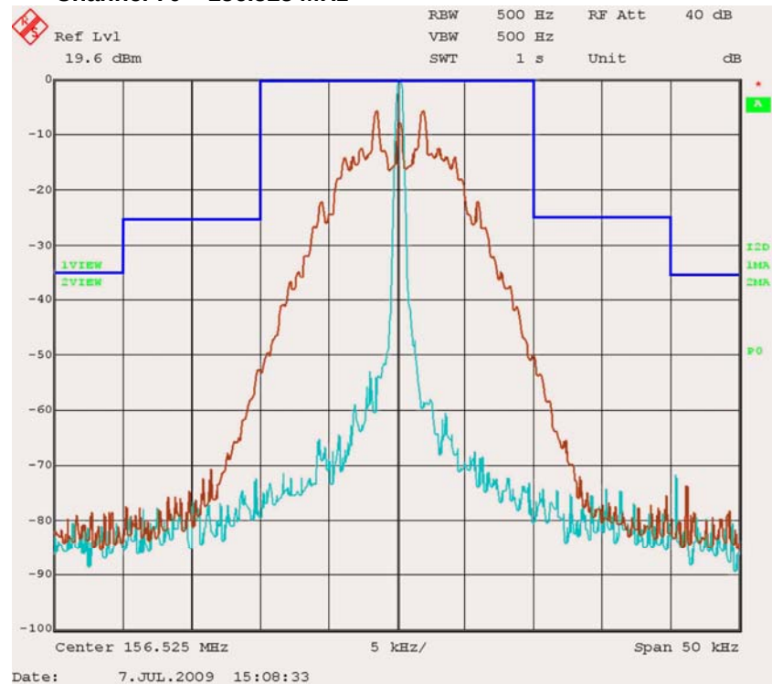
Channel 70 – 156.525 MHz
