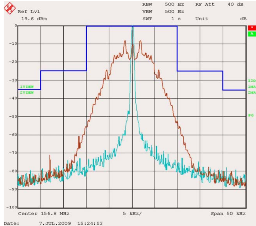
Channel 16 – 156.8 MHz
