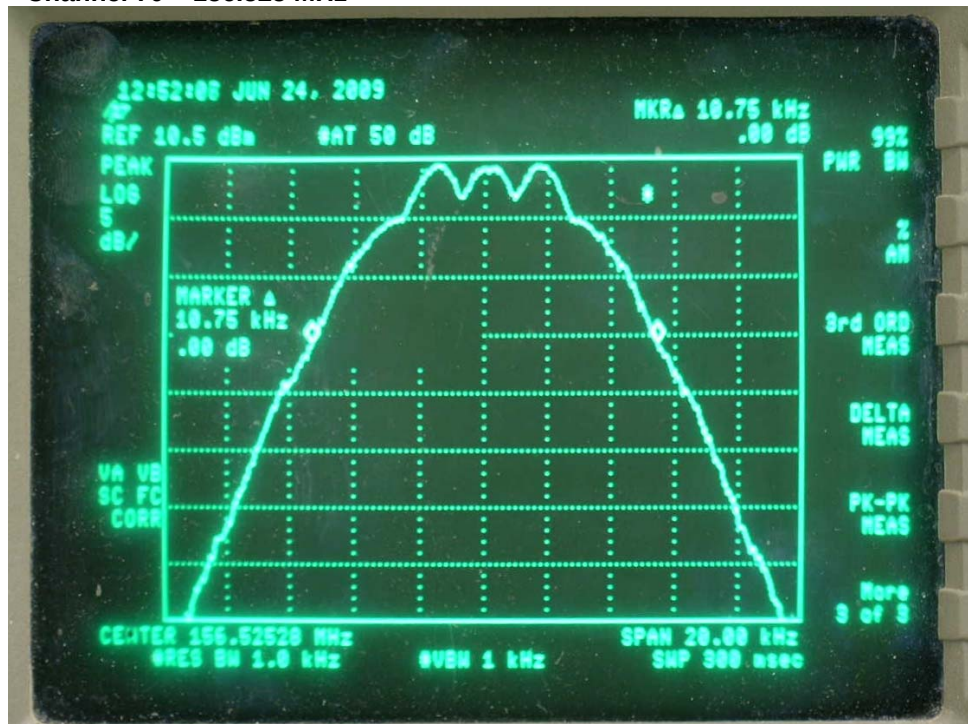
Channel 70 – 156.525 MHz
