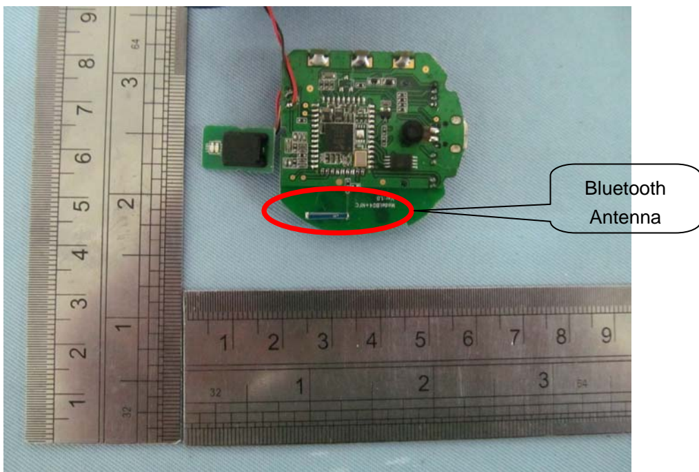
FRONT VIEW OF PCB-1
