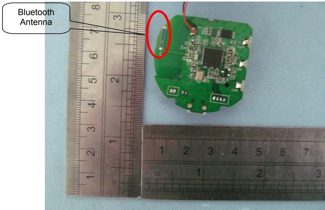
FRONT VIEW OF PCB-1
