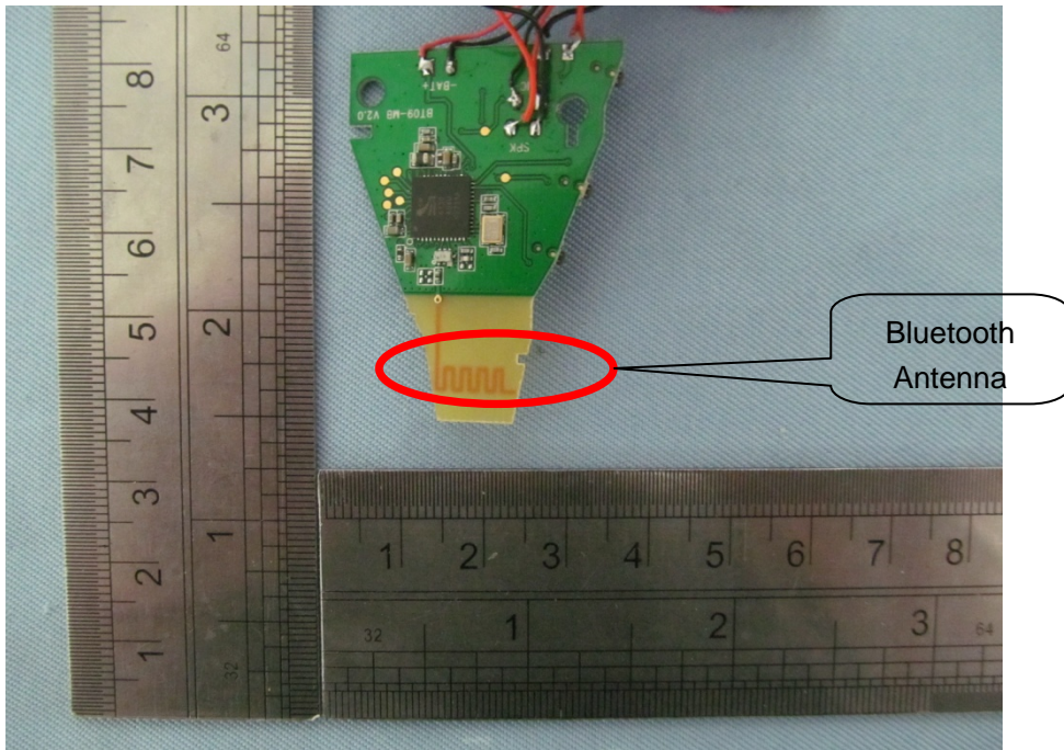
FRONT VIEW OF PCB-1
