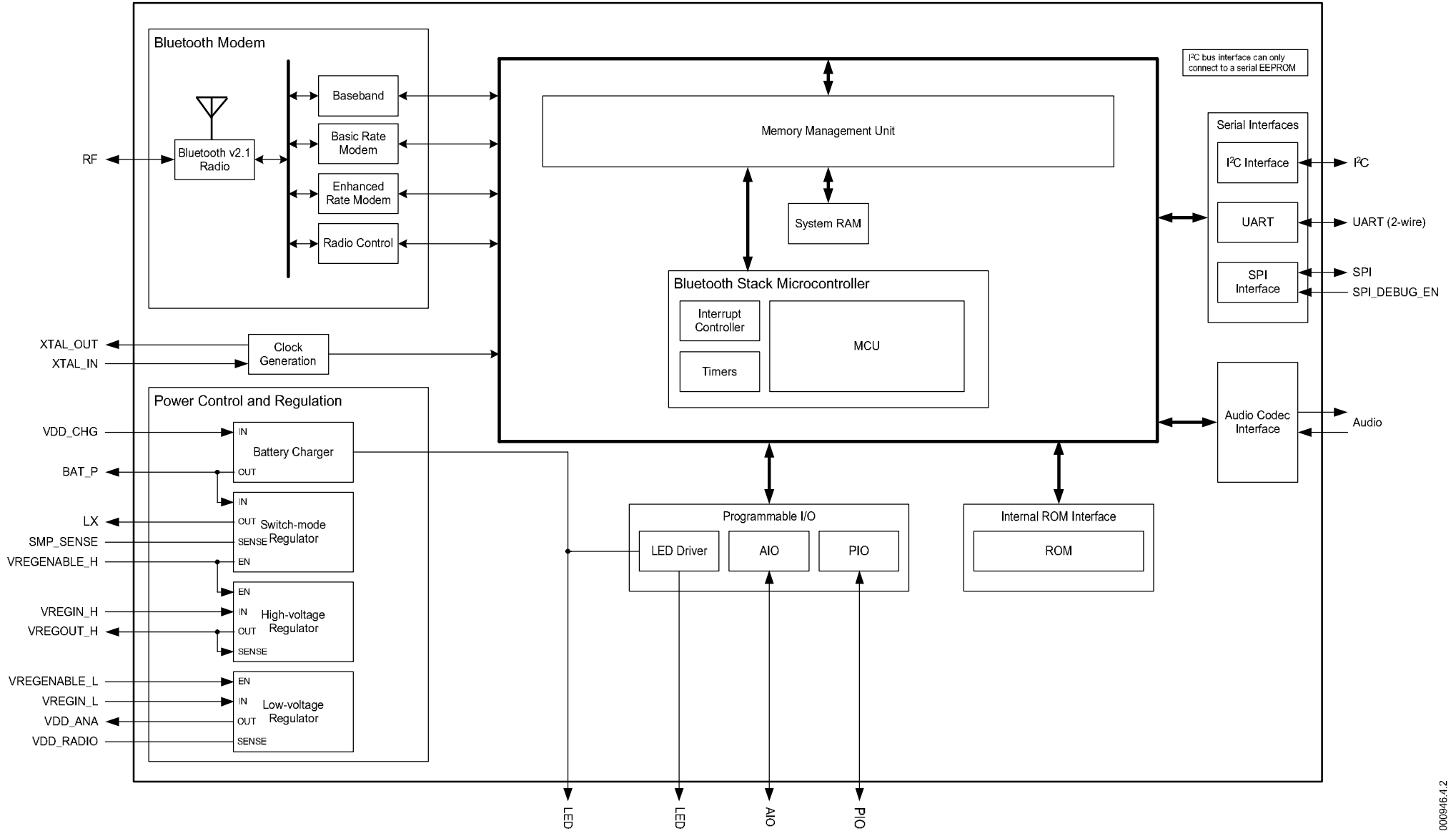
Figure 2.1: Functional Block Diagram
