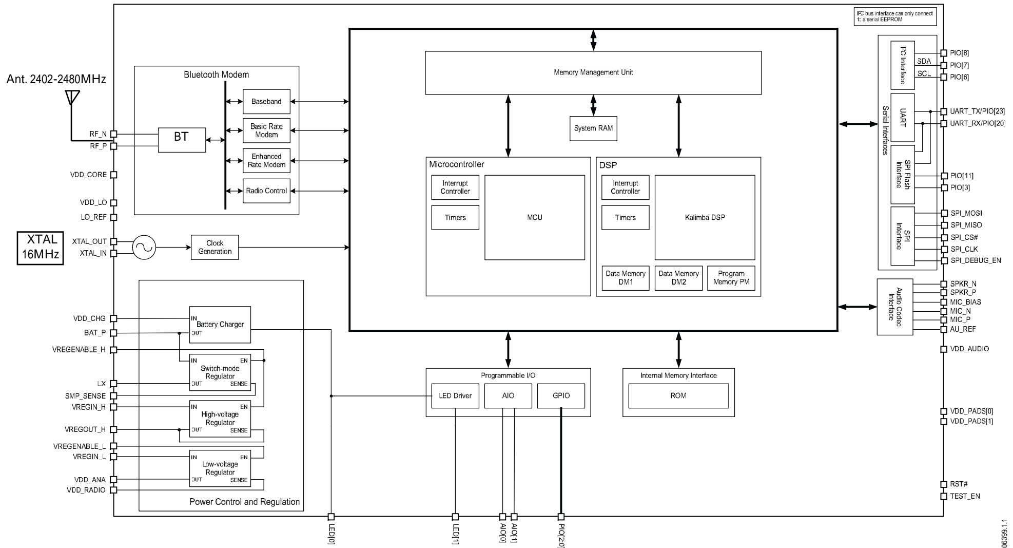
Figure : Functional Block Diagram
