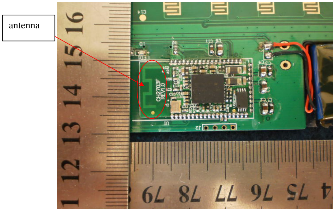
Appearance photograph of RF Board
