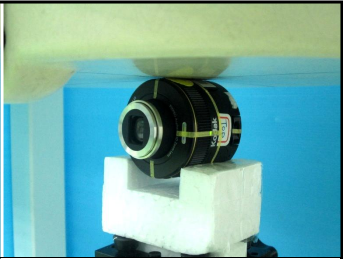
Ant Side of EUT with 0 cm Gap
